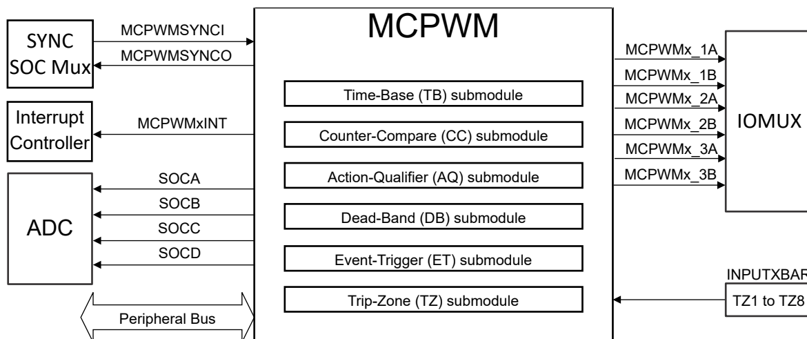
Figure 26-1. Submodules and Signal Connections for an MCPWM Module
