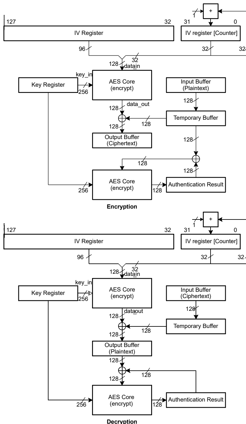
Figure 8-10. CCM Operation
