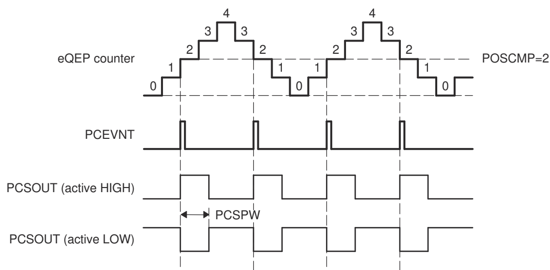
Figure 25-15. eQEP Position-compare Event Generation Points
