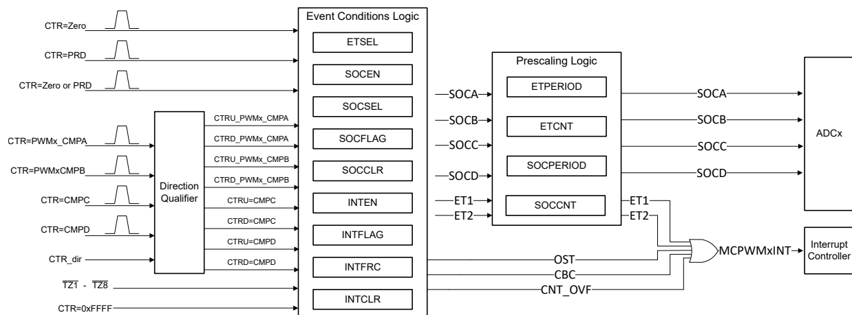
Figure 26-35. Event-Trigger Submodule Showing Event Inputs and Prescaled Outputs
