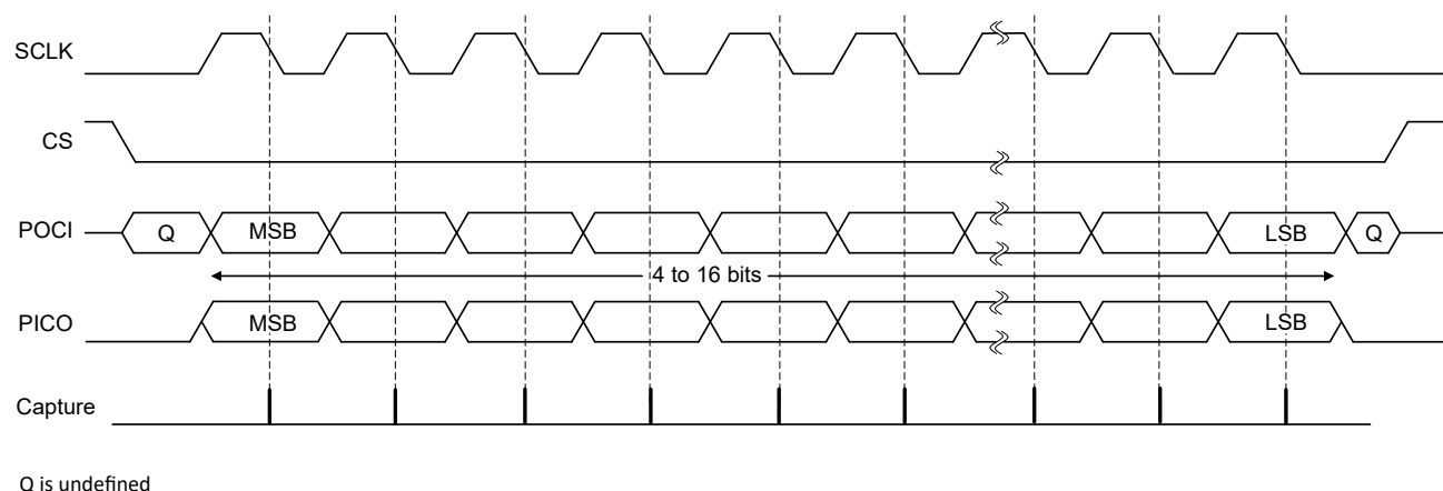
Figure 31-4. Motorola SPI Frame Format With SPO = 0 and SPH = 1
