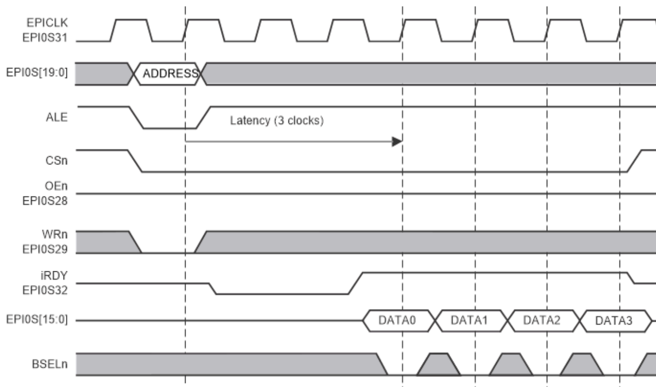
Figure 16-8. PSRAM Burst Write
