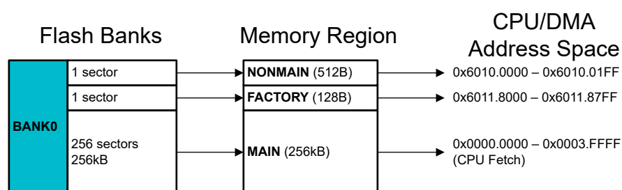
Figure 13-2. Memory Organization Example - Single Bank Configuration
