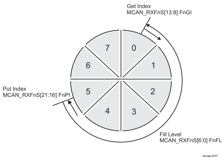
Figure 27-18. Rx FIFO Status
