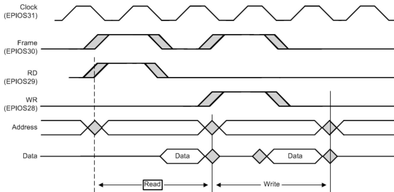
Figure 16-20. Two-Cycle Read, Write Accesses, FRM50 = 0, FRMCNT = 0, WR2CYC = 1
