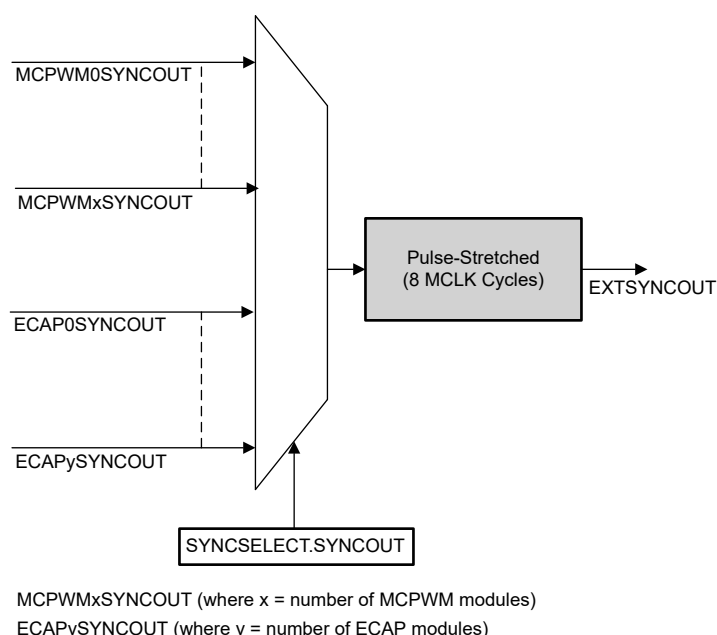
Figure 26-7. MCPWM External SYNC Output
