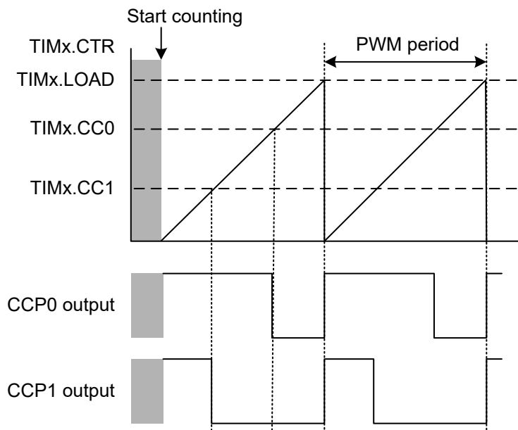
Figure 18-20. Edge-Aligned PWM Signals in Up-Counting Mode
