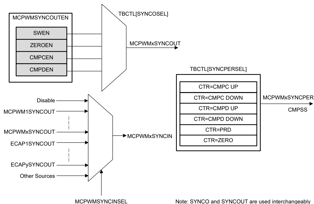
Figure 26-6. Time-Base Counter Synchronization Scheme
