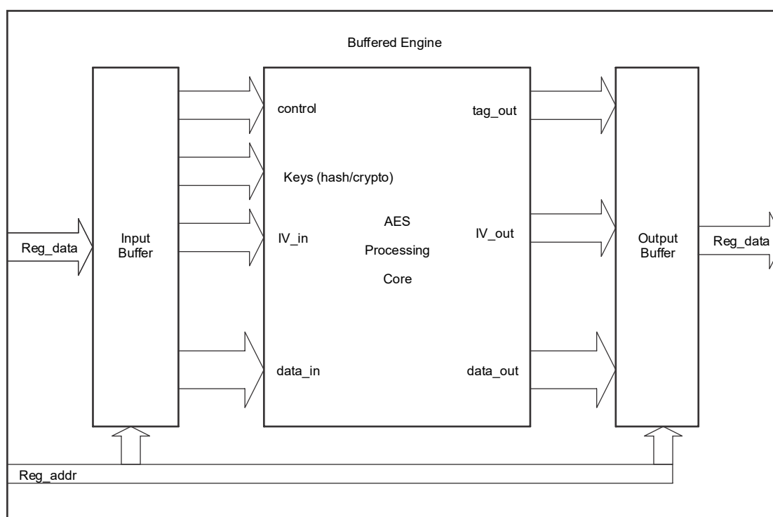
Figure 8-1. AES Block Diagram
