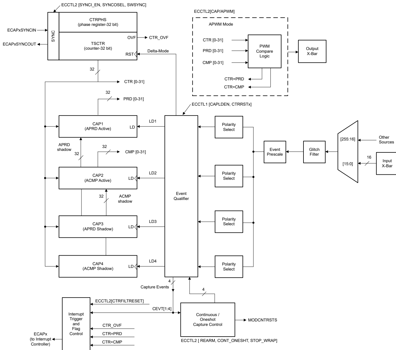
Figure 24-3. eCAP Block Diagram
