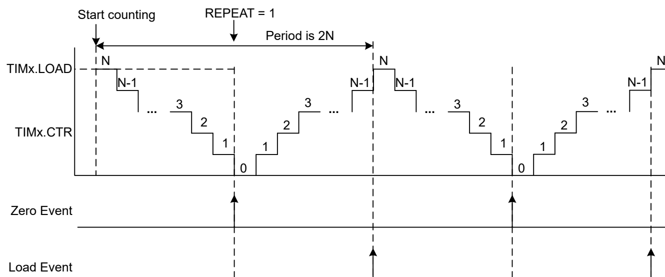
Figure 18-5. Down-up Counting Mode and Event Generation, CVAE = 0
