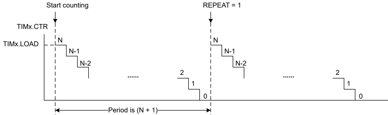
Figure 18-3. Down Counting Mode, CVAE = 0
