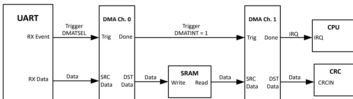
Figure 11-2. DMA Cascading Channels
