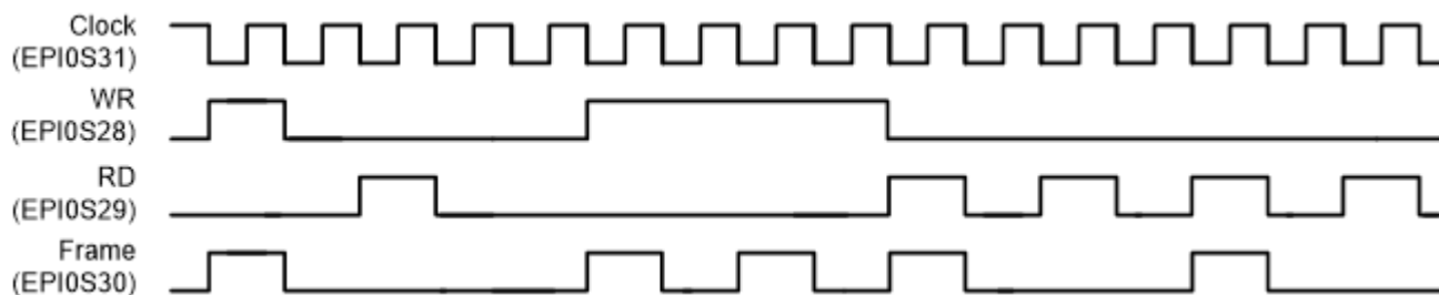
Figure 16-23. FRAME Signal Operation, FRM50 = 0 and FRMCNT = 1
