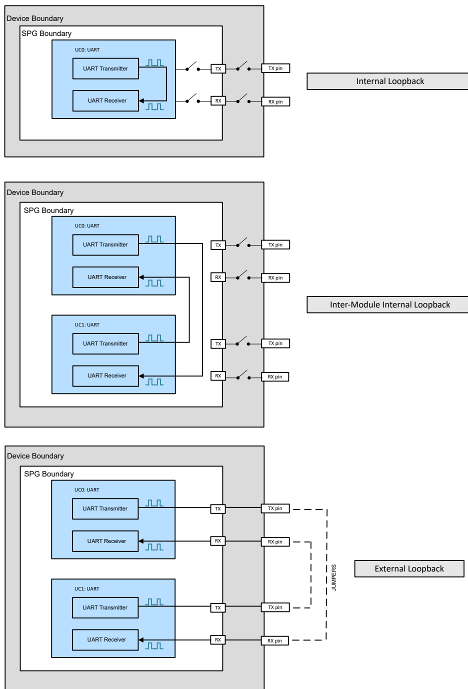
Figure 28-2. UNICOMM Loopback Types
