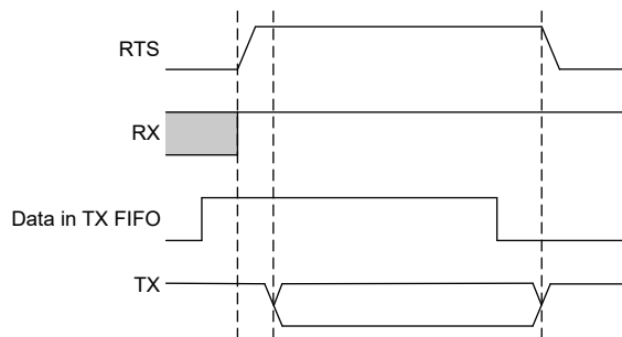
Figure 29-11. RS485 Data Exchange
