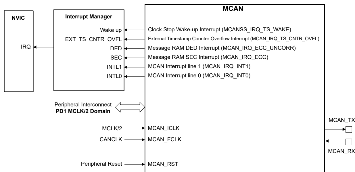
Figure 27-26. MCAN Integration
