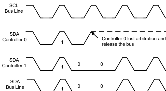
Figure 30-9. Arbitration Procedure Between Two Controller Transmitters
