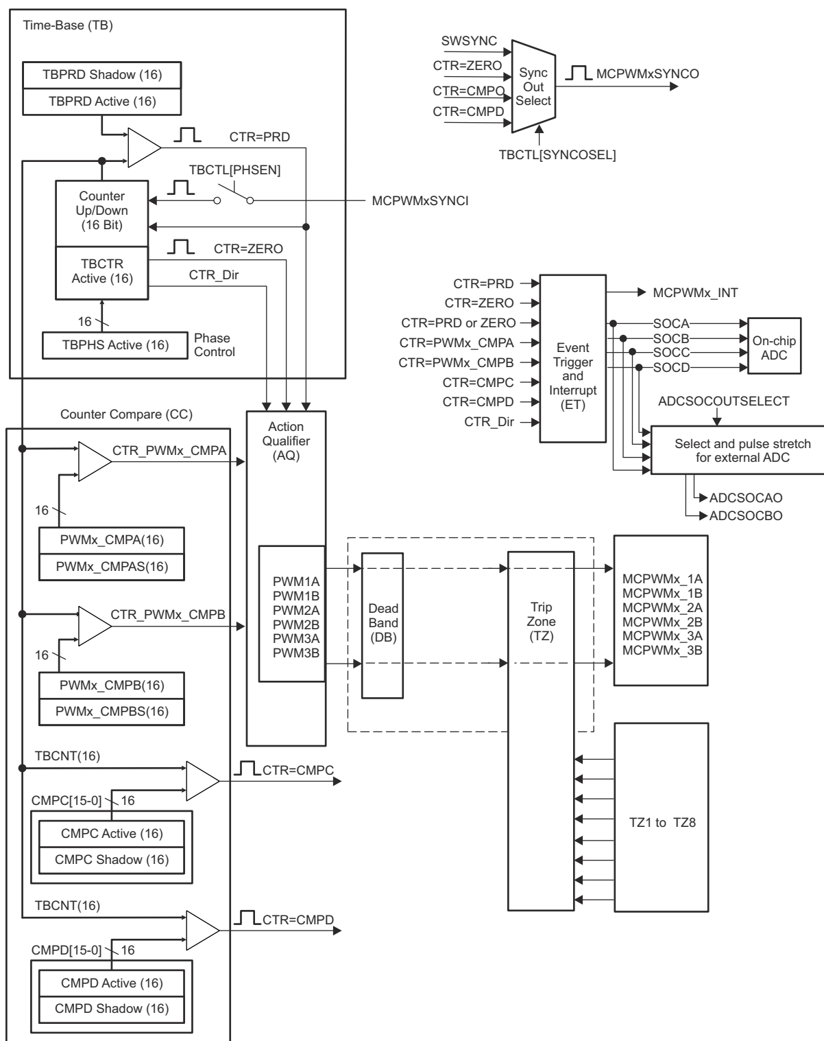
Figure 26-2. MCPWM Modules and Critical Internal Signal Interconnects
