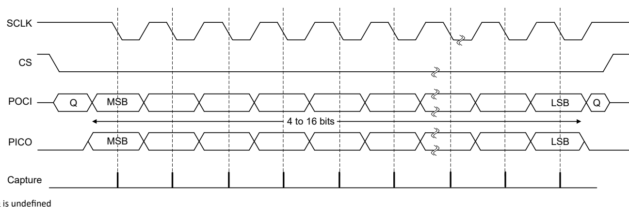
Figure 31-5. Motorola SPI Frame Format With SPO = 1 and SPH = 0
