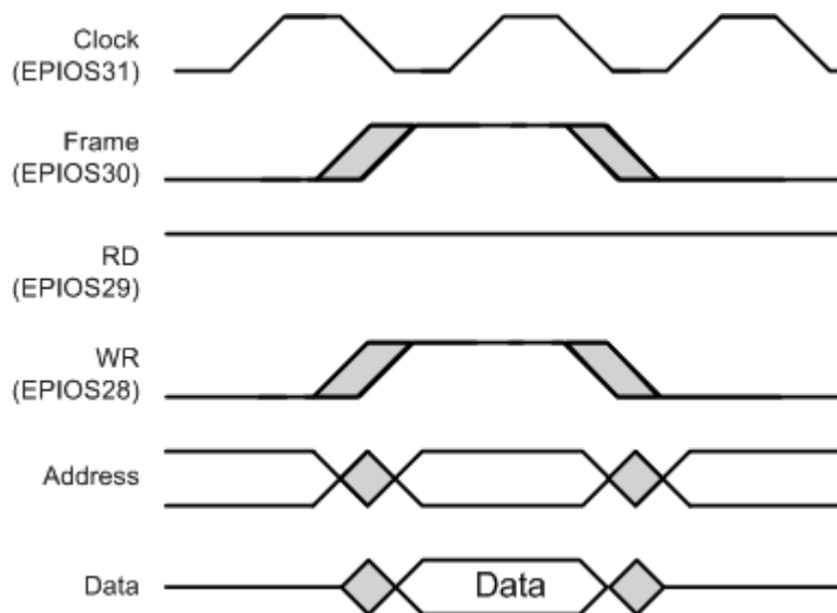
Figure 16-19. Single-Cycle Single Write Access, FRM50 = 0, FRMCNT = 0, WR2CYC = 0
