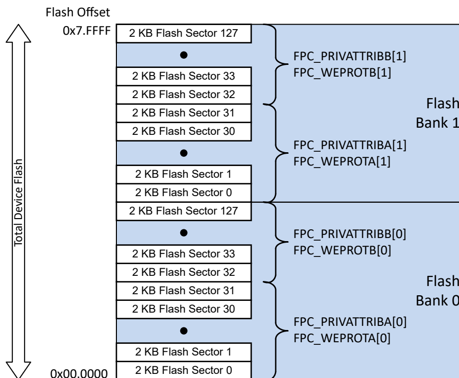
Figure 15-4. Flash Sector Mapping
