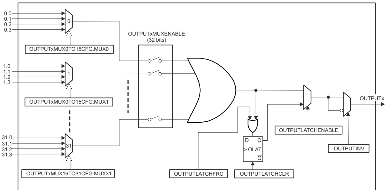
Figure 20-4. GPIO Output X-BAR Architecture
