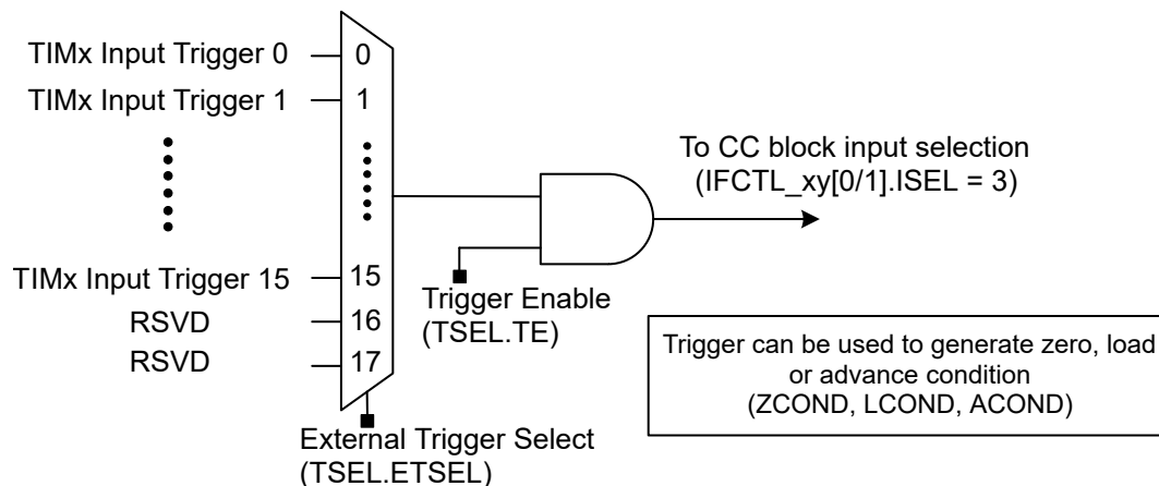
Figure 18-24. Secondary Timer Cross Trigger Input Configuration
