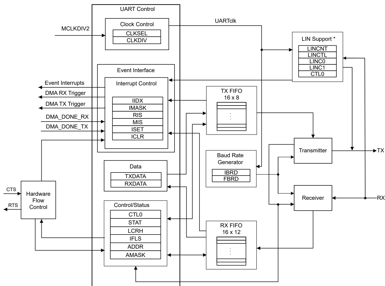
Figure 29-1. UART Functional Block Diagram
