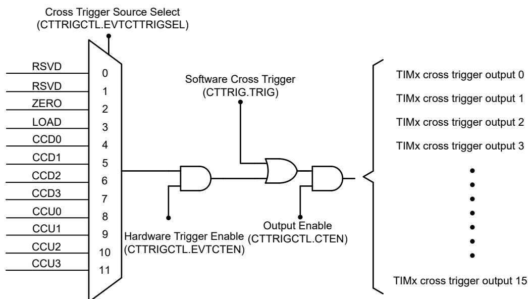
Figure 18-23. Main Timer Cross Trigger Output Configuration
