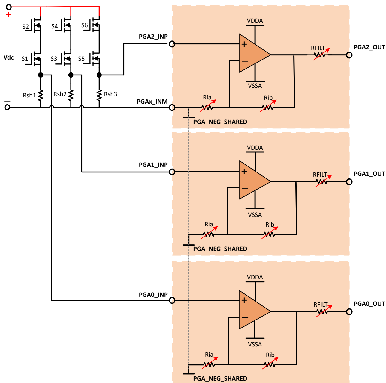
Figure 23-13. Three-phase Current Sensing Using PGA_NEG_SHARED Feature
