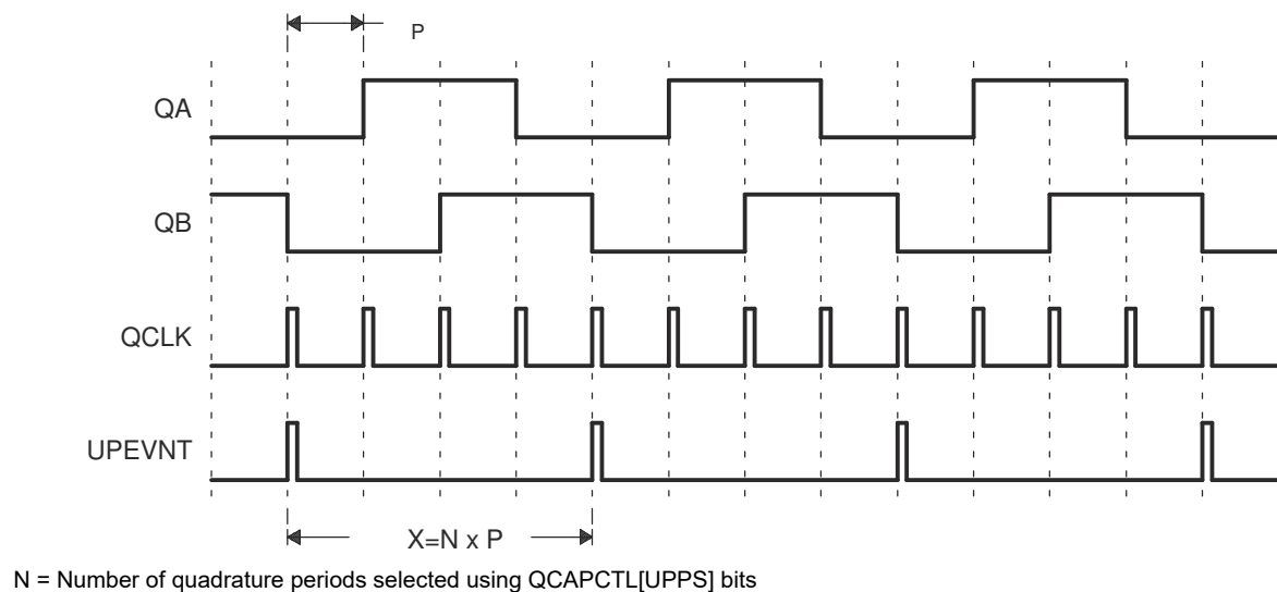
Figure 25-18. Unit Position Event for Low Speed Measurement (QCAPCTL[UPPS] = 0010)
