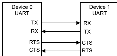
Figure 29-10. Flow Control
