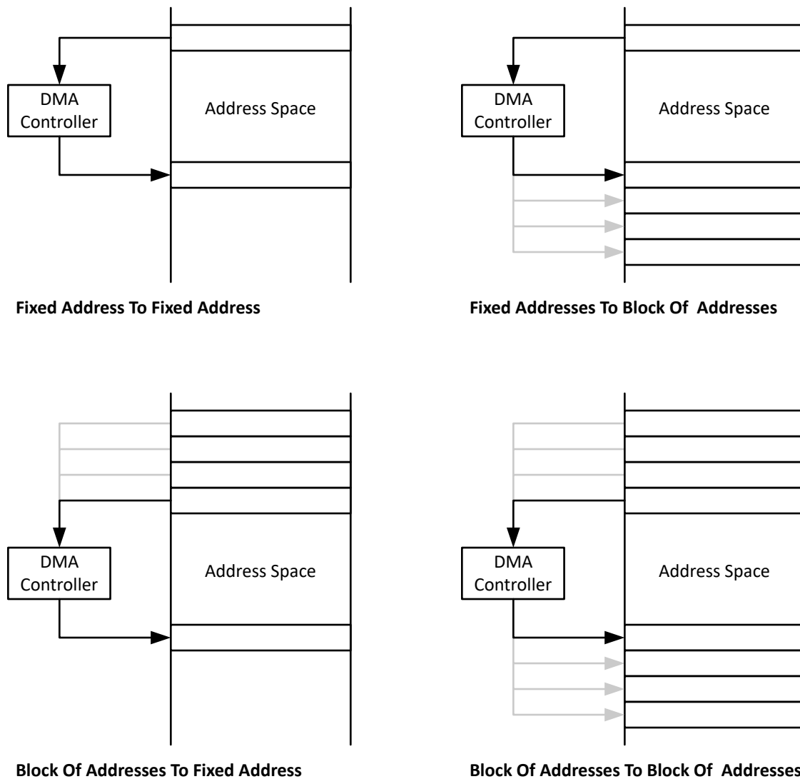
Figure 11-3. DMA Basic Addressing Modes
