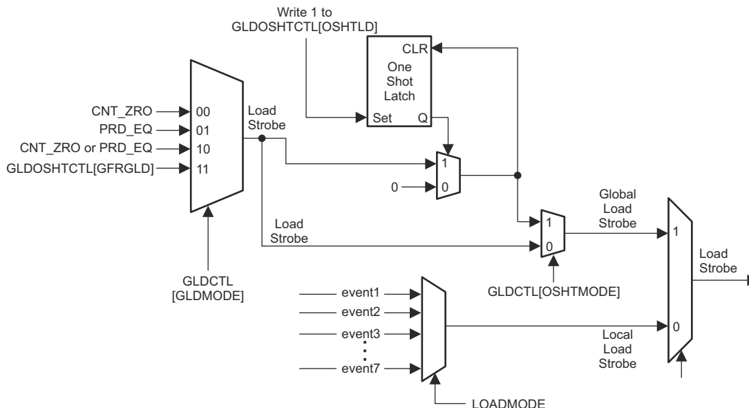
Figure 26-11. Global Load: Signals and Registers
