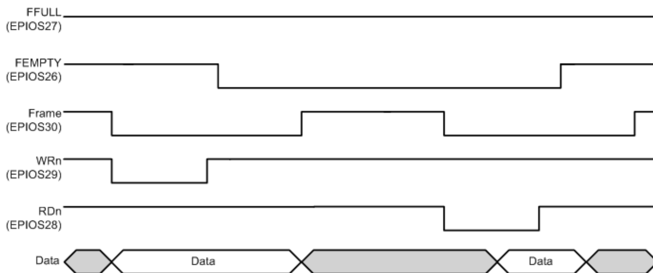
Figure 16-17. Write Followed by Read to External FIFO
