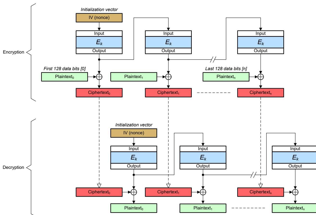
Figure 8-4. OFB Cipher
