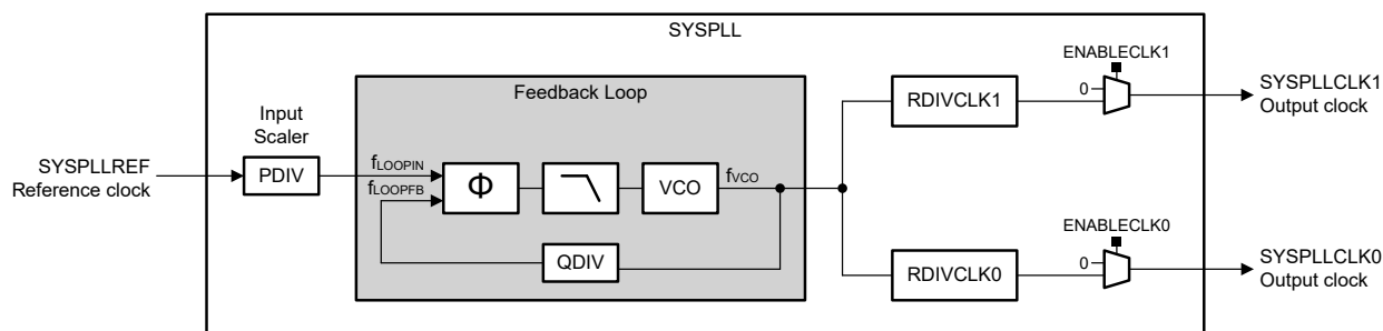
Figure 3-8. SYSPLL Diagram
