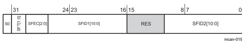
Figure 27-24. Standard Message ID Filter Element Structure
