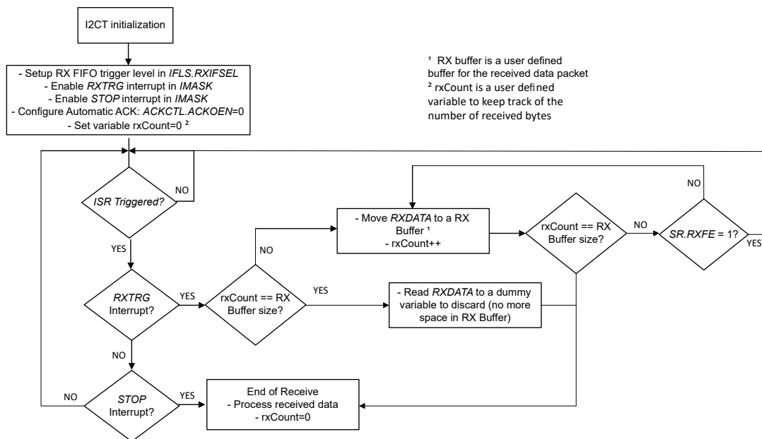
Figure 30-17. Target Receiver Mode using RXTRG and Automatic ACK
