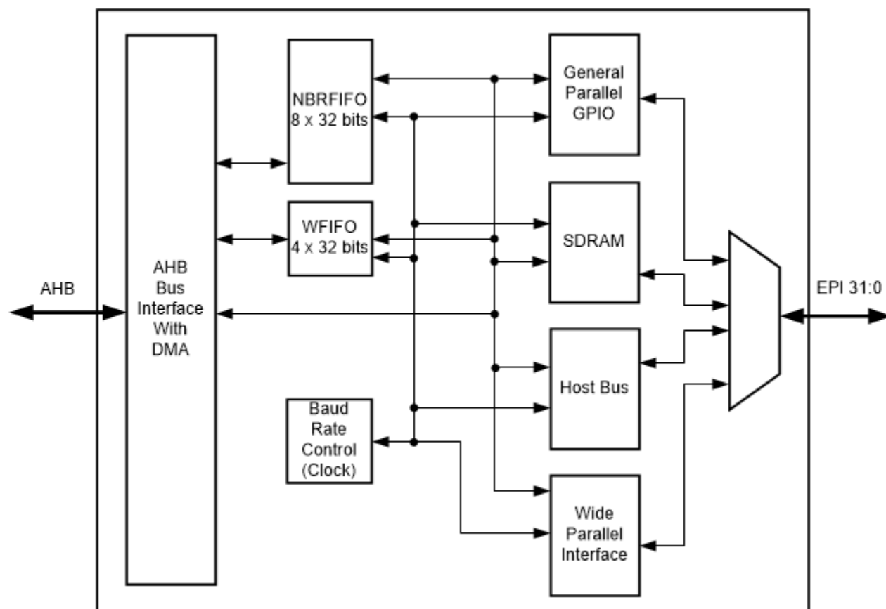
Figure 16-1. EPI Block Diagram
