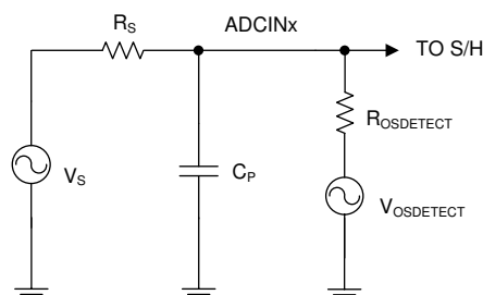
Figure 21-10. Input Circuit Equivalent with OSDETECT Enabled
