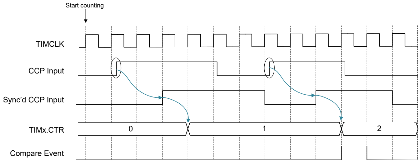
Figure 18-15. Edge Count Operation to Generate Compare Event (TIMx.CC = 2)
