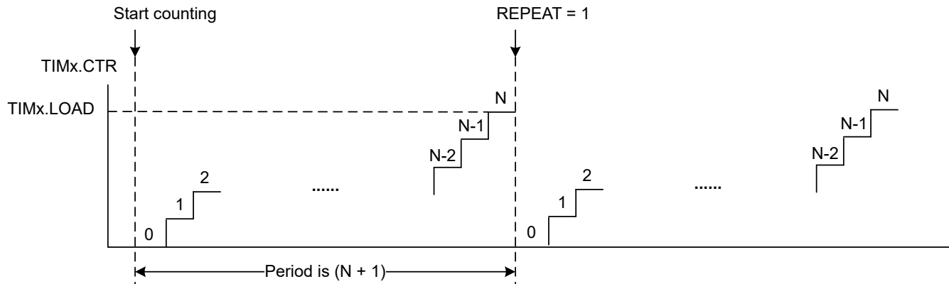
Figure 18-7. Up Counting Mode, CVAE = 2
