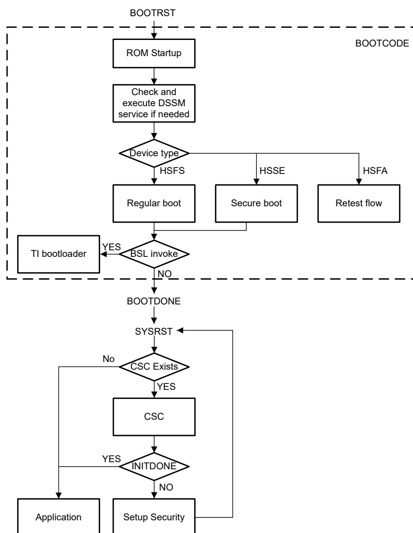
Figure 5-2. AM13E230x Secure Boot and Startup Sequence
