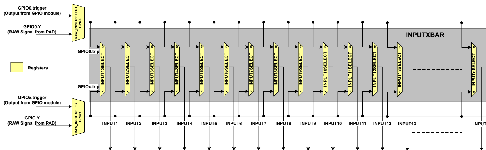
Figure 20-1. Input X-BAR Architecture
