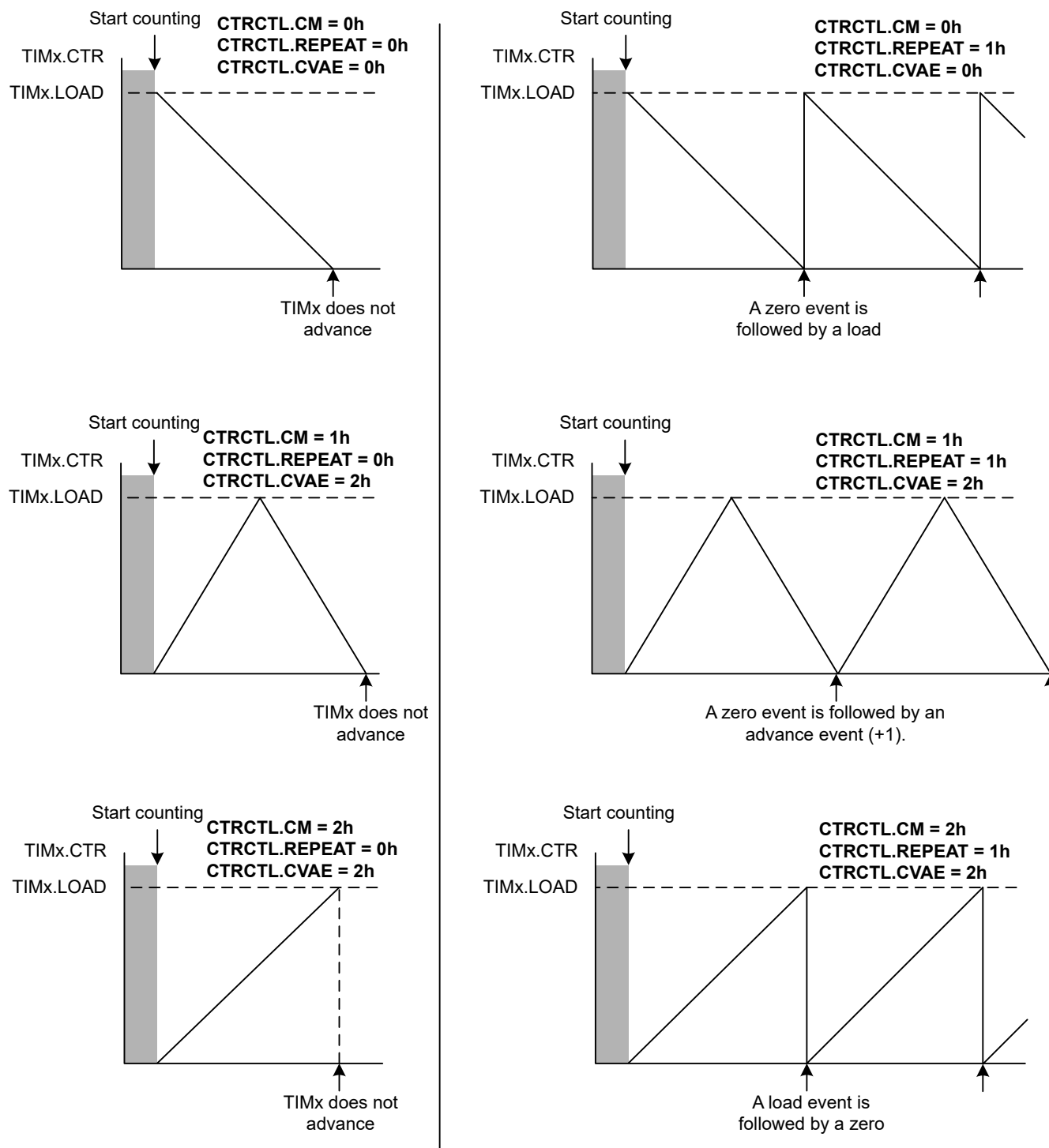
Figure 18-2. One-shot and Periodic Mode Behavior
