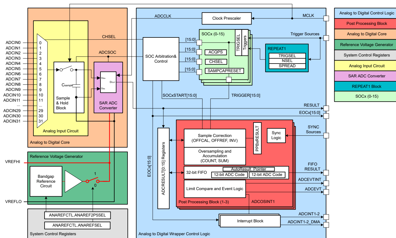
Figure 21-1. ADC Module Block Diagram
