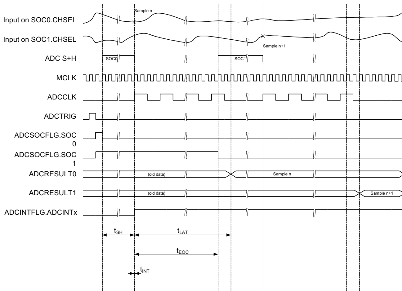
Figure 21-12. ADC Timings for 12-bit Mode in Late Interrupt Mode
