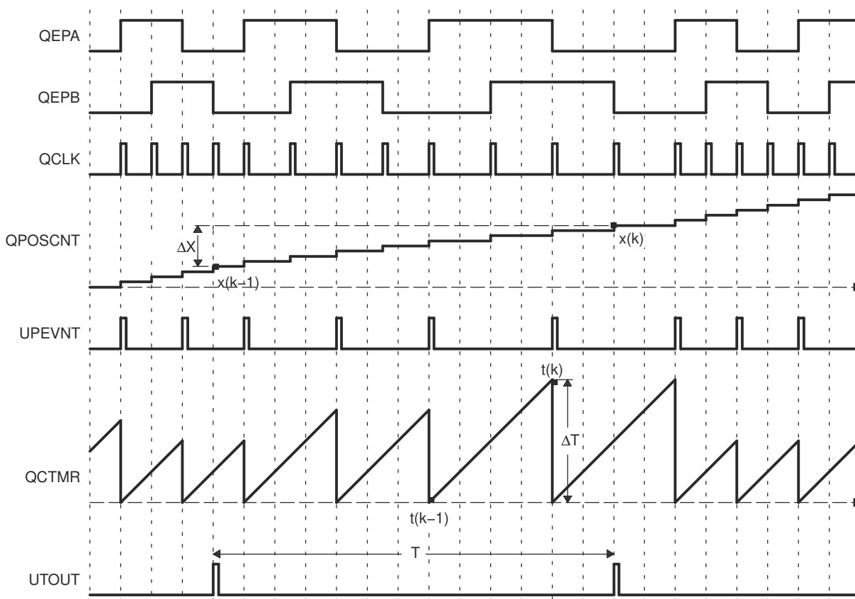
Figure 25-19. eQEP Edge Capture Unit - Timing Details
