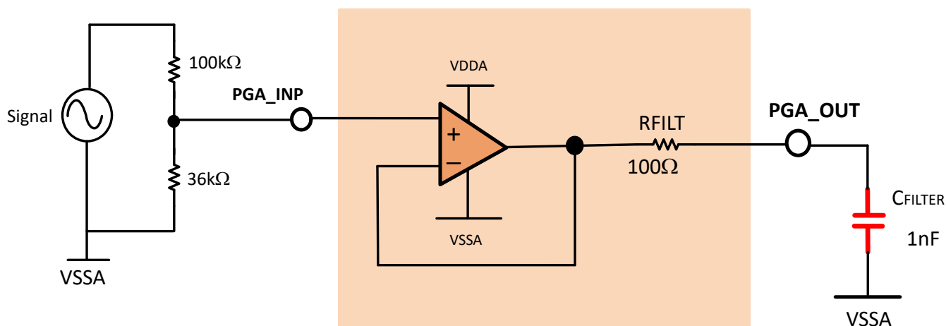
Figure 23-16. Buffer Mode Example
