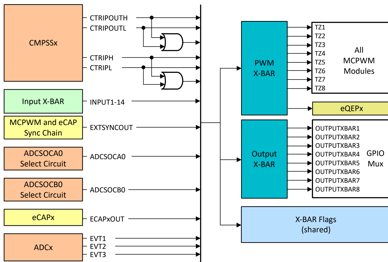
Figure 20-5. X-BAR Input Sources
