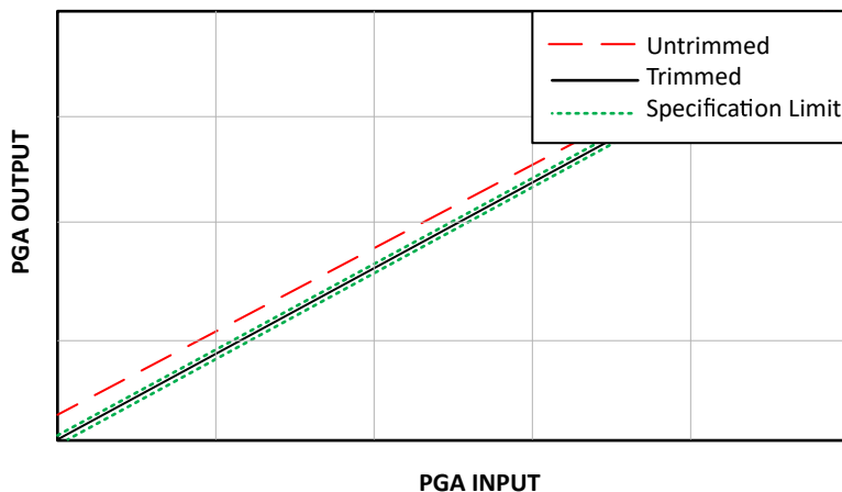
Figure 23-7. PGA Offset Trim
