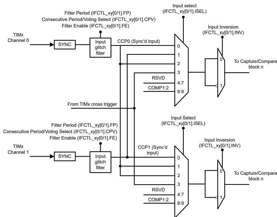
Figure 18-9. TIMx Capture Block Diagram
