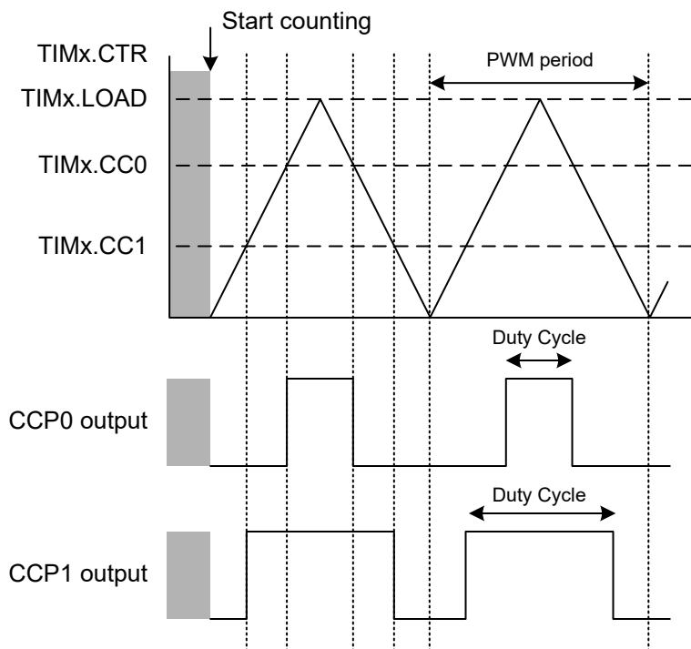
Figure 18-21. Center-Aligned PWM
