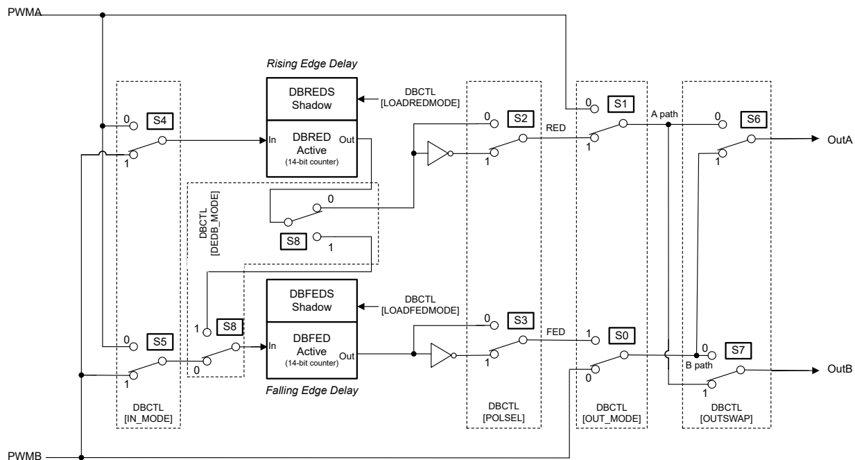
Figure 26-30. Configuration Options for the Dead-Band Submodule
