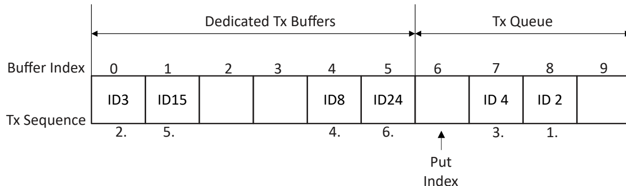
Figure 27-15. Mixed Dedicated Tx Buffers/ Tx FIFO (Example)
