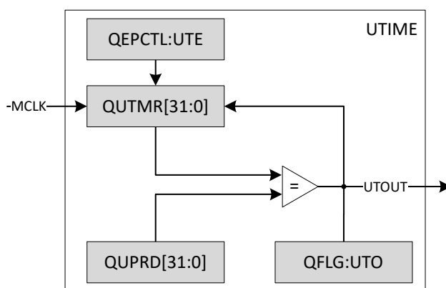
Figure 25-21. eQEP Unit Timer Base
