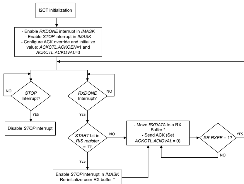
Figure 30-16. Target Receiver Mode using RXDONE and ACK Override
