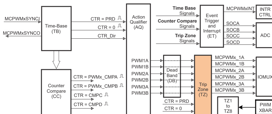
Figure 26-32. Trip-Zone Submodule
