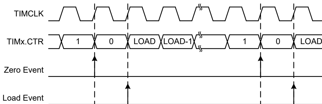
Figure 18-4. Down Counting Mode Event Generation
