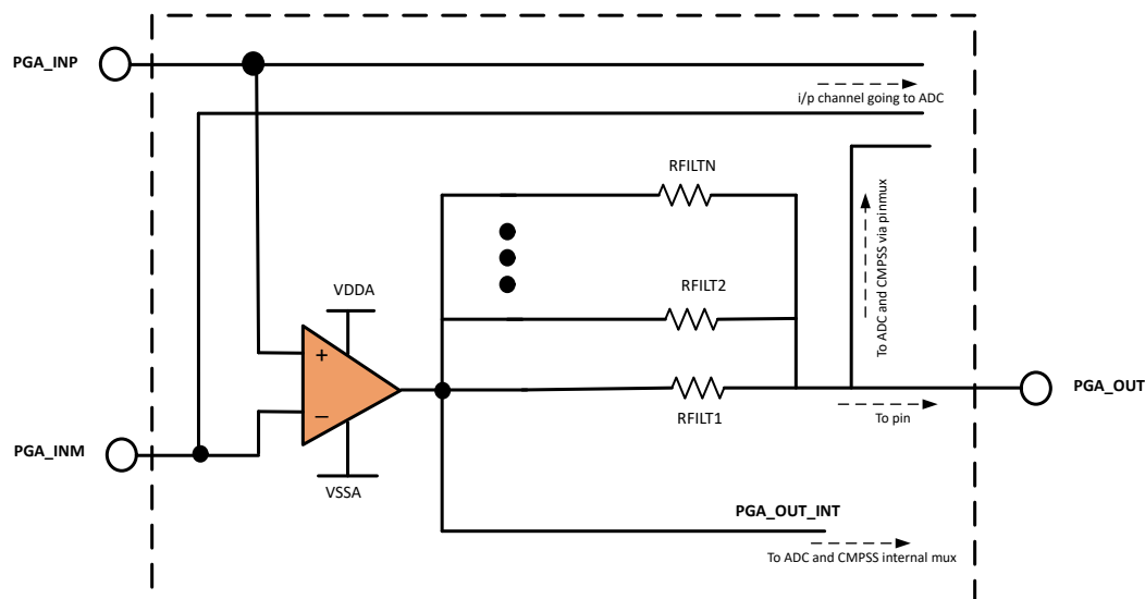
Figure 23-3. Standalone Mode
