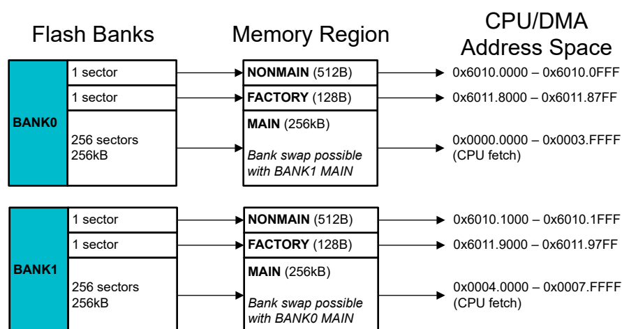
Figure 13-3. Memory Organization Example - Multiple Bank Configuration
