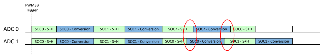
Figure 21-16. Example: Asynchronous Operation with Uneven SOC Numbers – Trigger Overflow
