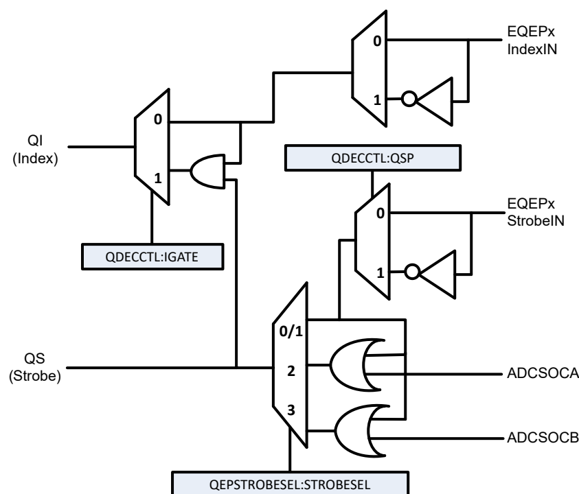
Figure 25-13. Latching Position Counter on ADCSOCA/ADCSOCB Event
