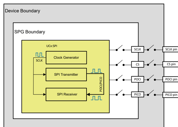
Figure 31-2. SPI Internal Loopback
