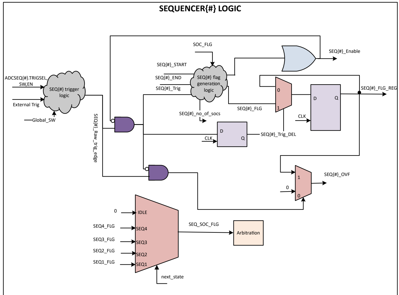
Figure 21-4. Sequencer Enable and Overflow Logic
