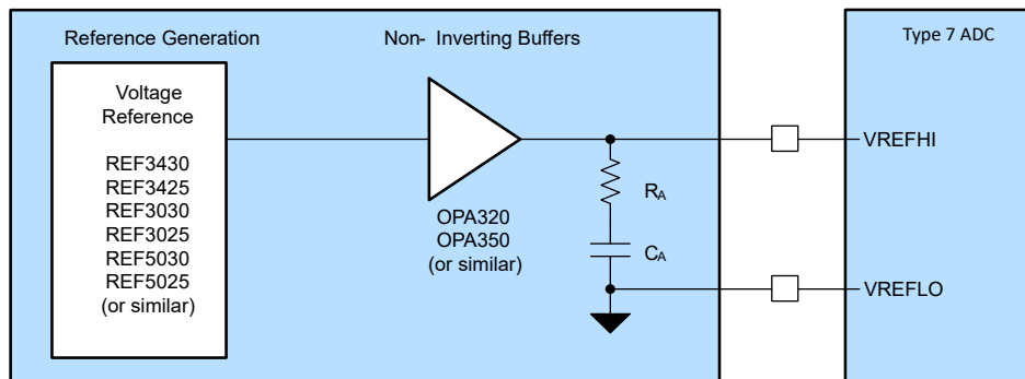
Figure 21-18. ADC Reference System
