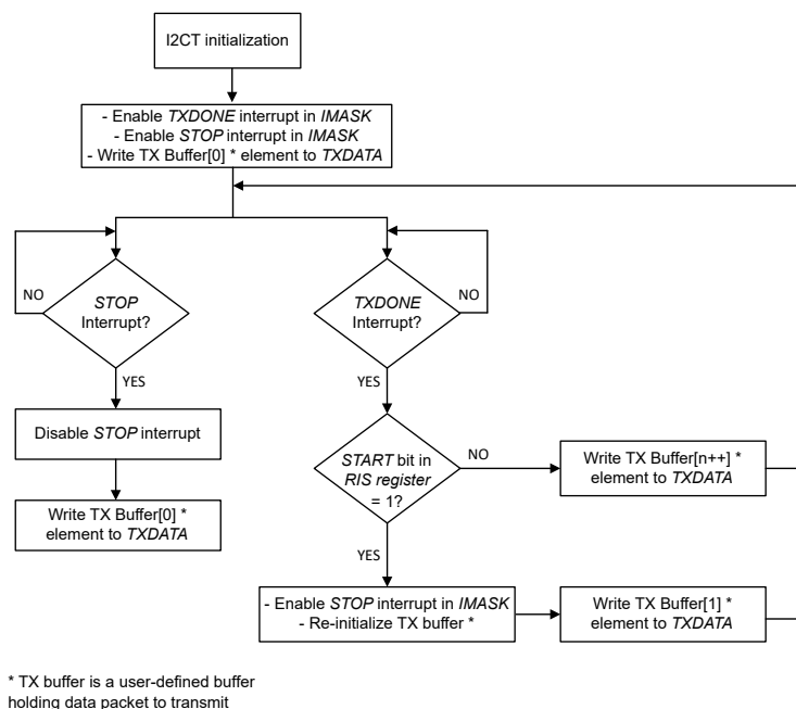
Figure 30-18. Target Transmitter Mode using TXDONE
