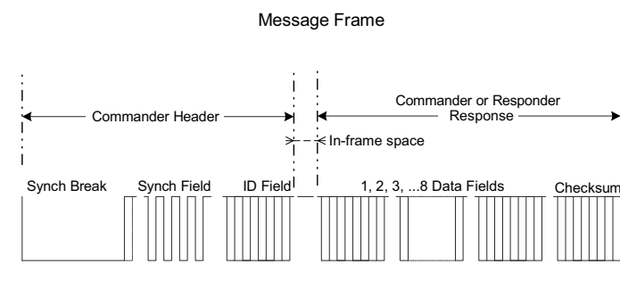
Figure 29-6. LIN Protocol Message Structure
