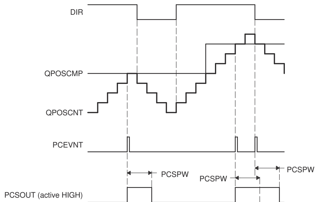
Figure 25-16. eQEP Position-compare Sync Output Pulse Stretcher
