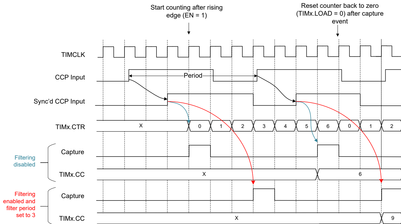
Figure 18-12. Period Capture Mode in Up-Counting Mode, CVAE = 2
