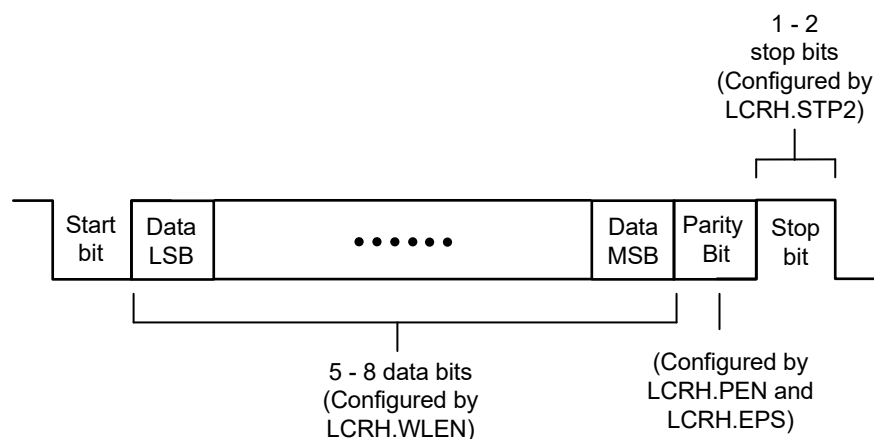
Figure 29-2. UART Character Frame
