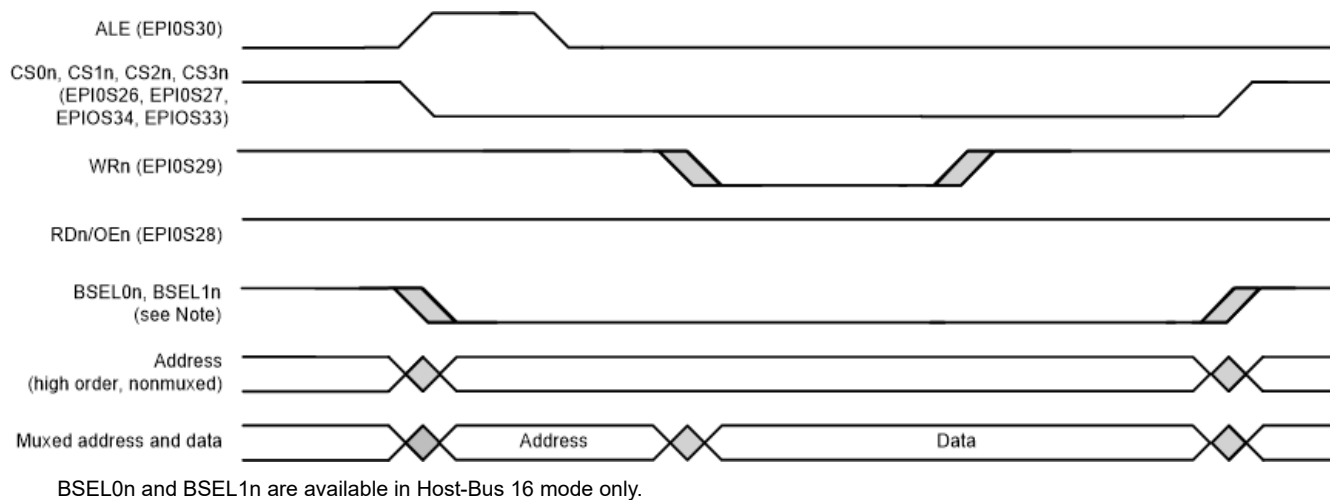
Figure 16-15. Host-Bus Write Cycle with Multiplexed Address and Data and ALE With Dual or Quad CSn
