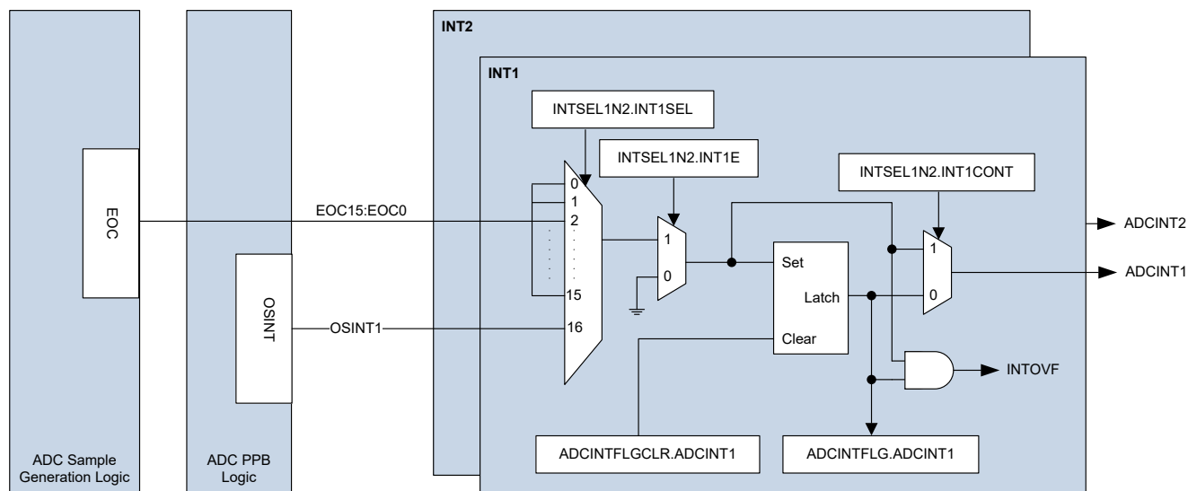
Figure 21-7. ADC End-of-Conversion (EOC) Signal Interrupts
