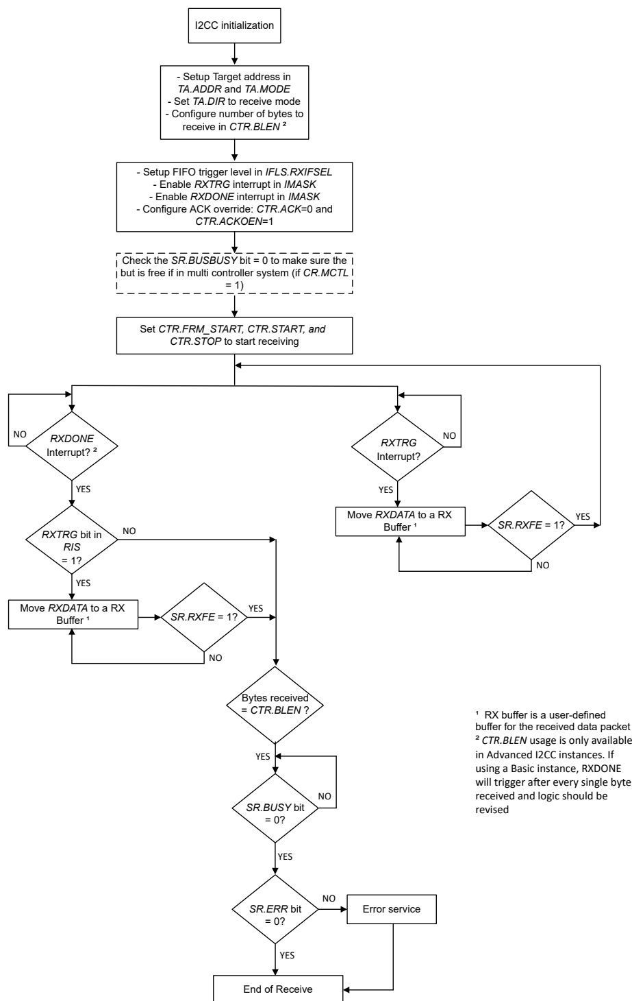
Figure 30-14. Controller Receive Mode
