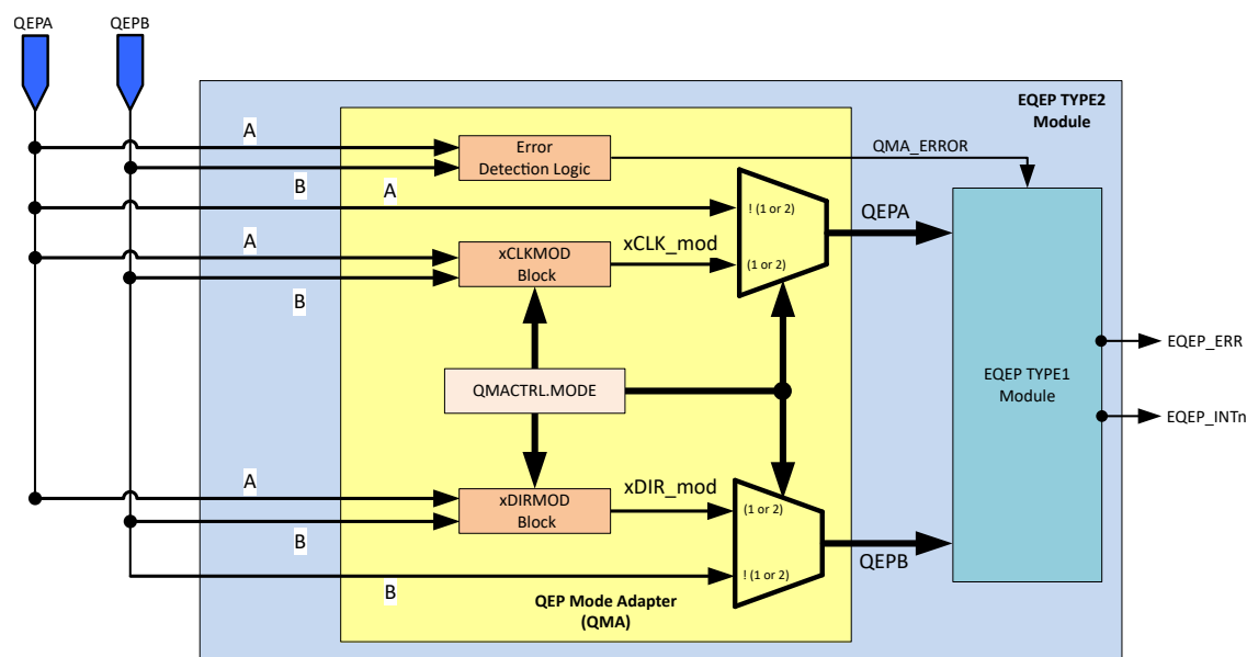
Figure 25-22. QMA Module Block Diagram
