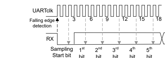
Figure 29-3. UART Oversampling mode
