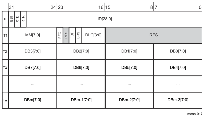
Figure 27-22. Tx Buffer Element Structure
