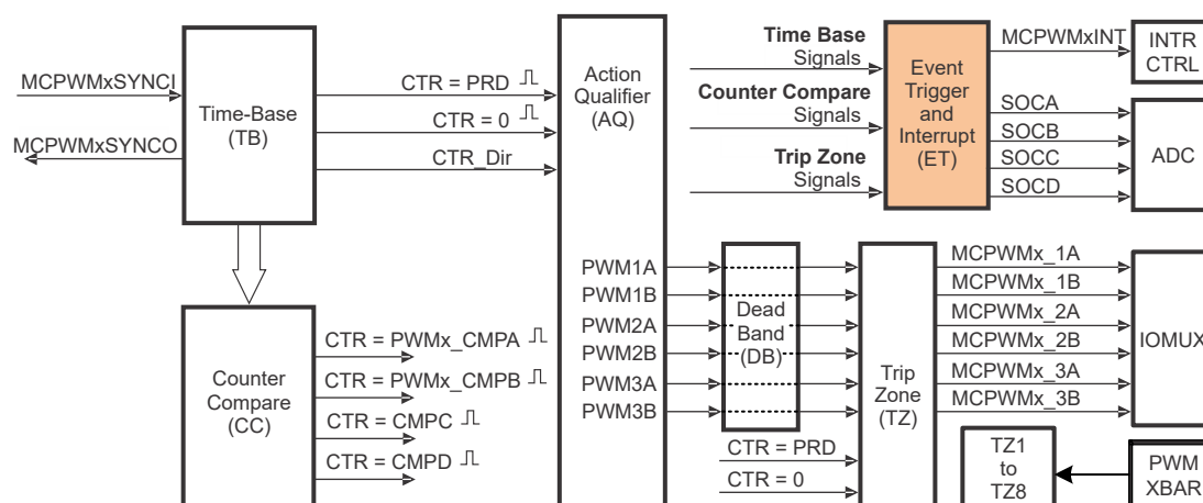
Figure 26-34. Event-Trigger Submodule
