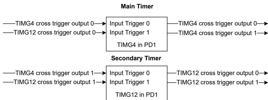
Figure 18-22. Cross Trigger Connections for Main Timer (TIMGx) and Secondary Timer (TIMAx) in Power Domain 1
