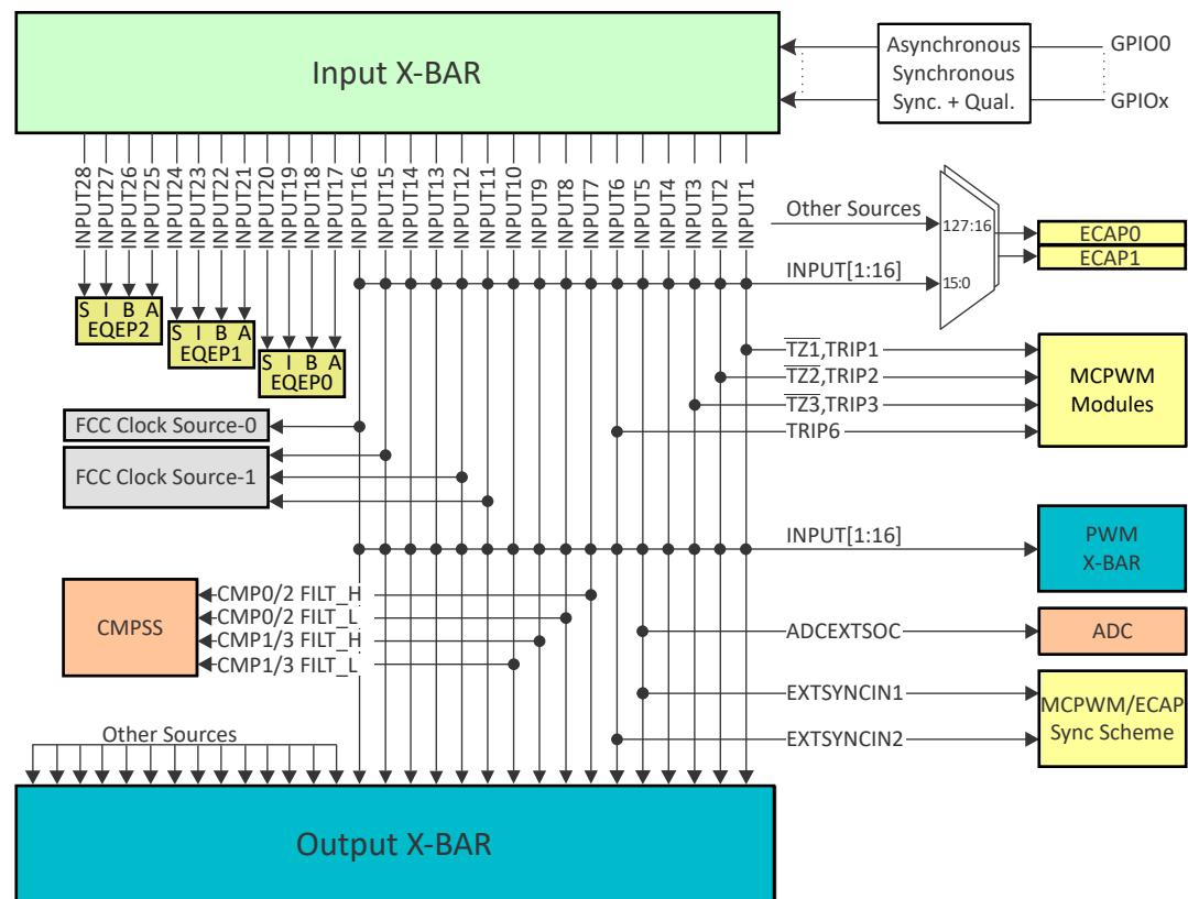
Figure 20-2. INPUTXBAR Connectivity
