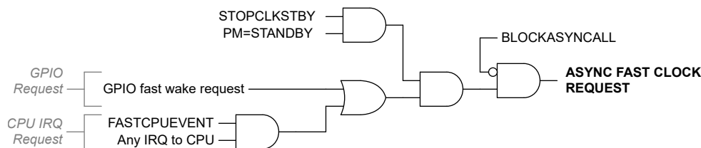
Figure 3-9. Asynchronous Fast Clock Request Logic
