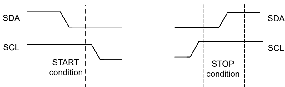
Figure 30-5. START and STOP Conditions
