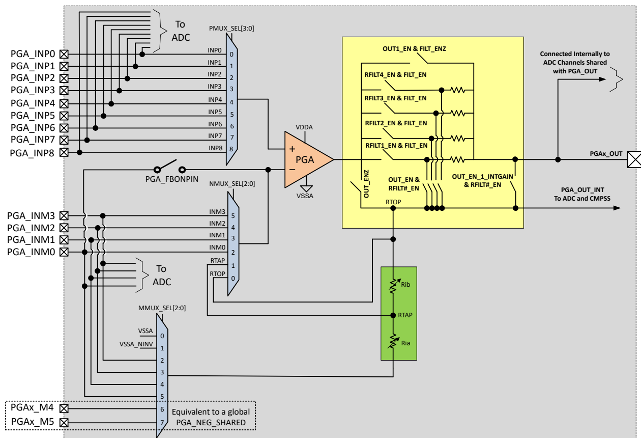
Figure 23-1. PGA Block Diagram
