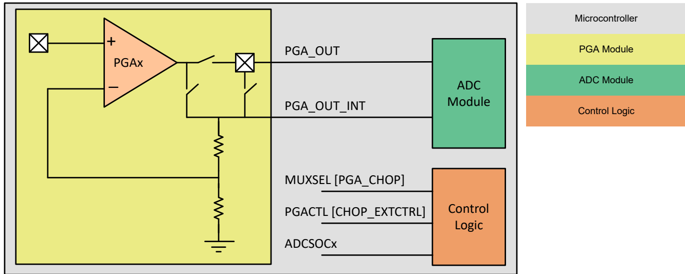
Figure 23-10. ADC-Assisted Chopping Block Diagram
