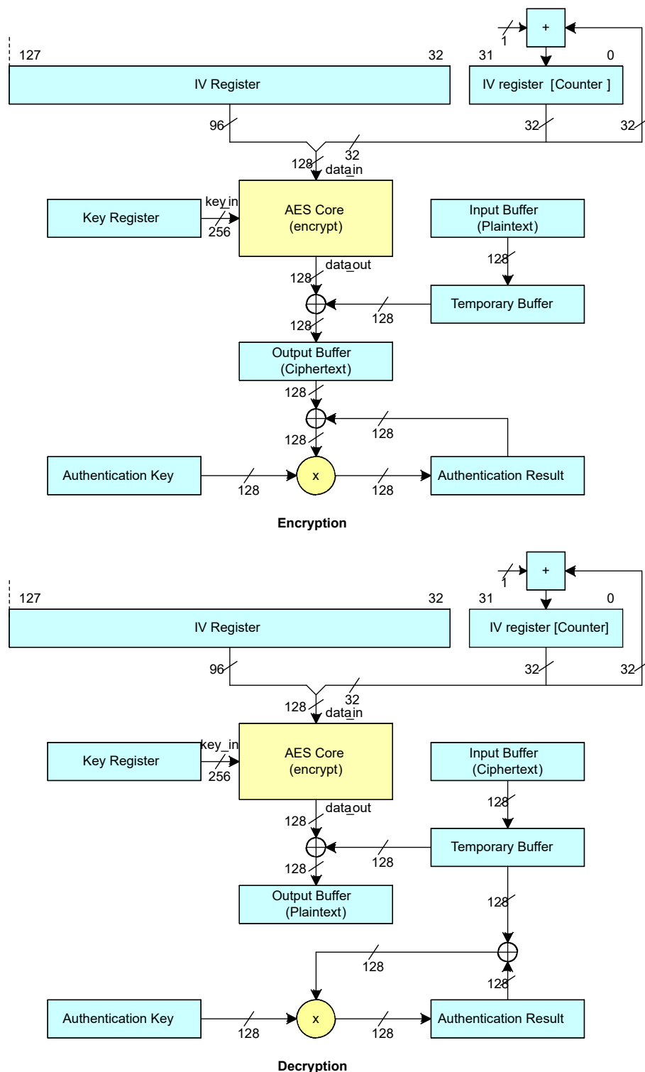
Figure 8-8. GCM Operation on a Block
