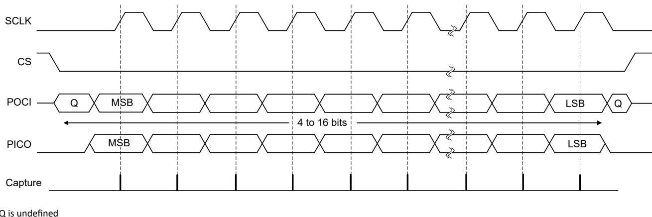
Figure 31-3. Motorola SPI Format With SPO = 0 and SPH = 0
