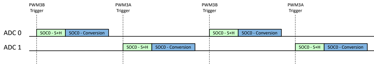
Figure 21-17. Example: Synchronous Equivalent Operation with Non-Overlapping Conversions
