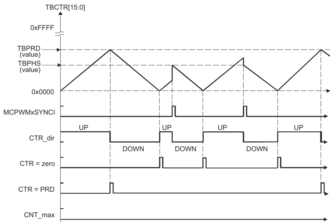
Figure 26-9. Time-Base Up-Down Count Waveforms, TBCTL[PHSDIR = 0] Count Down On Synchronization Event
