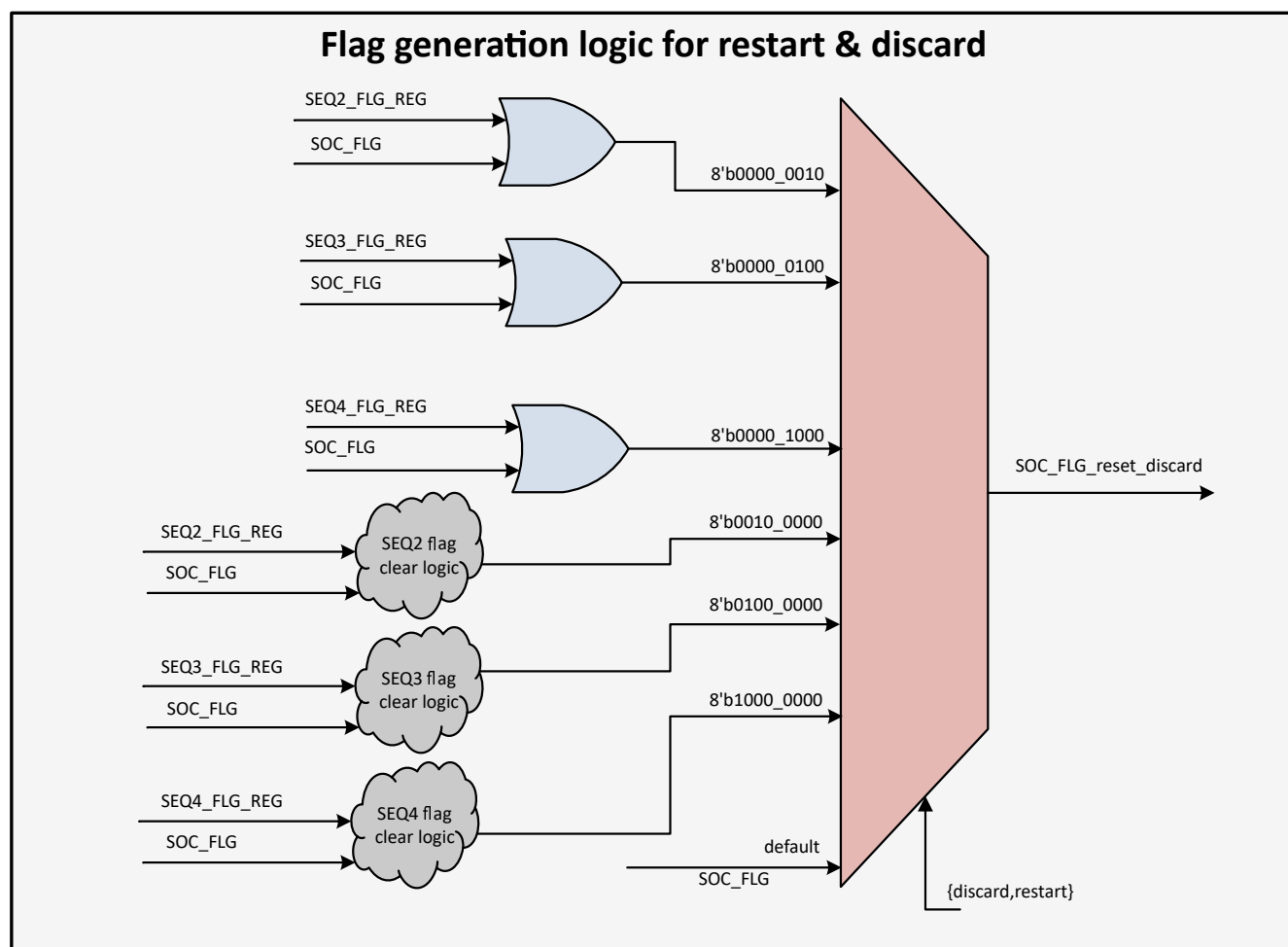
Figure 21-5. Sequencer Pre-empt Restart & Discard Logic
