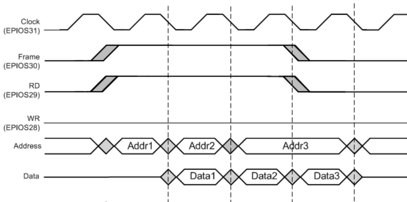
Figure 16-21. Read Accesses, FRM50 = 0, FRMCNT = 0
