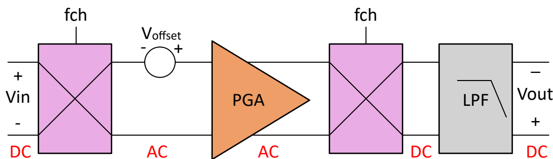
Figure 23-9. General Chopping Technique
