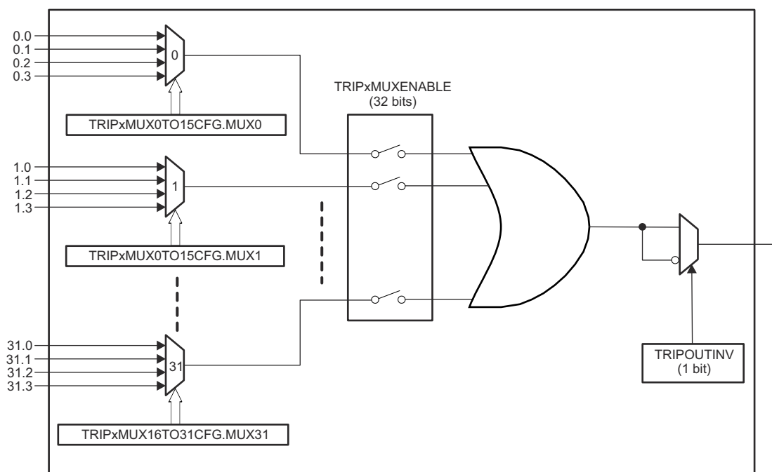
Figure 26-38. PWM X-BAR Architecture - Single Output
