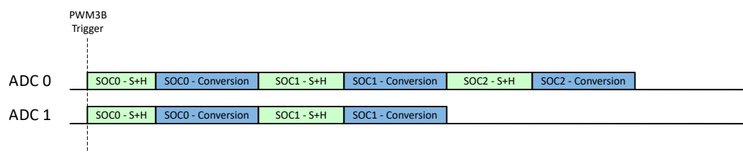
Figure 21-15. Example: Synchronous Operation with Uneven SOC Numbers
