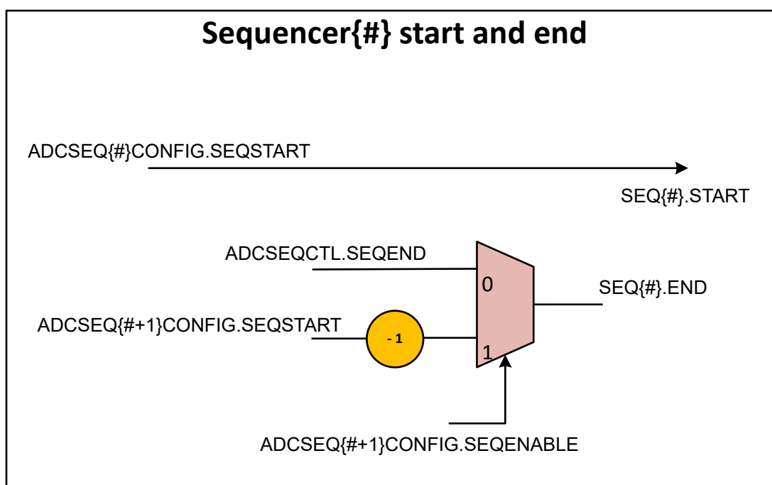
Figure 21-3. Sequencer start and end
