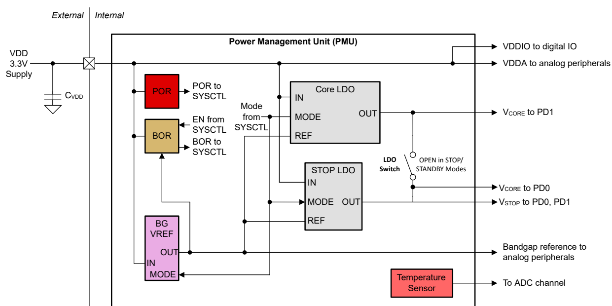
Figure 3-4. PMU Block Diagram
