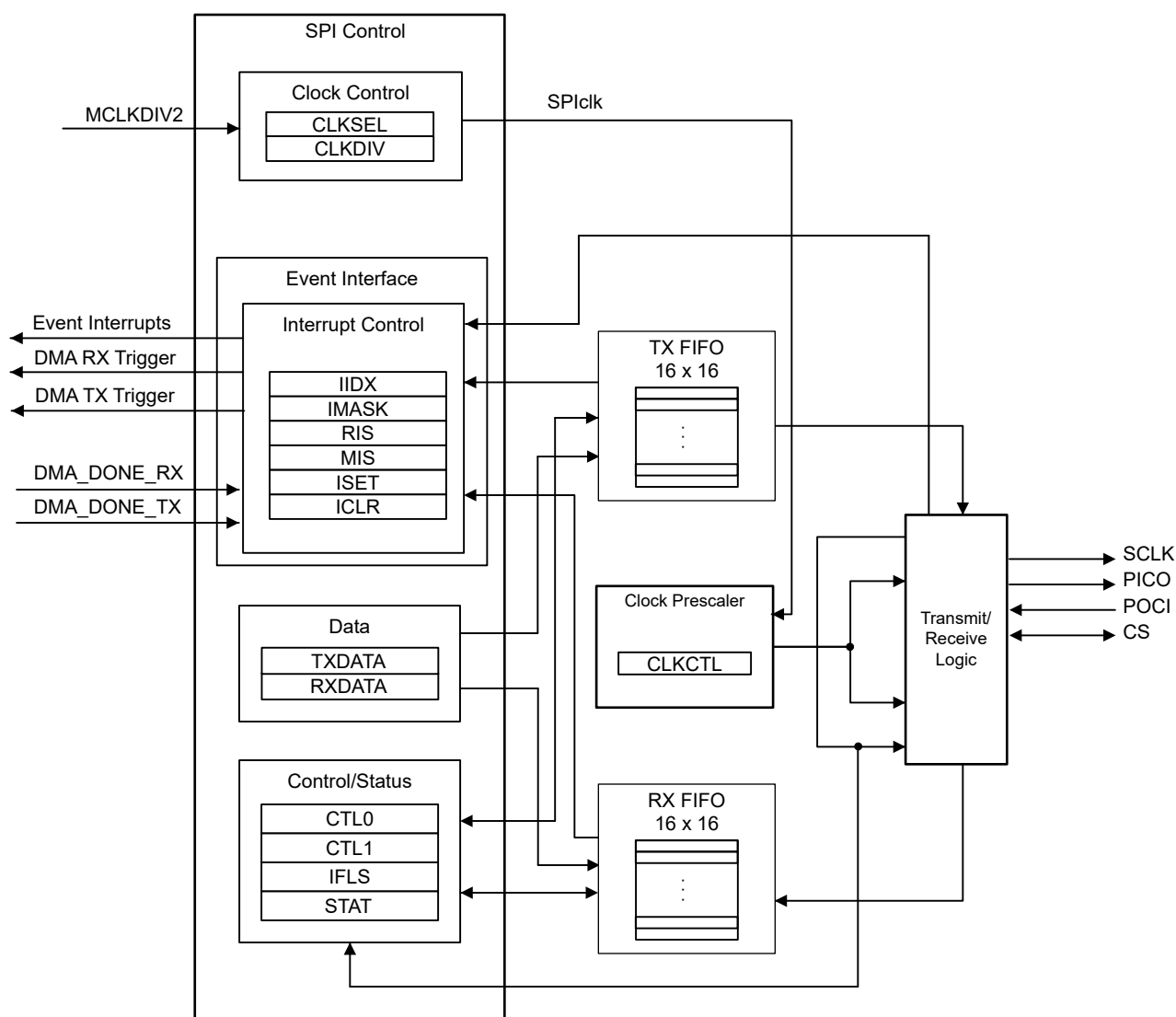
Figure 31-1. SPI Functional Block Diagram
