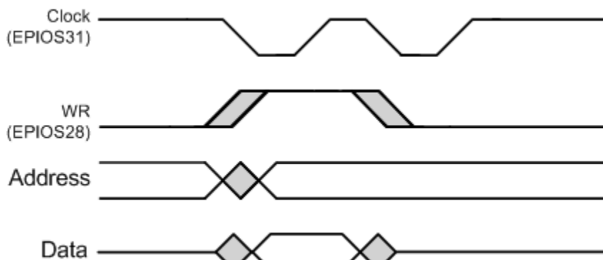
Figure 16-29. EPI Clock Operation, CLKGATE = 1, WR2CYC = 1
