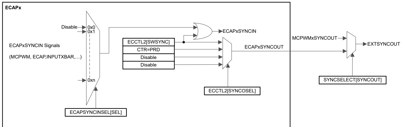
Figure 24-8. eCAP Synchronization Scheme
