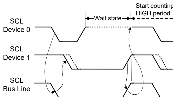
Figure 30-10. Clock Synchronization
