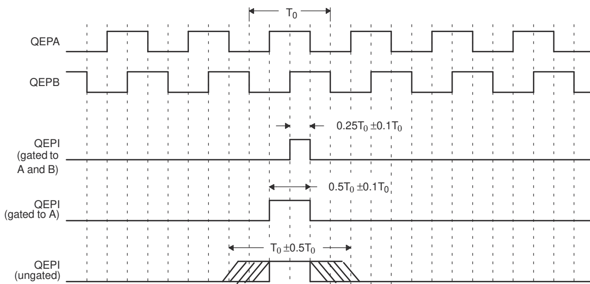
Figure 25-3. Index Pulse Example
