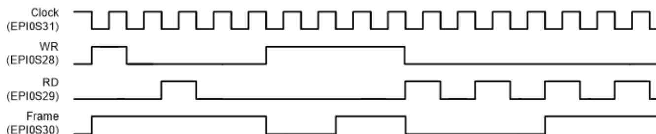
Figure 16-26. FRAME Signal Operation, FRM50 = 1 and FRMCNT = 1
