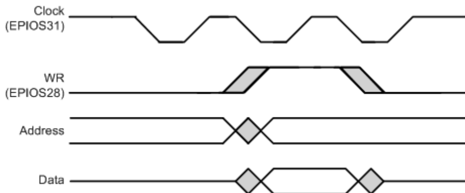
Figure 16-28. EPI Clock Operation, CLKGATE = 1, WR2CYC = 0
