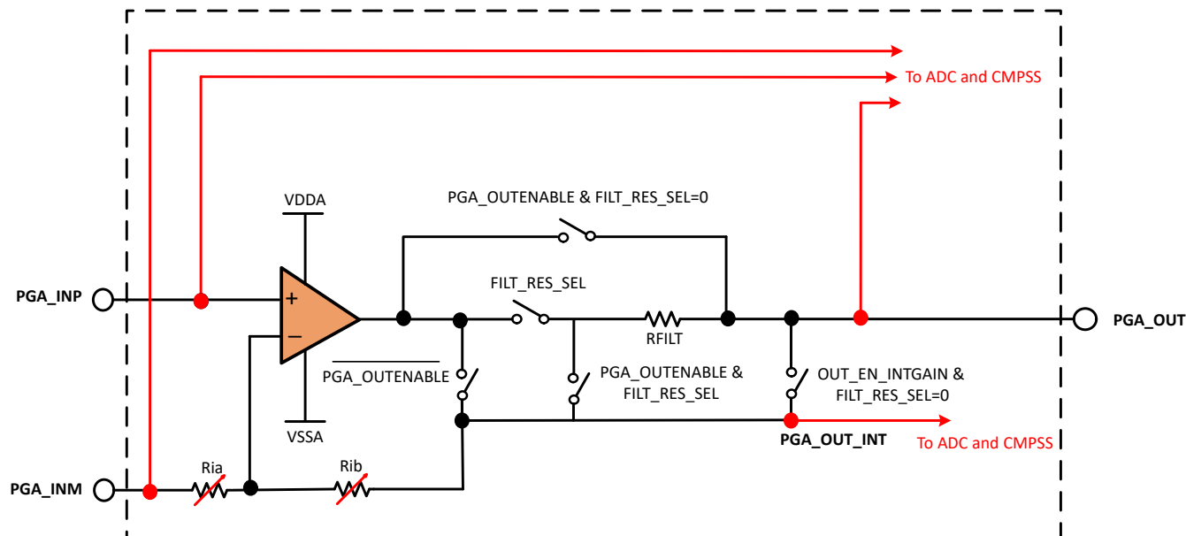
Figure 23-14. PGA Pin Alternate Functions
