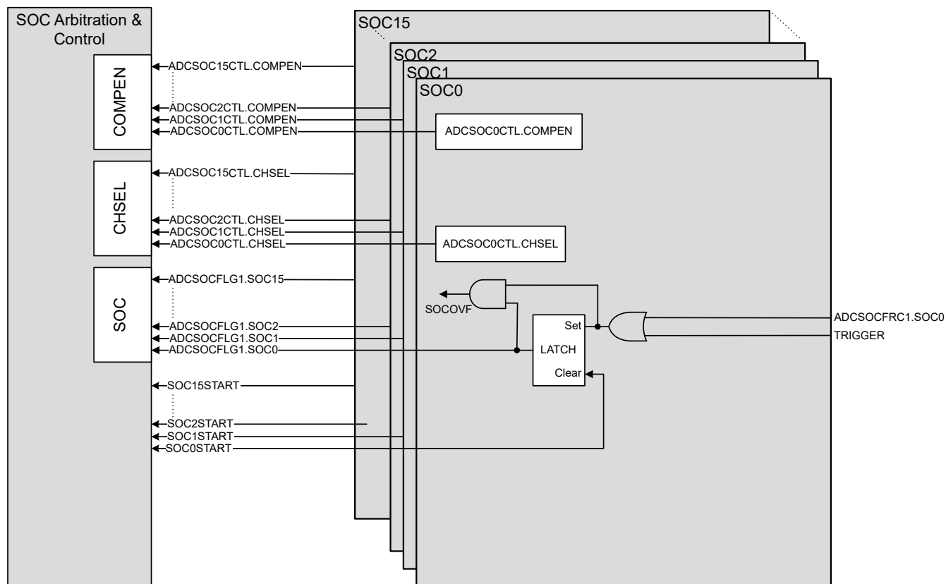
Figure 21-2. SOC Block Diagram
