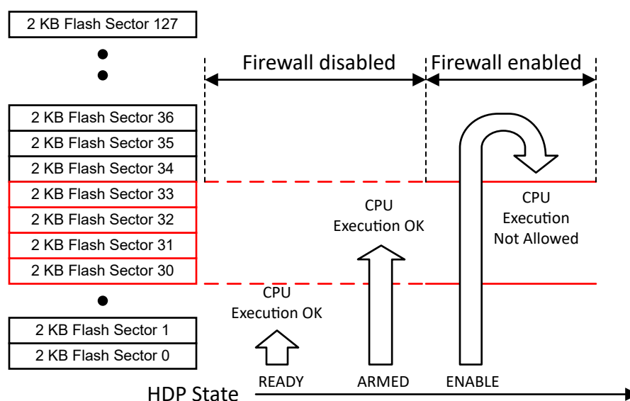
Figure 15-6. HDP Execution Flow
