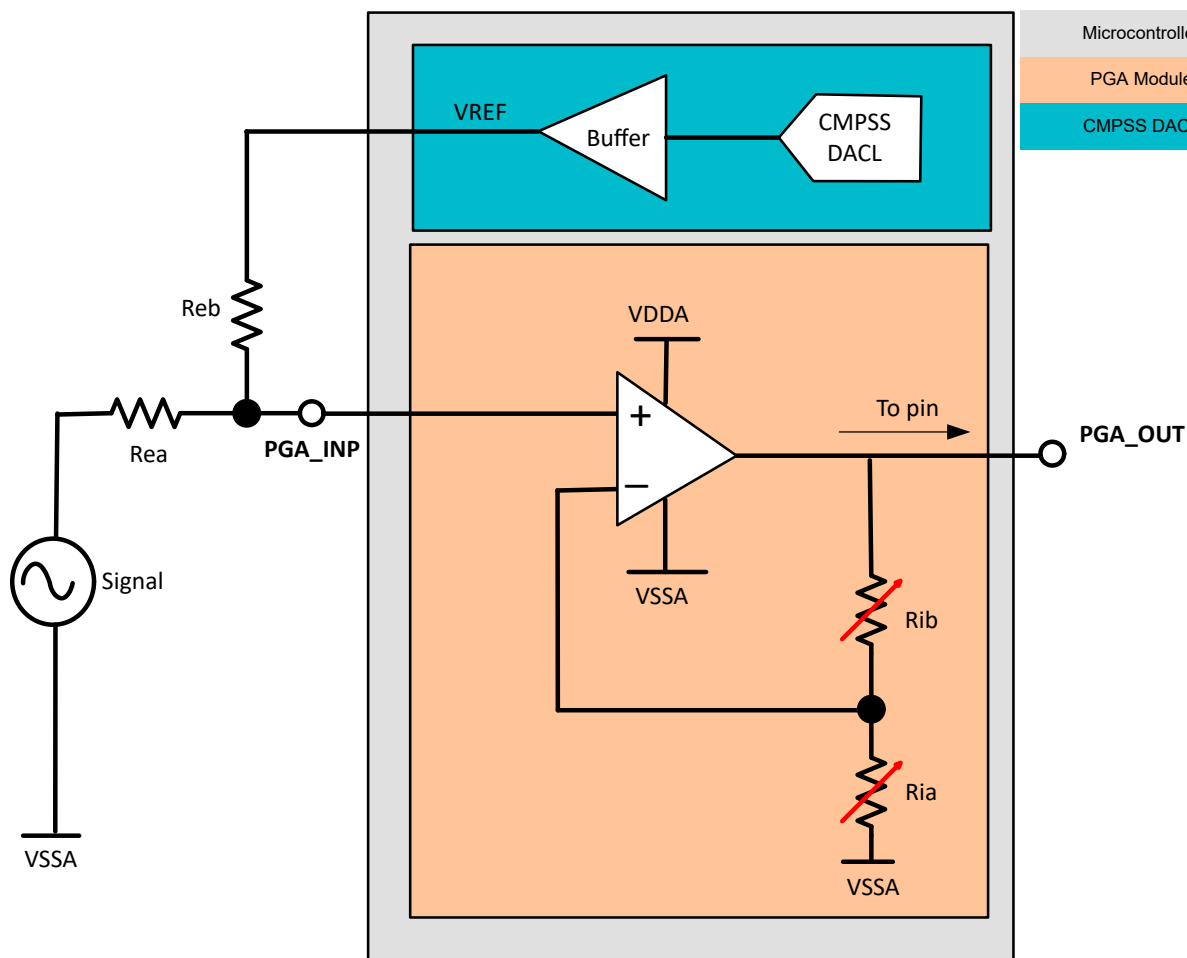
Figure 23-11. Level Shifting Using Internal DAC
