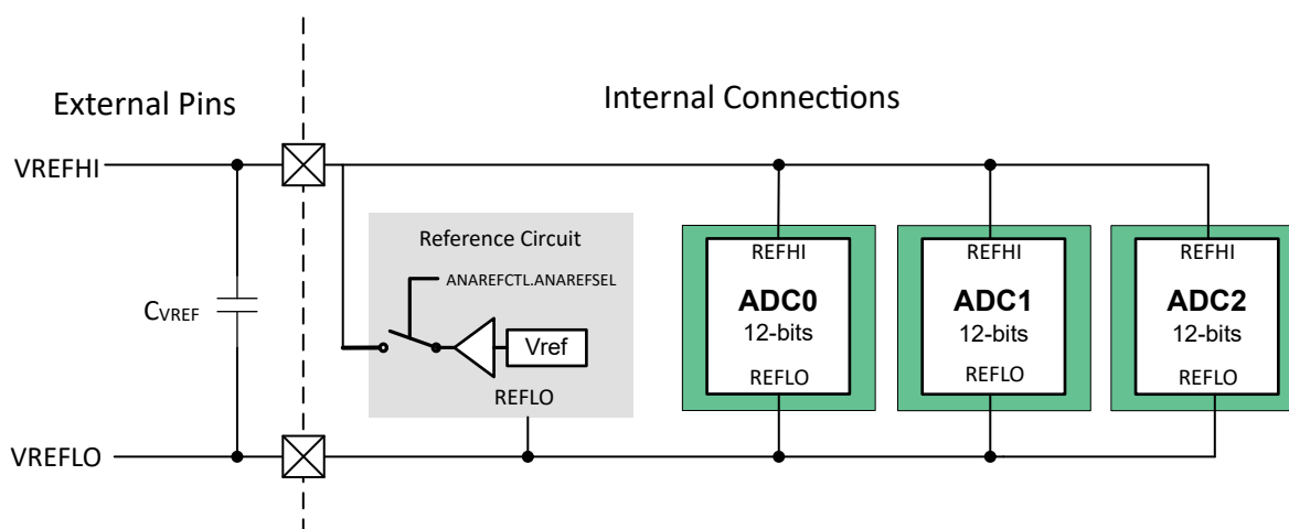
Figure 3-6. VREF to ADC Connections
