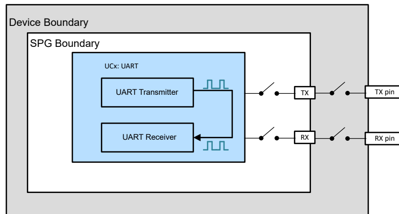
Figure 29-5. UART Internal Loopback
