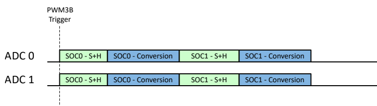
Figure 21-13. Example: Basic Synchronous Operation
