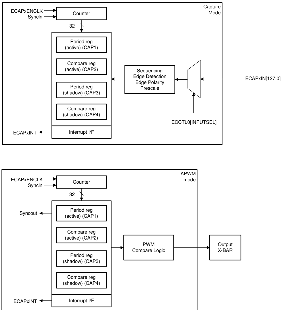
Figure 24-1. Capture and APWM Modes of Operation
