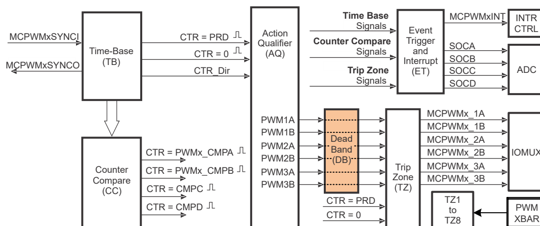
Figure 26-29. Dead-band Generator Submodule
