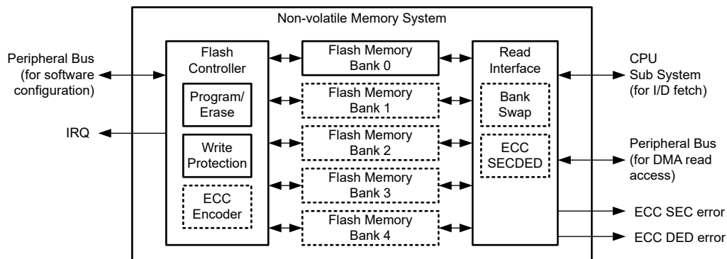
Figure 13-1. Non-volatile Memory System Components
