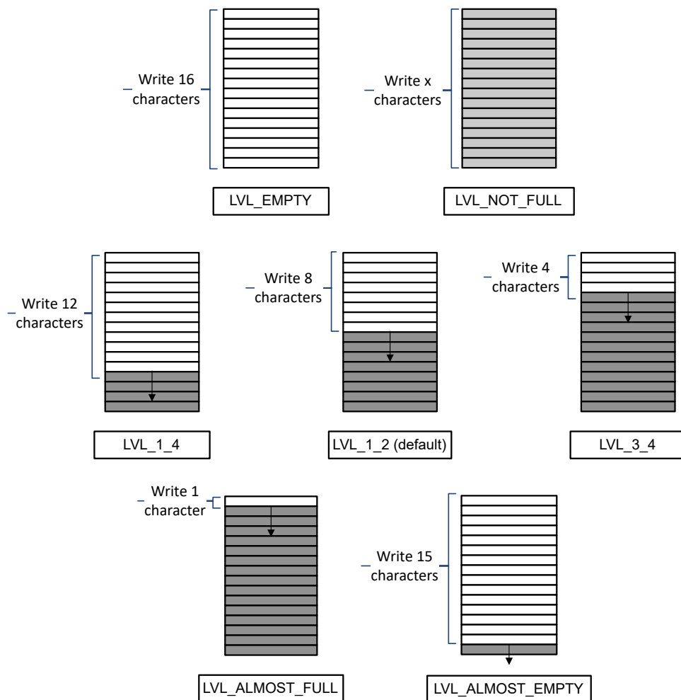
Figure 28-4. UNICOMM Transmit FIFO Levels
