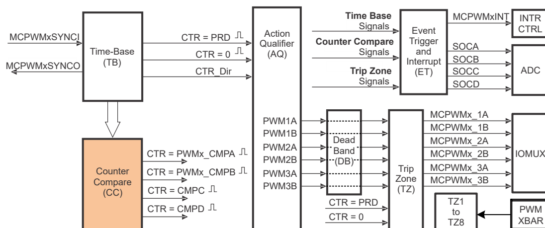
Figure 26-12. Counter-Compare Submodule
