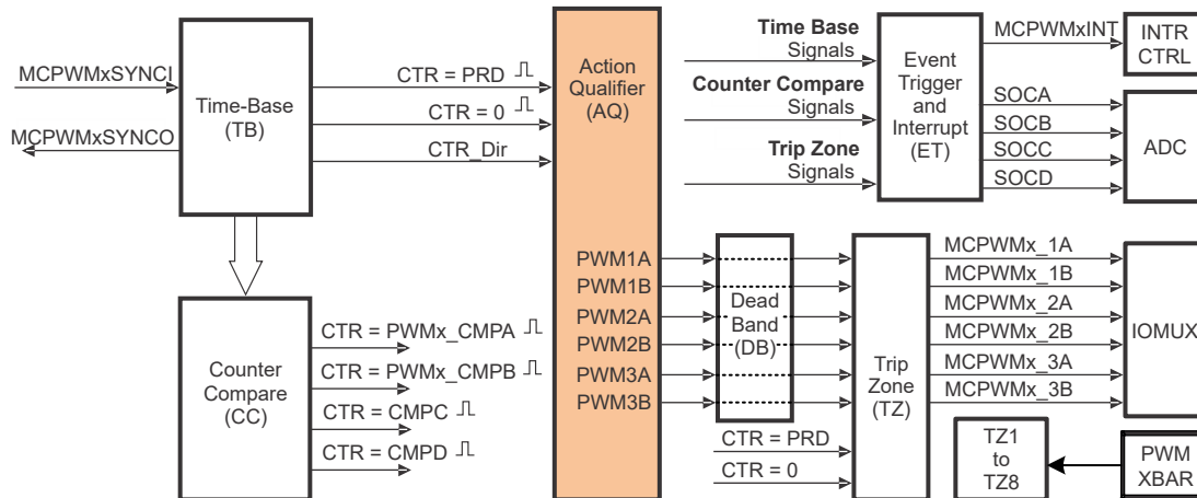
Figure 26-17. Action-Qualifier Submodule
