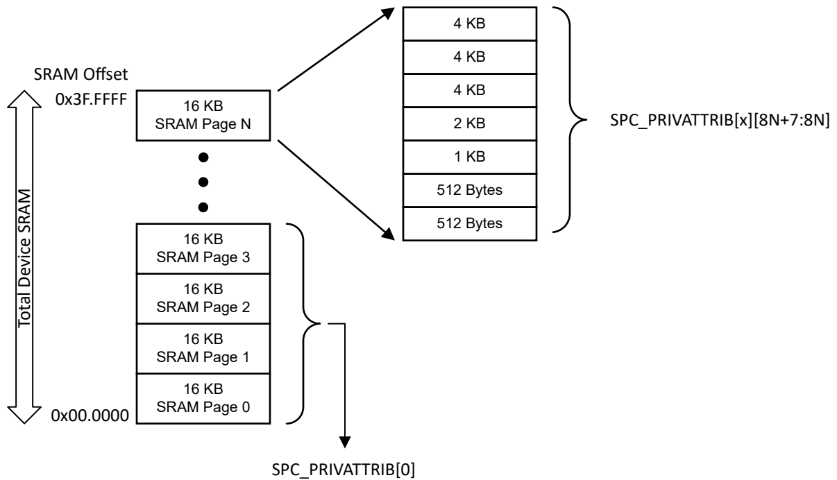
Figure 15-2. SRAM Page and Chunk Mapping
