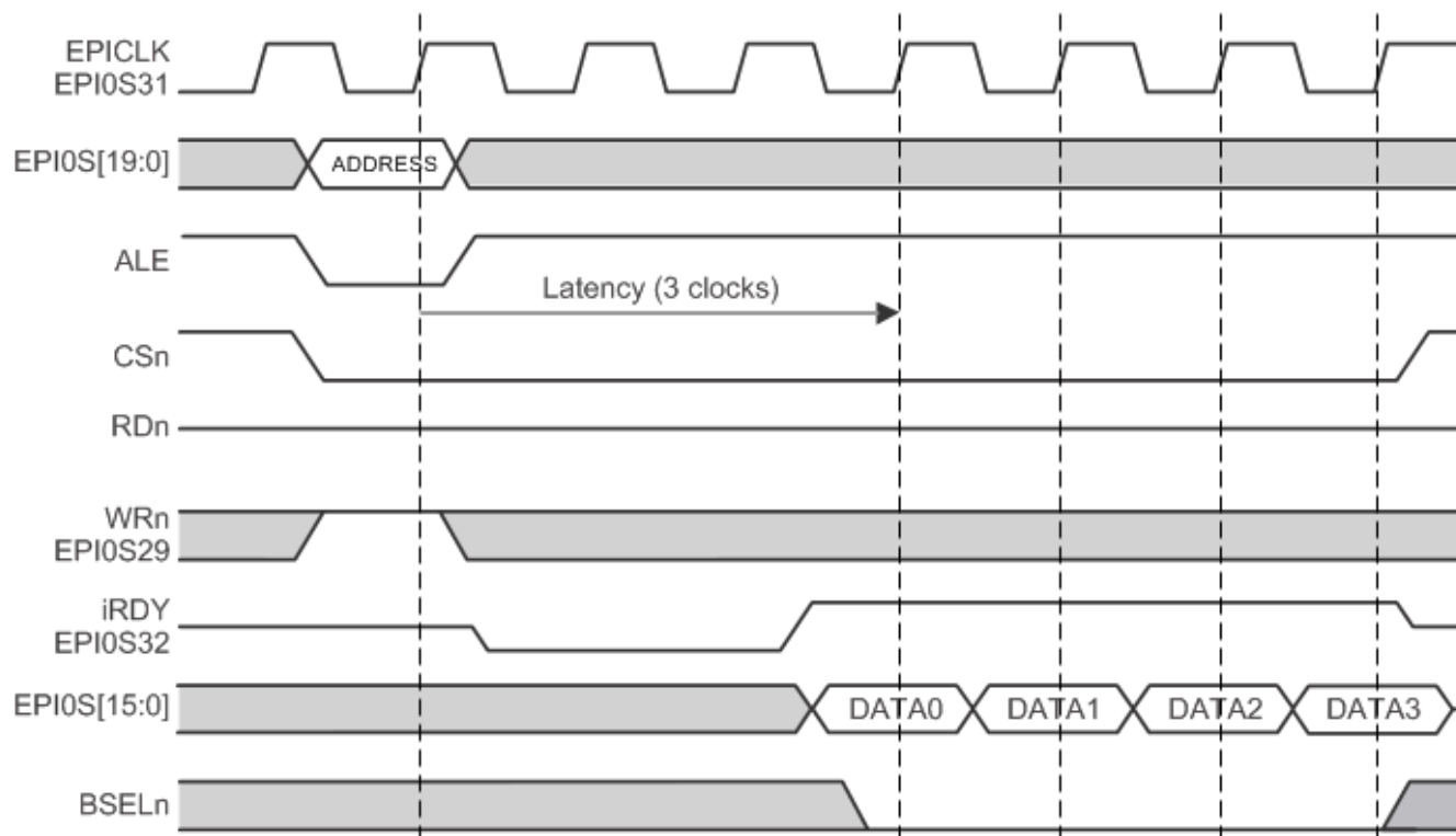
Figure 16-7. PSRAM Burst Read
