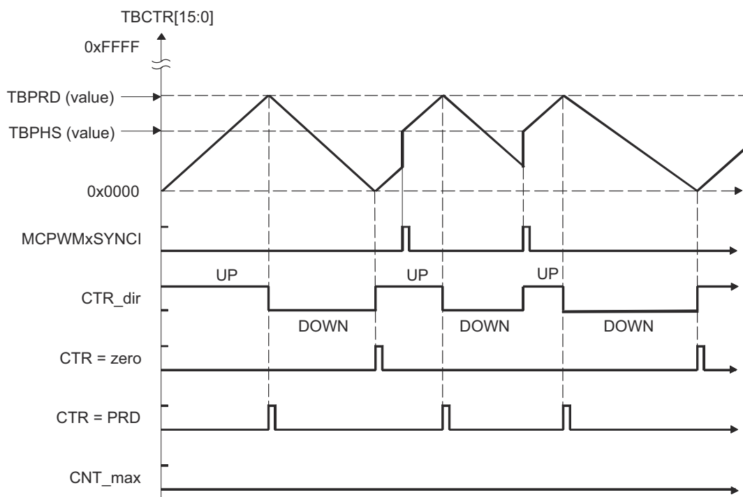
Figure 26-10. Time-Base Up-Down Count Waveforms, TBCTL[PHSDIR = 1] Count Up On Synchronization Event
