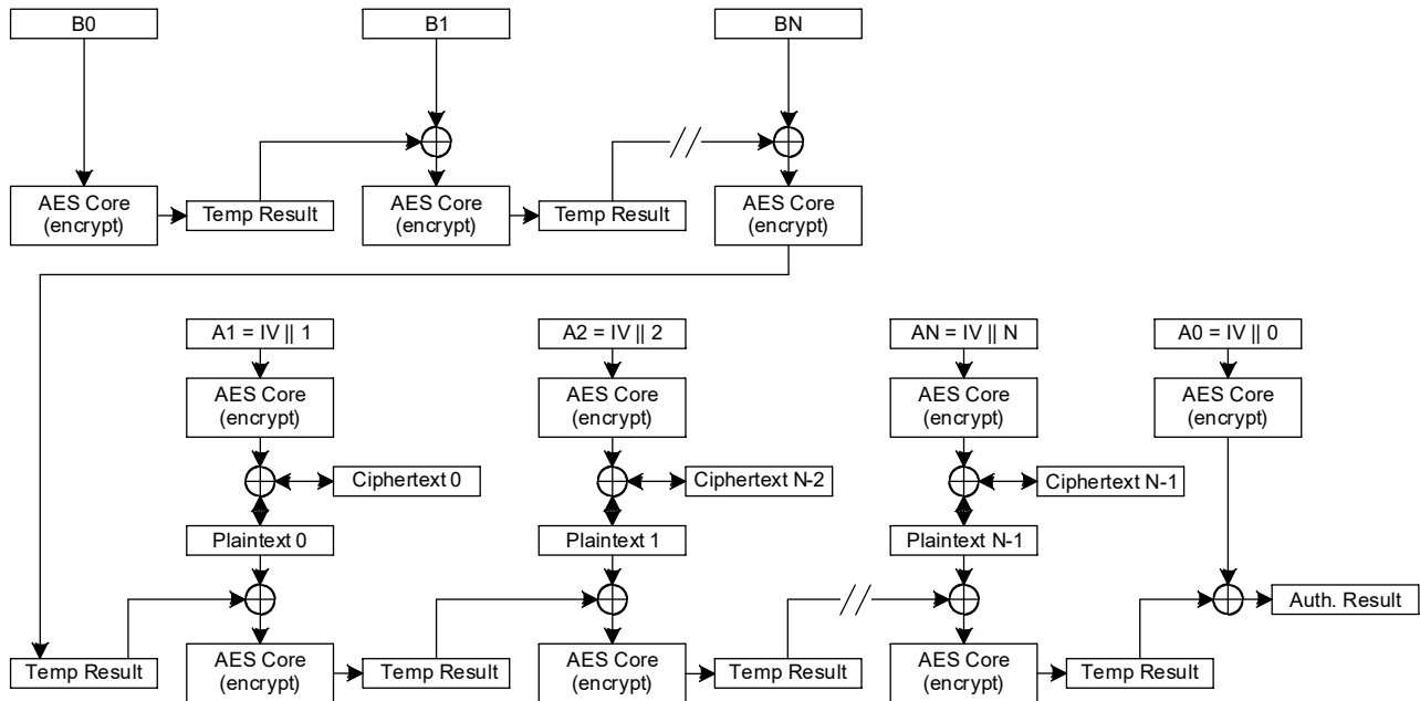
Figure 8-9. CCM Protocol Operation
