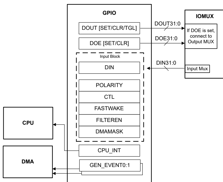
Figure 14-1. GPIO Block Diagram
