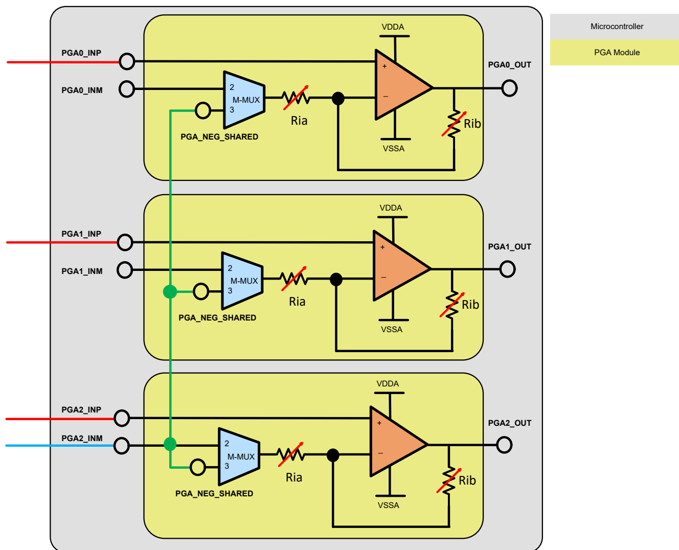
Figure 23-12. Sharing PGA_NEG Pin Between PGA Modules
