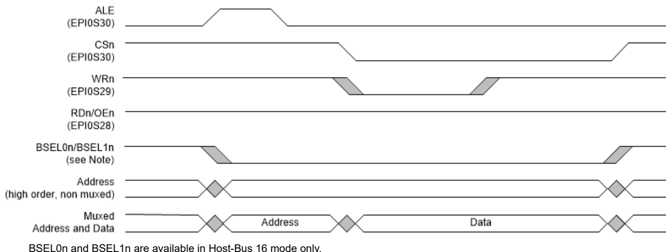
Figure 16-14. Host-Bus Write Cycle with Multiplexed Address and Data, MODE = 0x0, WRHIGH = 0, RDHIGH = 0
