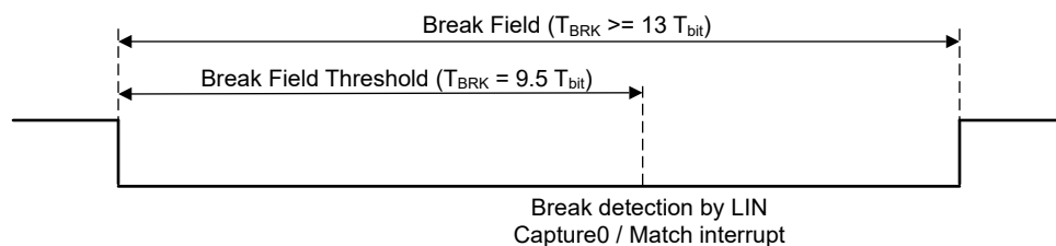
Figure 29-7. LIN Break Field Detection
