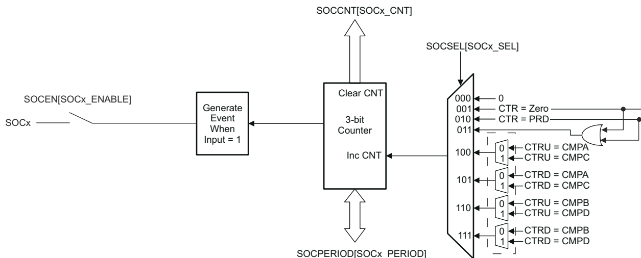
Figure 26-37. Event-Trigger Start-of-Conversion (SOC) Pulse Generator
