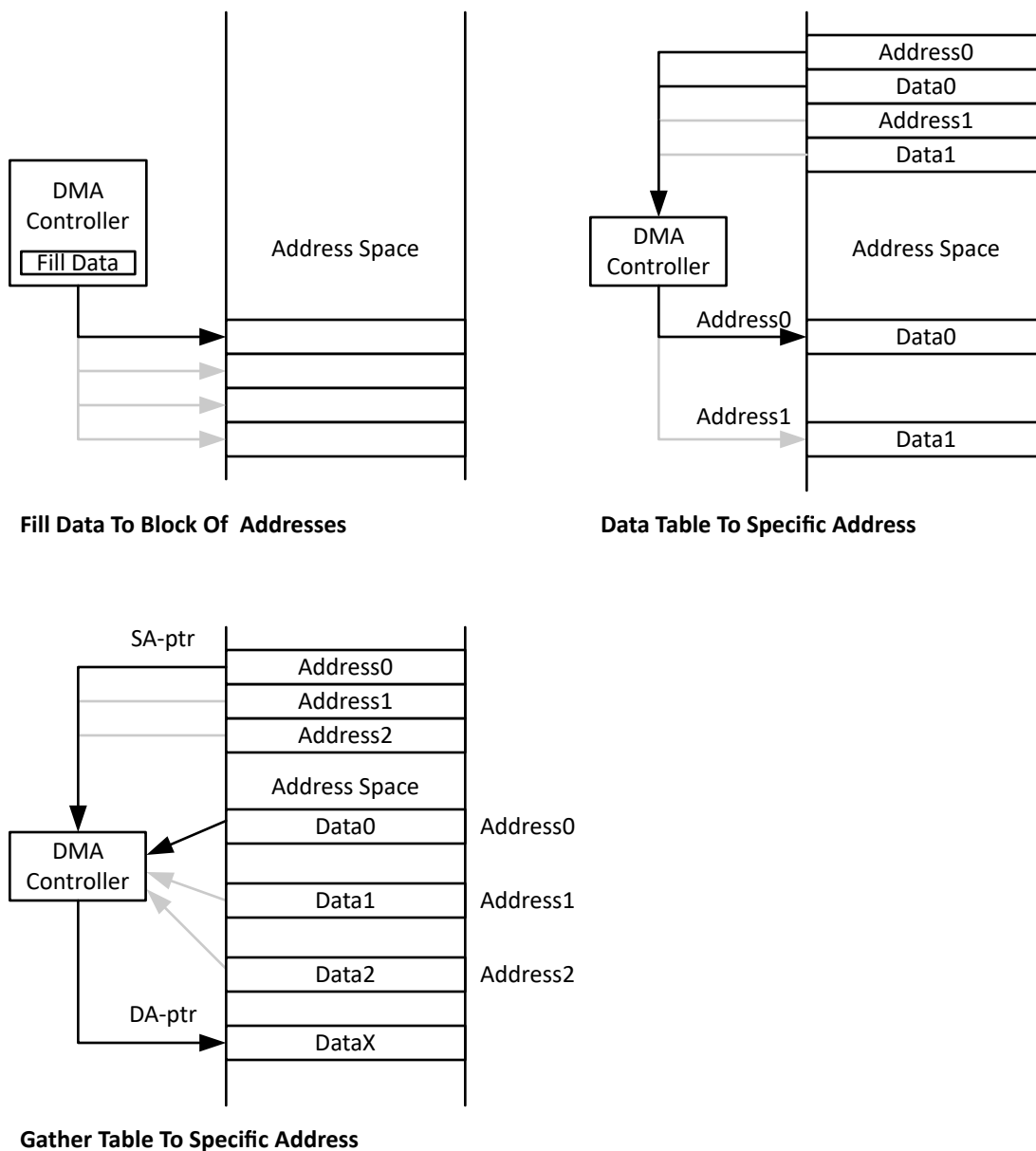
Figure 11-4. DMA Extended Modes Diagram
