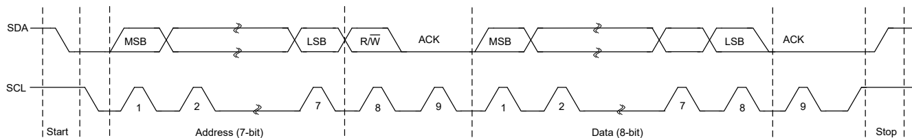
Figure 30-3. Module Data Transfer
