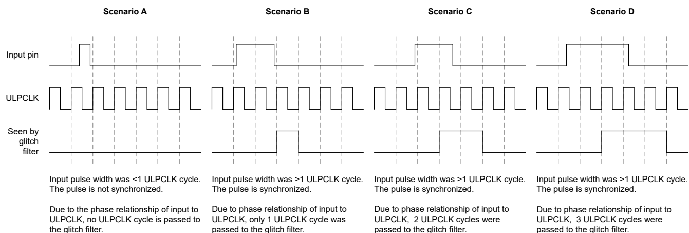
Figure 14-3. GPIO Input Synchronizer and Glitch Filtering Scenarios
