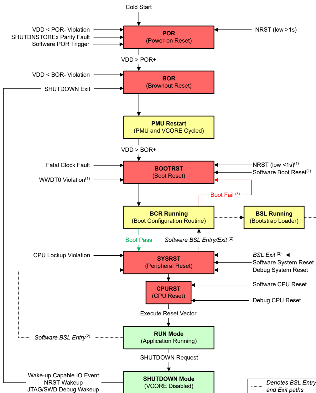
Figure 3-10. Device Reset Levels
