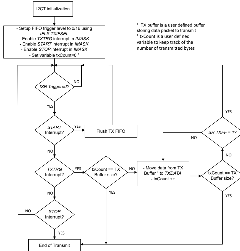
Figure 30-19. Target Transmitter Mode using TXTRG
