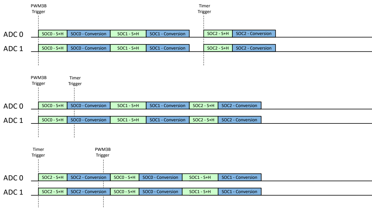
Figure 21-14. Example: Synchronous Operation with Multiple Trigger Sources
