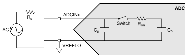
Figure 21-6. Single-Ended Input Model
