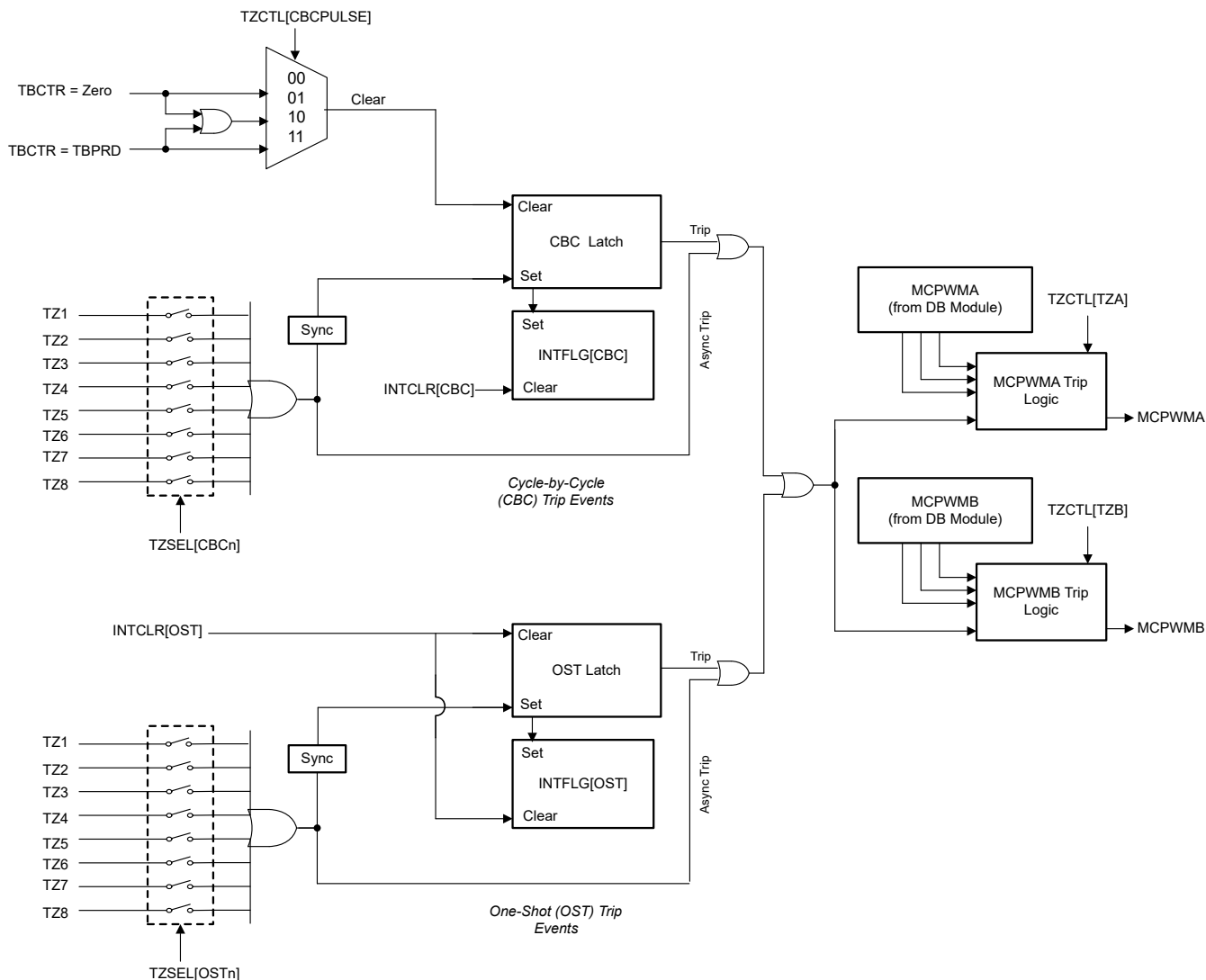
Figure 26-33. Trip-Zone Submodule Mode Control Logic
