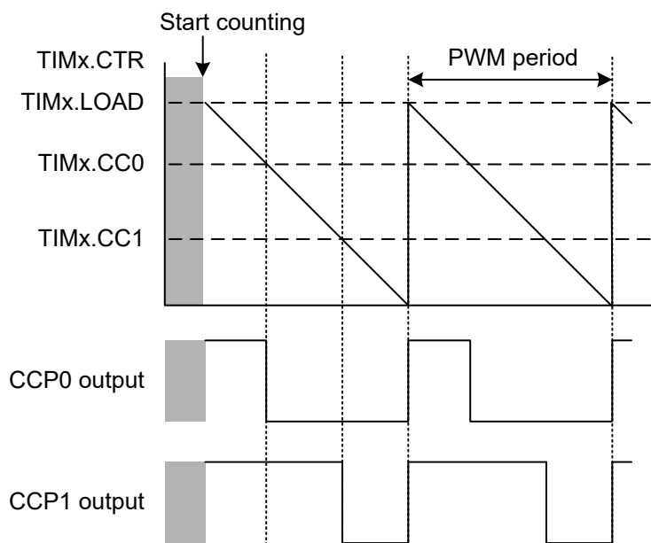
Figure 18-19. Edge-Aligned PWM Signals in Down-Counting Mode
