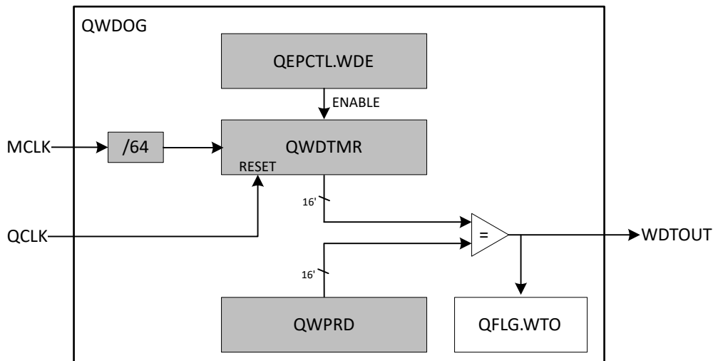
Figure 25-20. eQEP Watchdog Timer
