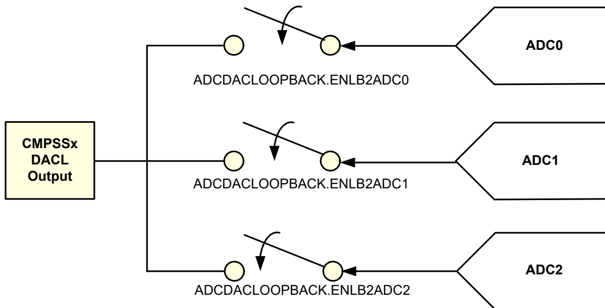
Figure 21-19. CMPSS to ADC Loopback Connection
