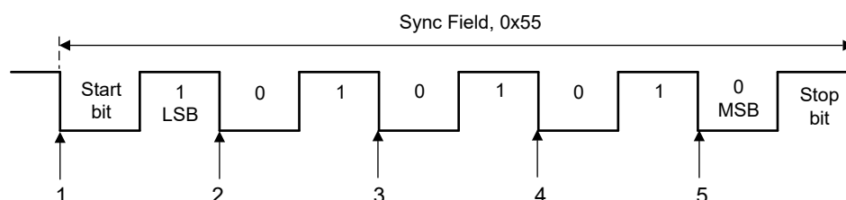
Figure 29-8. LIN Sync Field Detection
