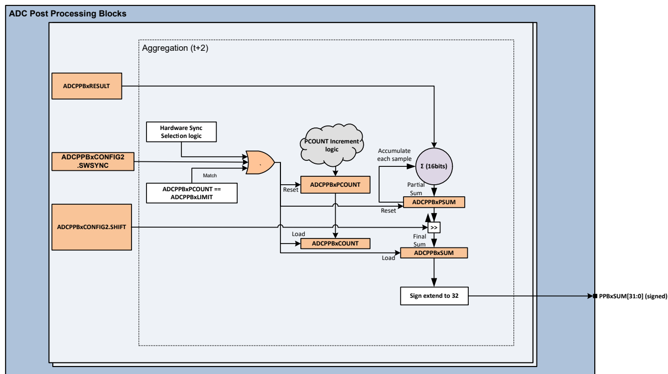
Figure 21-8. ADC Post-Processing Blocks (PPB) Block Diagram
