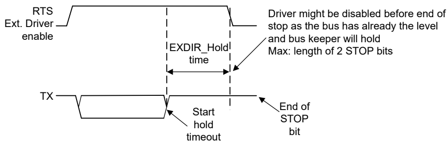
Figure 29-12. RS485 external driver control
