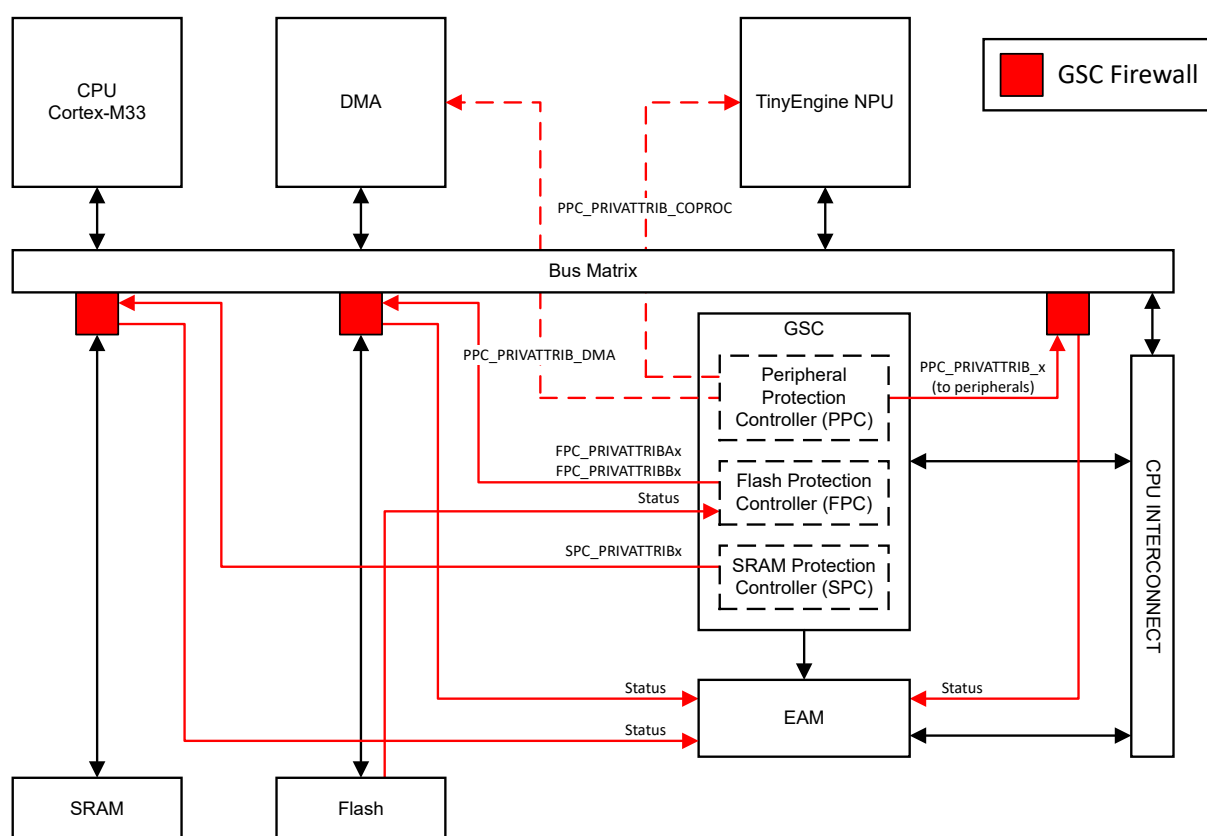
Figure 15-1. GSC Functional Block Diagram
