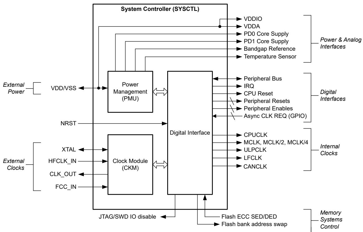
Figure 3-1. Sysctl Top-Level Diagram
