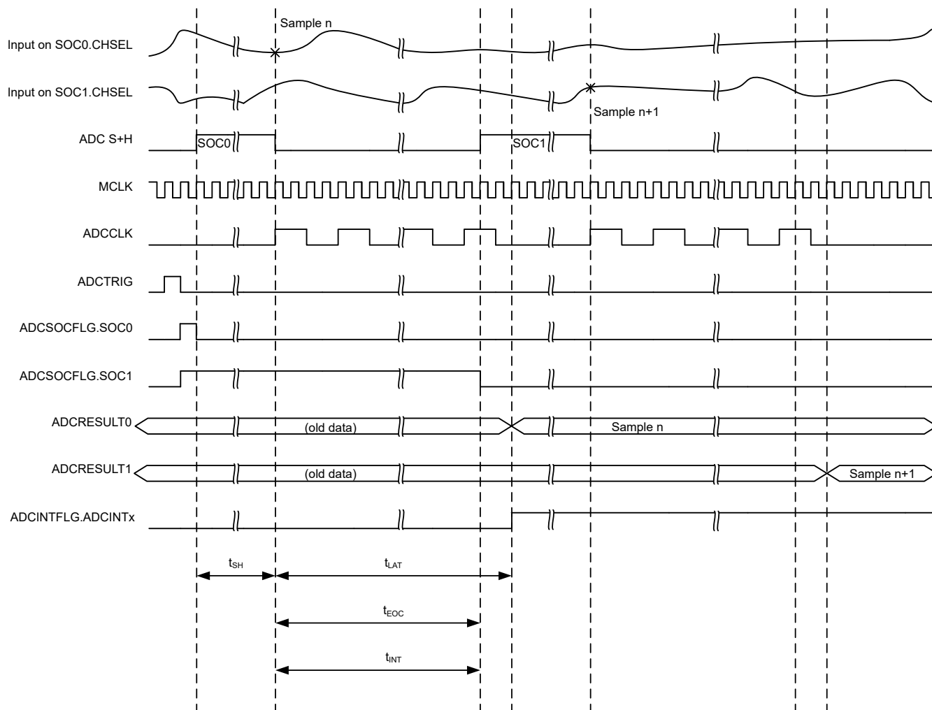
Figure 21-11. ADC Timings for 12-bit Mode in Early Interrupt Mode
