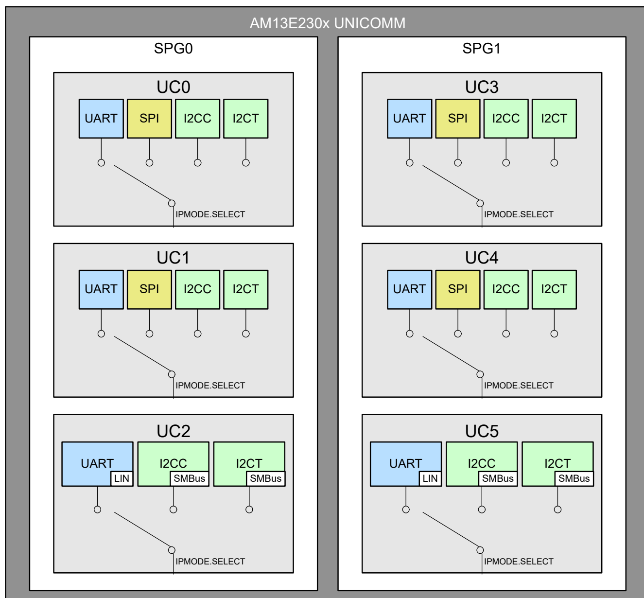
Figure 28-1. Unicommm Block Diagram
