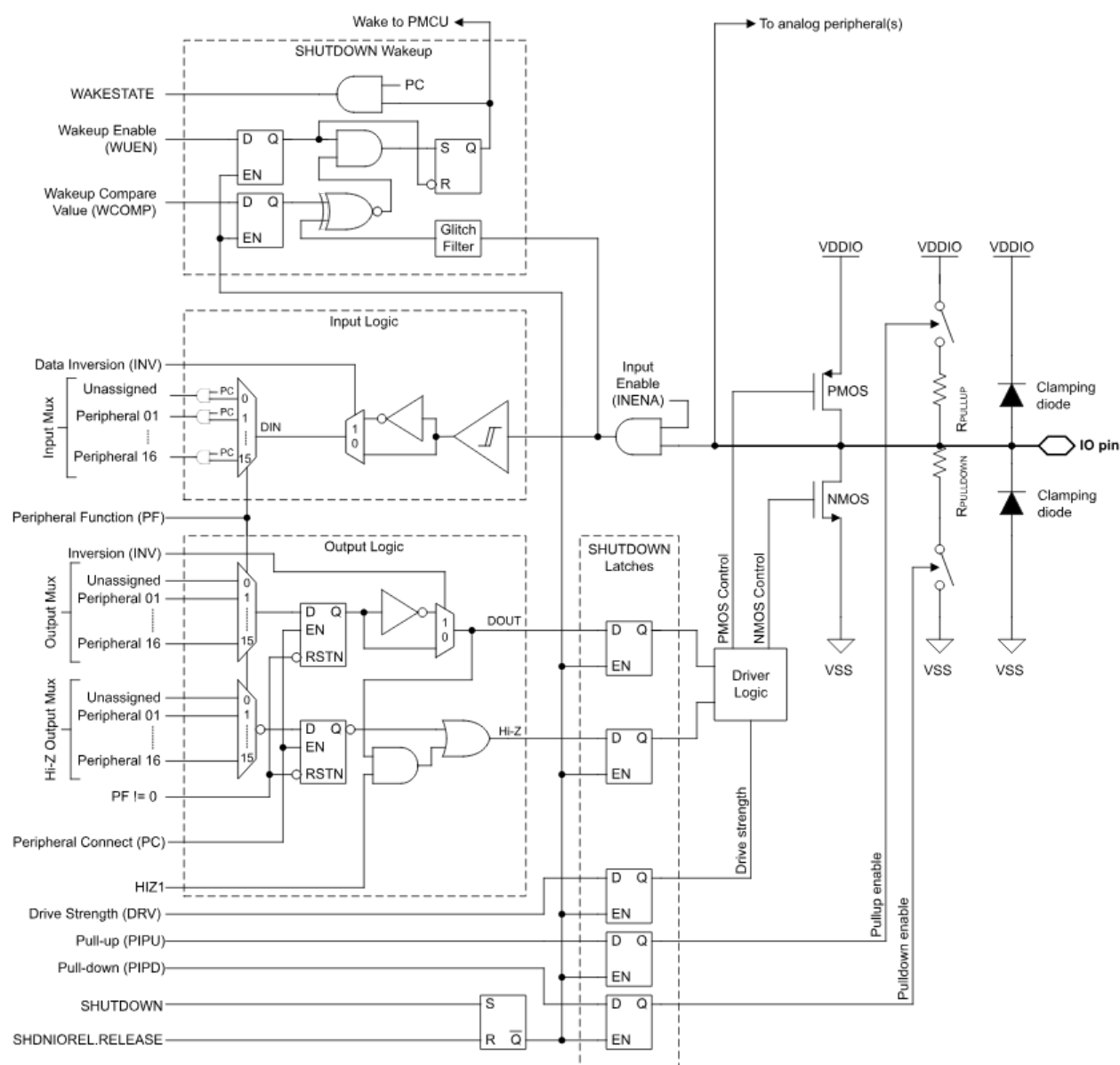
Figure 17-1. Superset IO Slice
