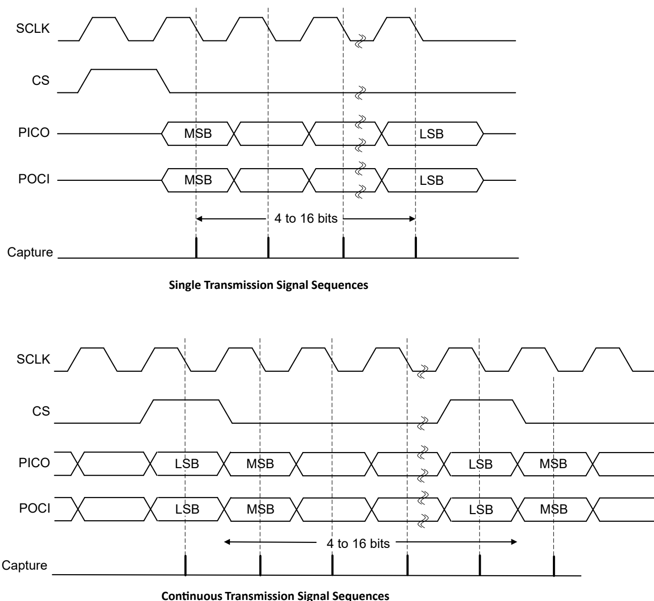
Figure 31-7. TI Synchronous Serial Frame Format
