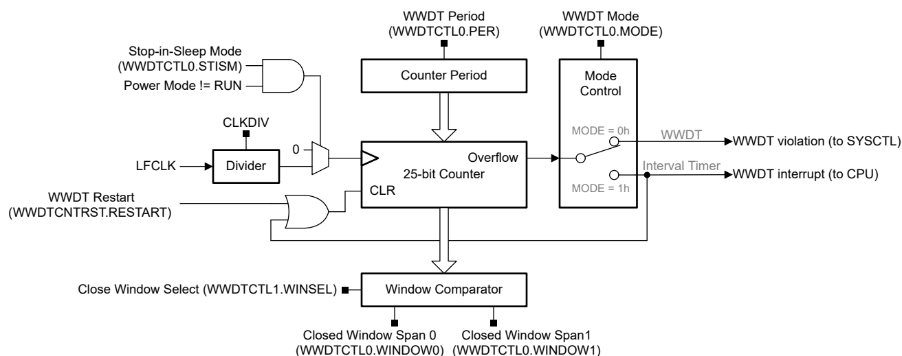
Figure 19-2. WWDT Diagram
