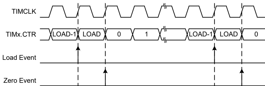
Figure 18-8. Up Counting Mode Event Generation
