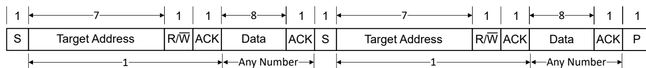
Figure 30-8. Data Format with Repeated Start
