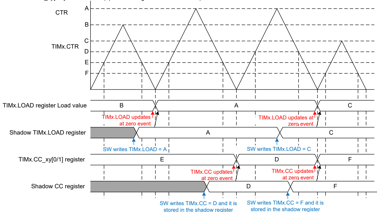
Figure 18-17. Shadow Load and Shadow Compare Taking Effect at Zero Event in Up/Down Mode
