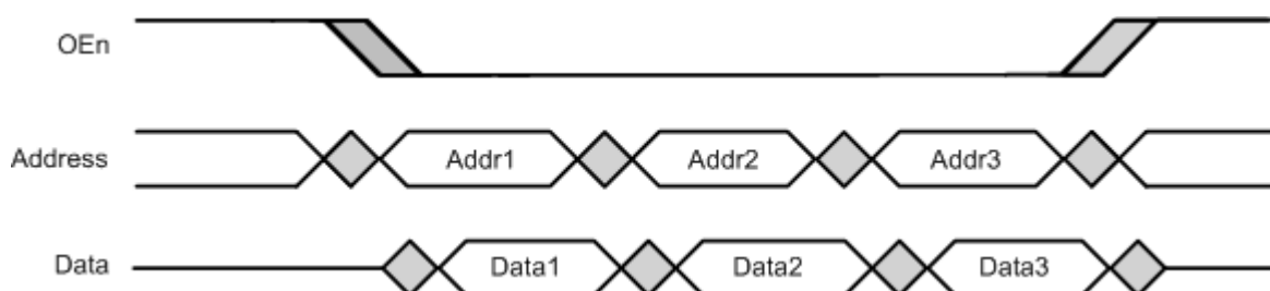
Figure 16-16. Continuous Read Mode Accesses
