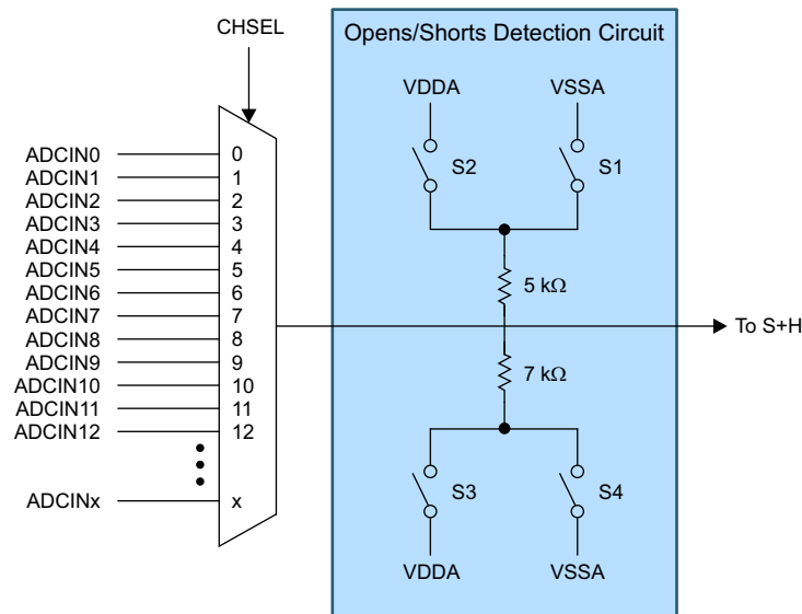
Figure 21-9. Opens/Shorts Detection Circuit
