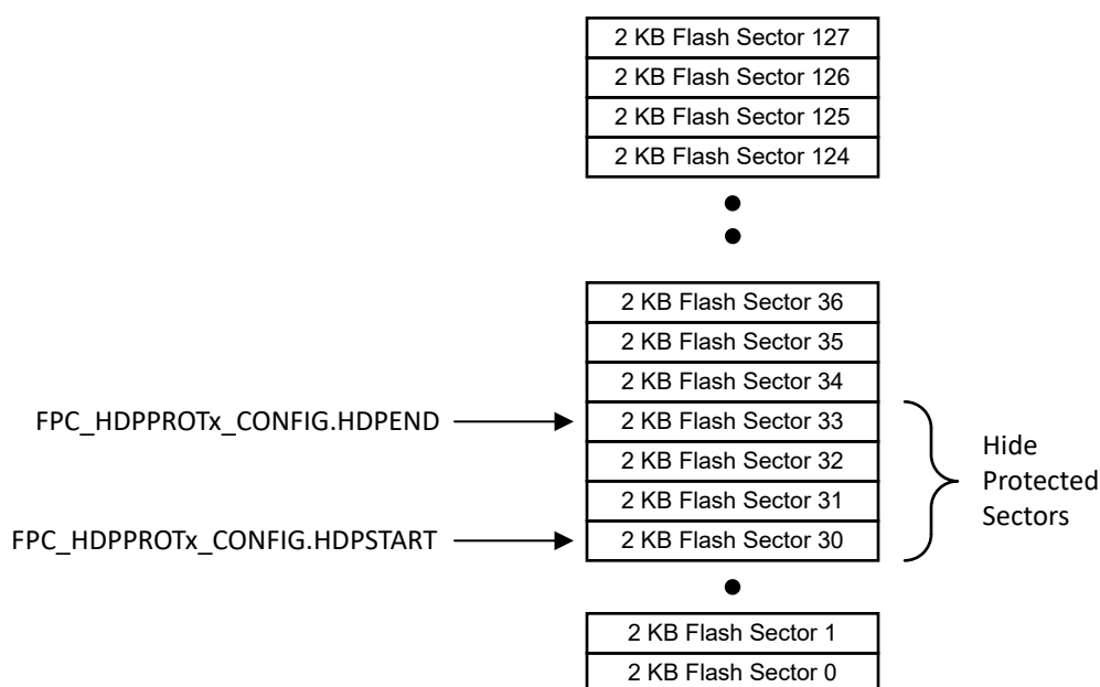
Figure 15-5. Flash Hide Protection Memory View
