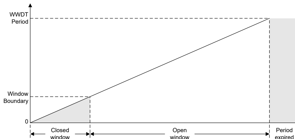
Figure 19-1. WWDT Functionality
