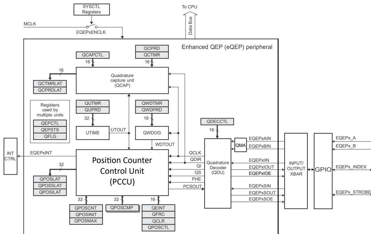
Figure 25-5. Functional Block Diagram of the eQEP Peripheral
