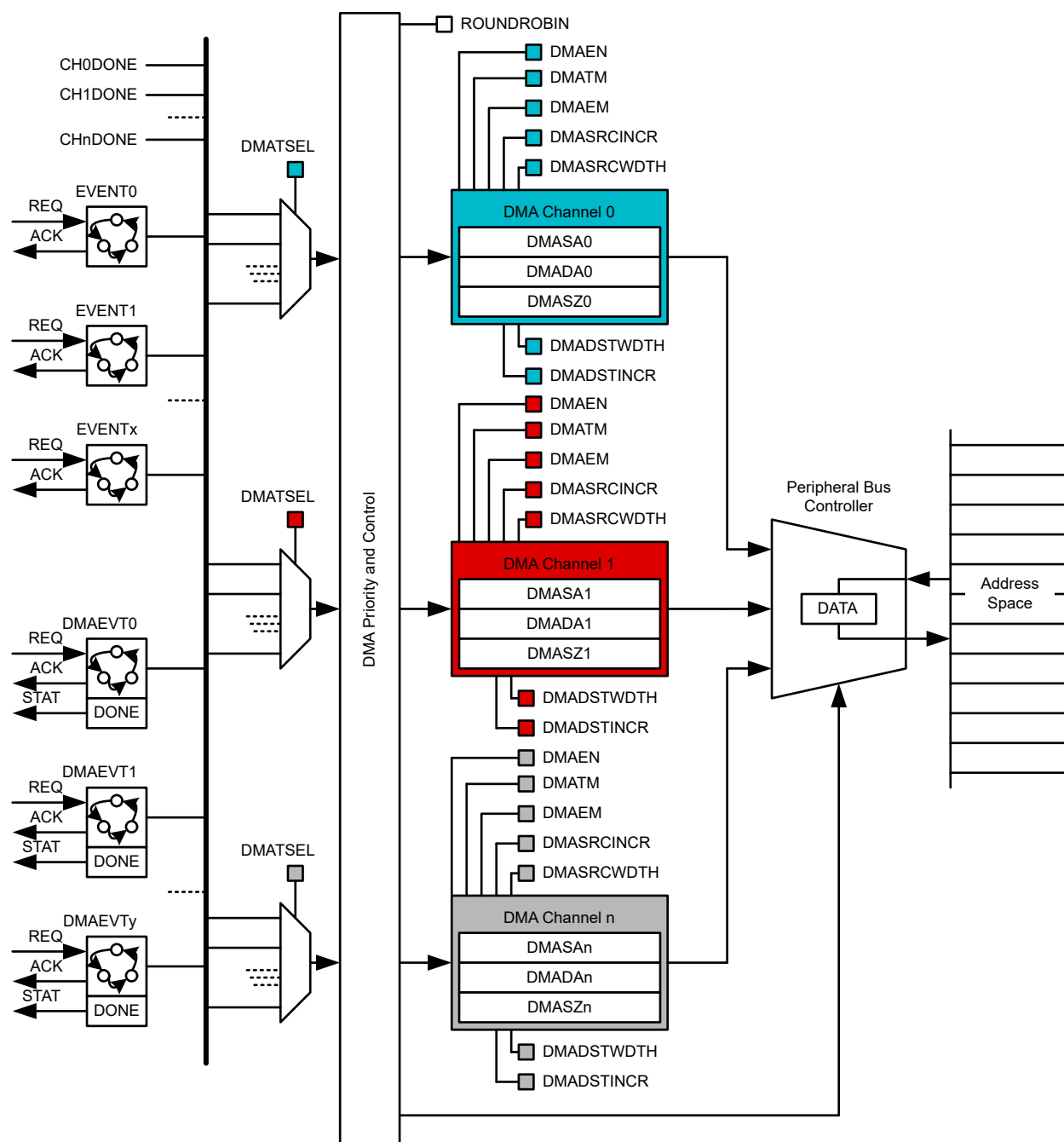
Figure 11-1. DMA Block Diagram
