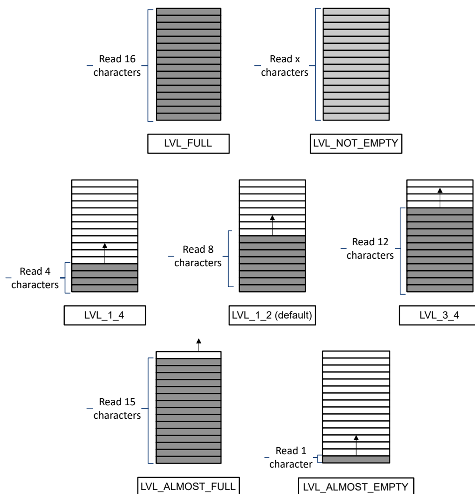
Figure 28-3. UNICOMM Receive FIFO Levels
