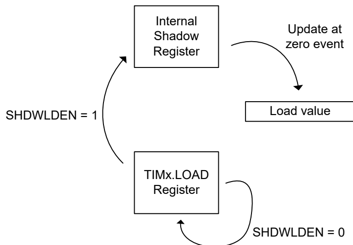
Figure 18-16. Load value updates for TIMx instances when EN=1
