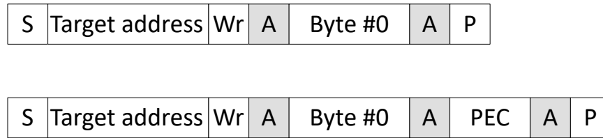
Figure 30-12. Send Byte Message with and without PEC
