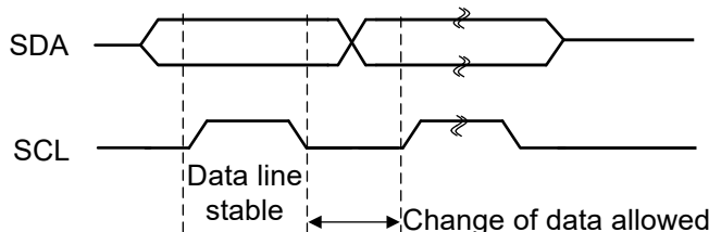
Figure 30-4. Data Change Period
