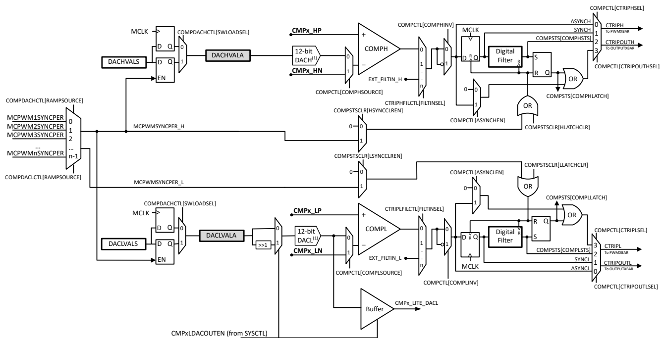
Figure 22-2. CMPSS_LITE Module Block Diagram
