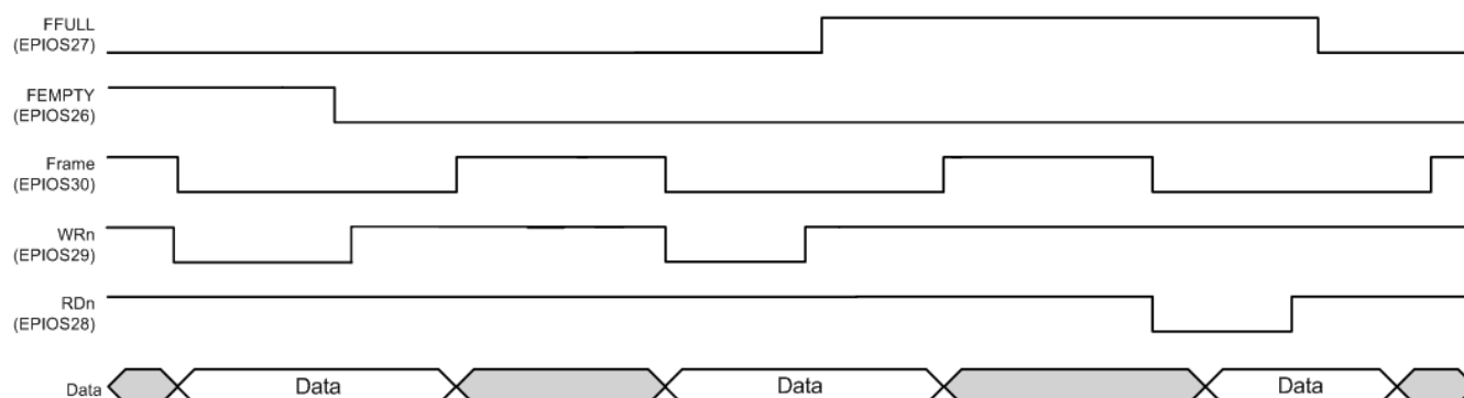
Figure 16-18. Two-Entry FIFO
