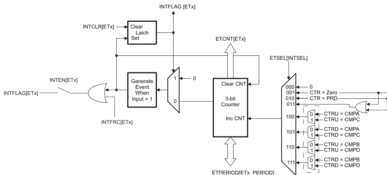
Figure 26-36. Event-Trigger Interrupt Generator
