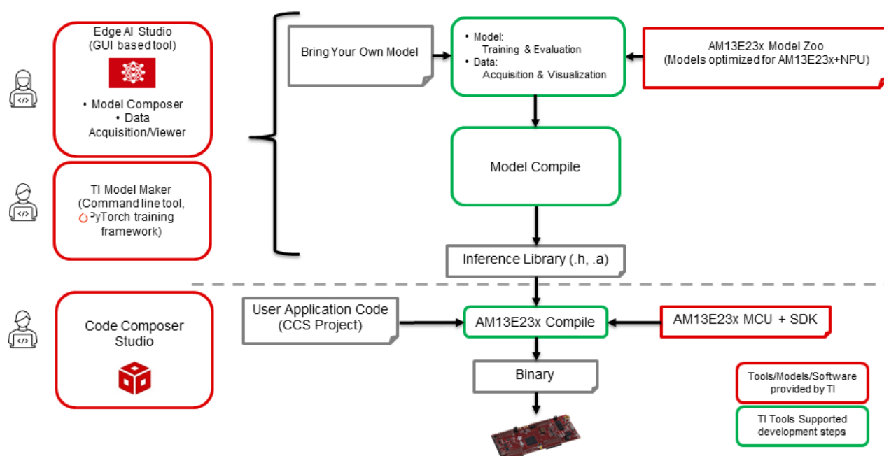
Figure 7-1. TinyEngine™ NPUDevelopment Flow
