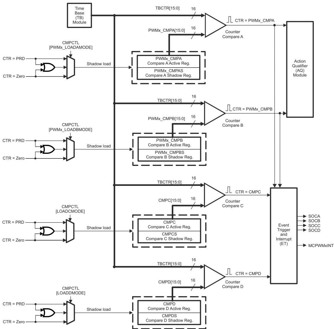
Figure 26-13. Detailed View of the Counter-Compare Submodule
