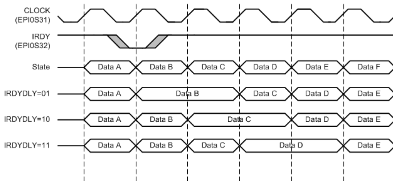
Figure 16-5. iRDY Access Stalls, IRDYDLY = 01, 10, 11
