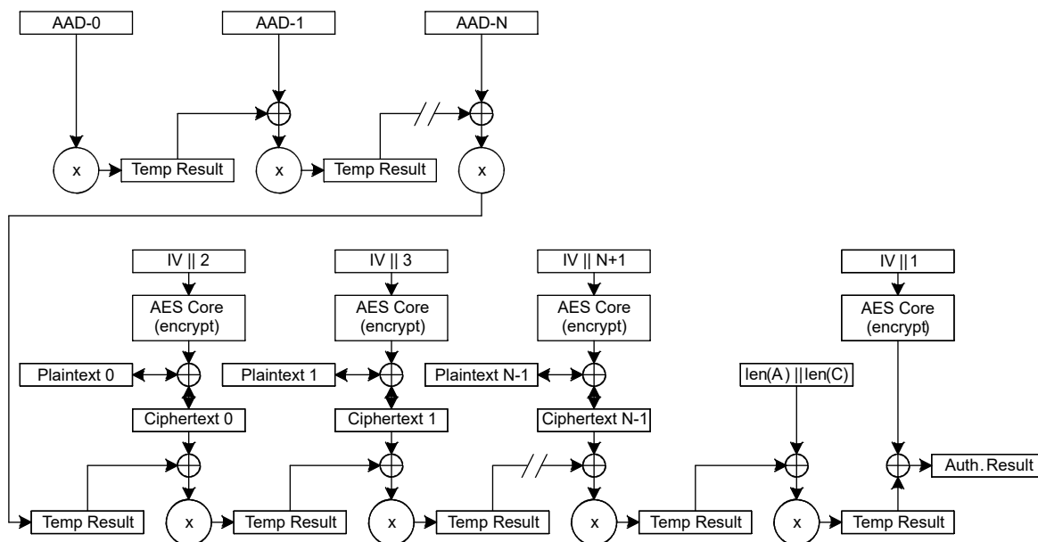
Figure 8-7. GCM Protocol Operation
