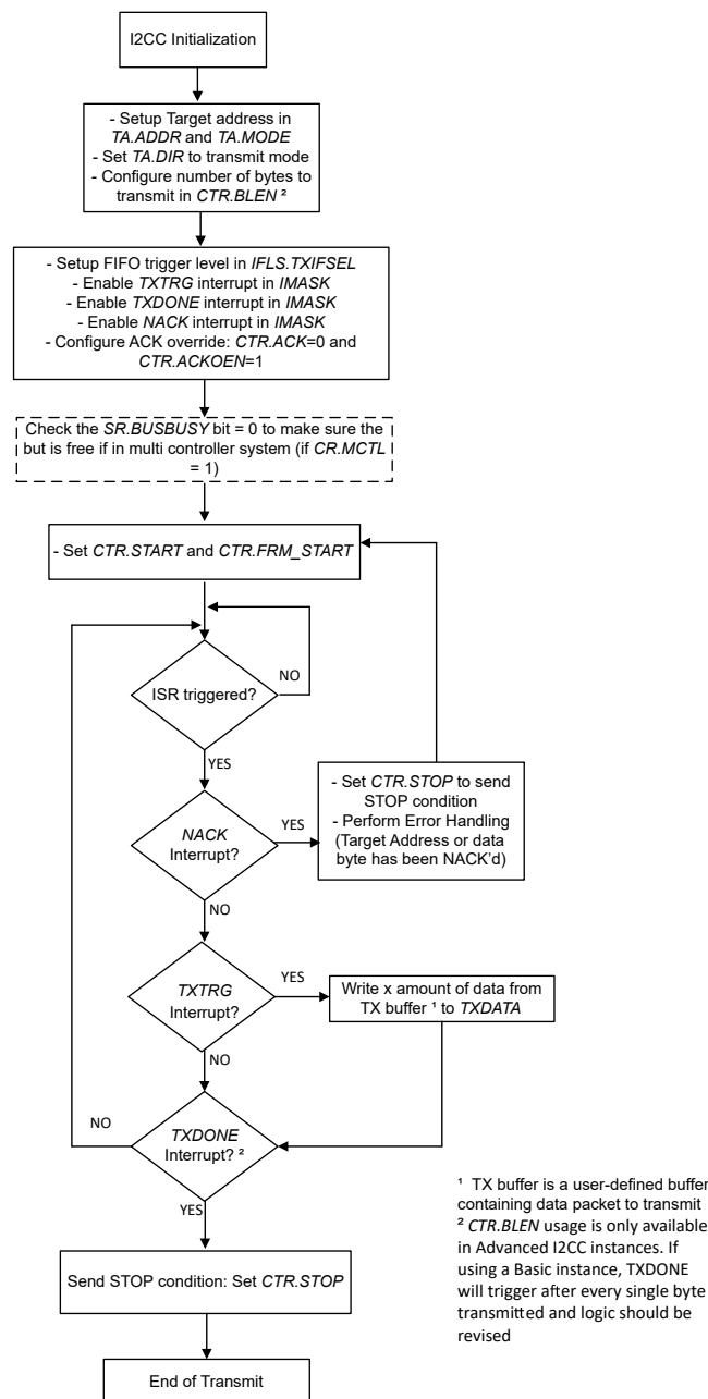
Figure 30-15. Controller Transmitter Mode
