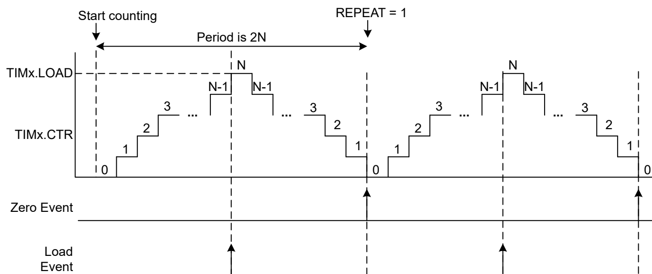
Figure 18-6. Up-down Counting Mode and Event Generation, CVAE = 2
