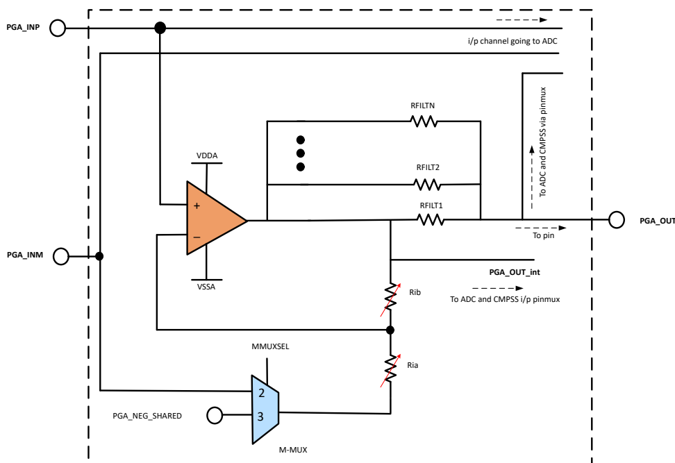
Figure 23-5. Subtractor Mode
