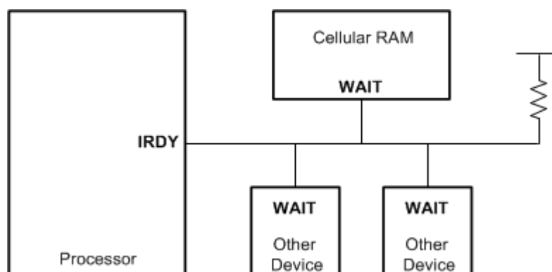
Figure 16-6. iRDY Signal Connection
