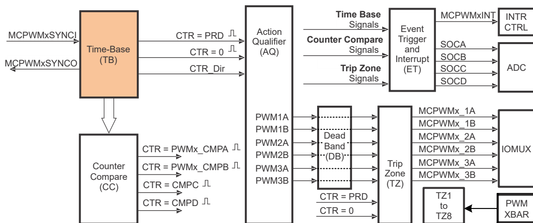
Figure 26-3. Time-Base Submodule
