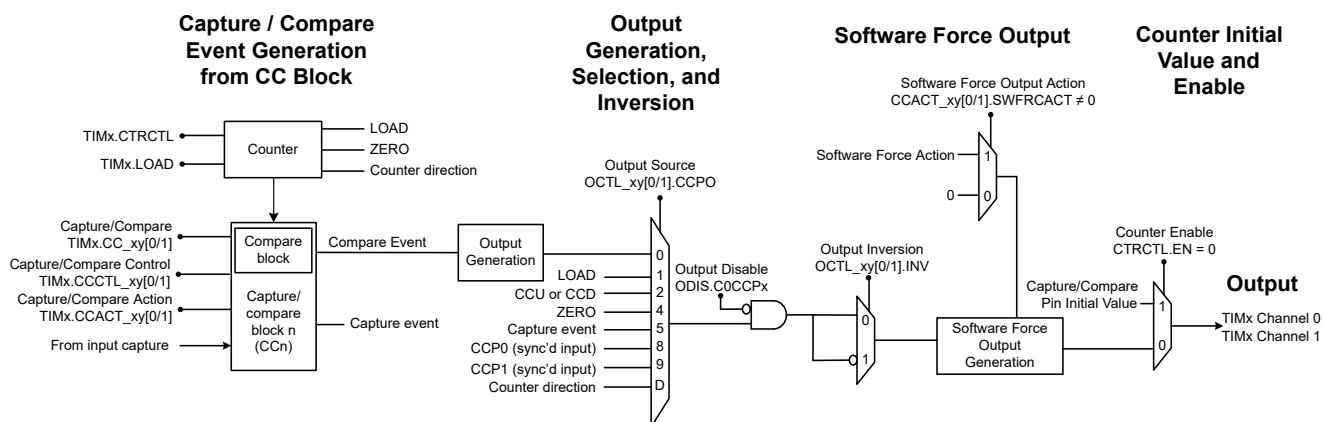
Figure 18-18. Output Connection for TIMx
