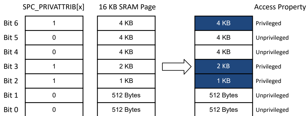
Figure 15-3. SRAM Page Use Example
