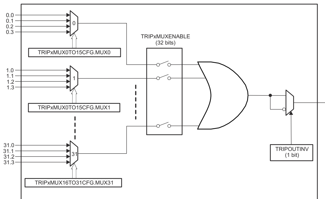
Figure 20-3. MCPWM X-BAR Architecture - Single Output
