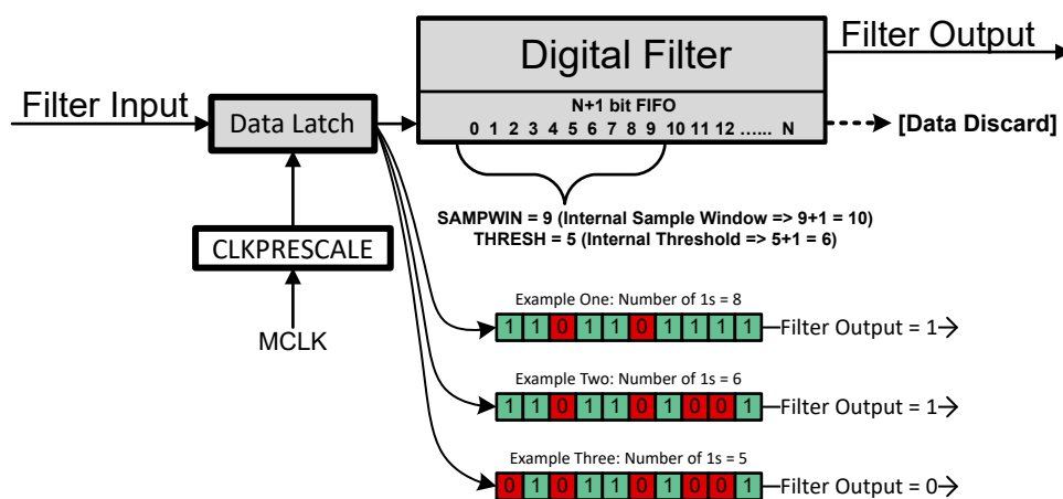
Figure 22-5. Digital Filter Behavior
