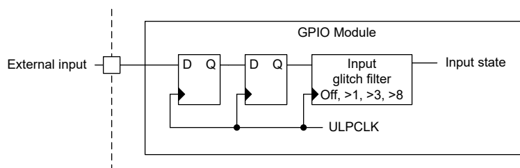
Figure 14-2. GPIO Input Synchronizer
