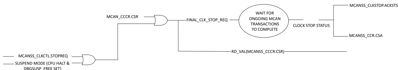
Figure 27-8. Clock Stop Request
