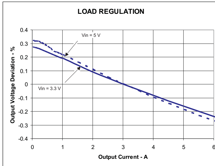
Figure 3. TPS54618EVM-606 Load Regulation
