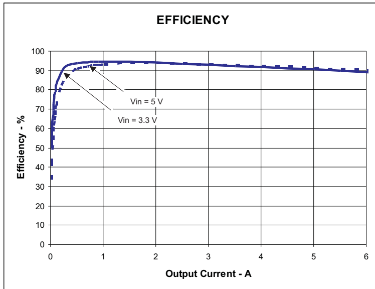
Figure 1. TPS54618EVM-606 Efficiency
