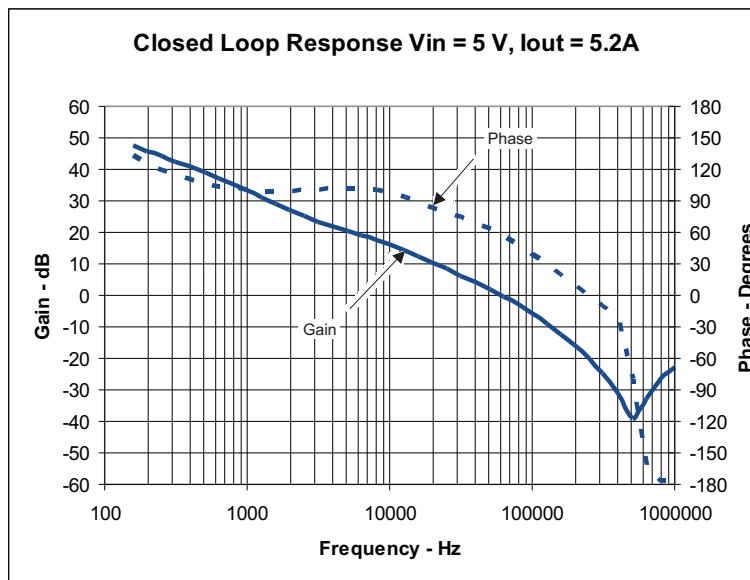
Figure 6. TPS54618EVM-606 Loop Response
