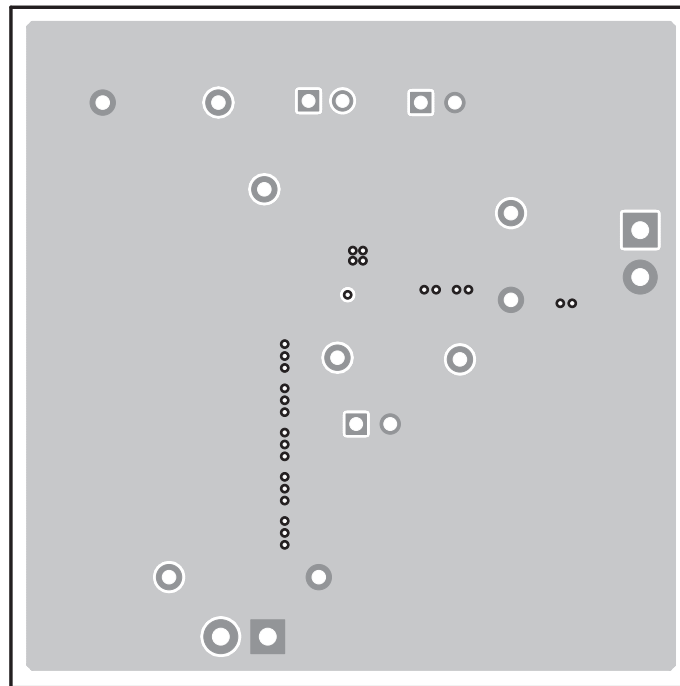
Figure 14. TPS54618EVM-606 Internal Layer 2
