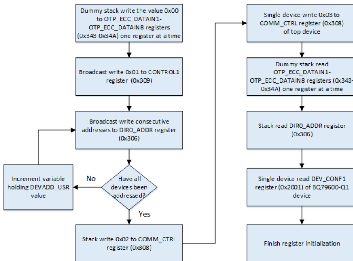
Figure 1-3. Auto-Addressing Flowchart
