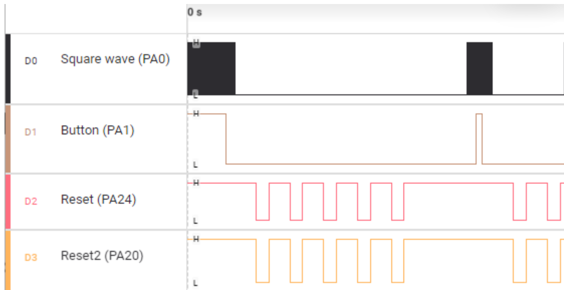
Figure 2-8. SWD Remapped – Laptop_PC_WDT_IC_SWD_Remapped_MSPM0C1103SDSGR_v1
