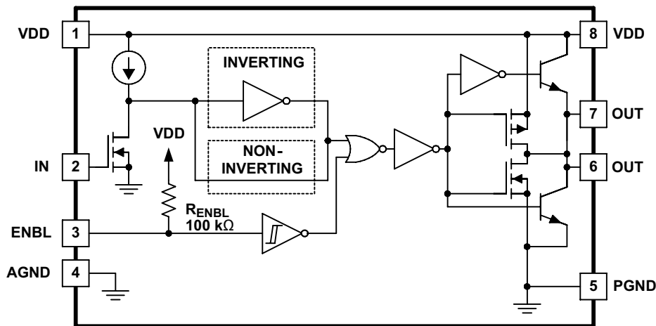
Block Diagram
