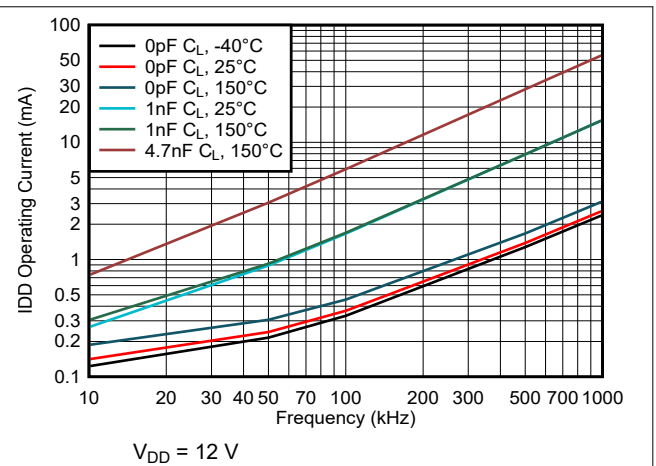
Figure 5-3. IDD Operating Current vs Frequency
