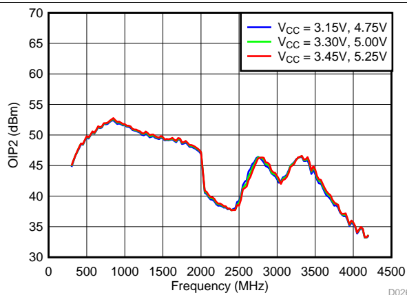
Figure 23. OIP2 vs Supply, High Gain Mode
