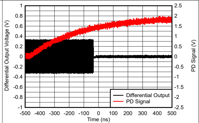
Figure 5-48. Step Response
