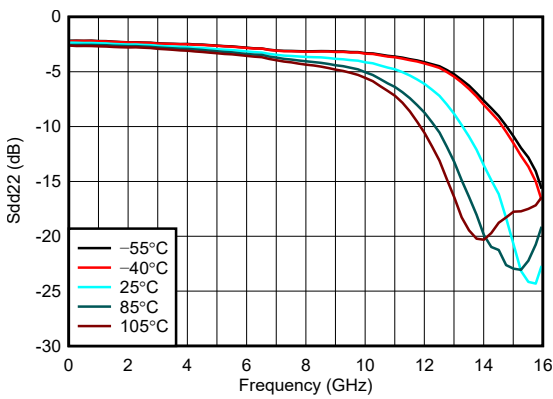
P_{IN} = -20\text{dBm} with 50 \Omega source at all excited ports, nonexcited ports are terminated with 50 \Omega
