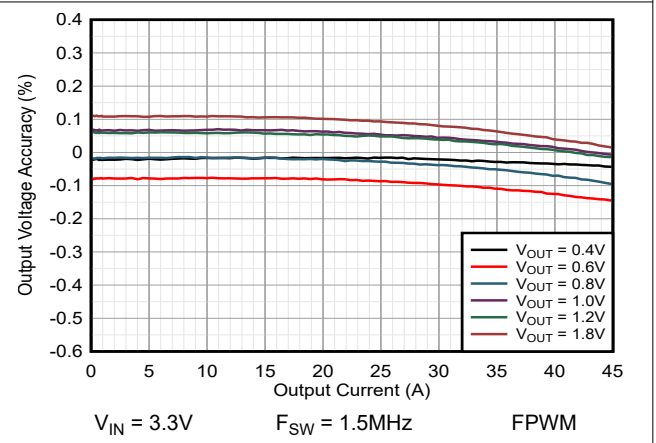
Figure 9-44. Load Regulation
