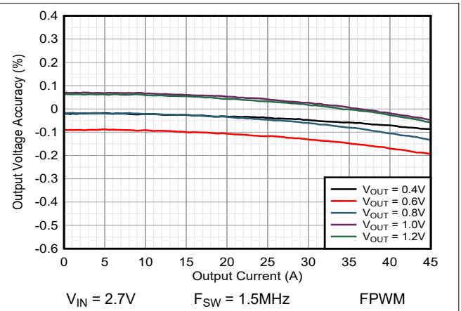
Figure 9-42. Load Regulation
