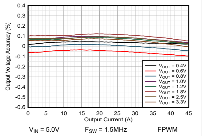
Figure 9-46. Load Regulation
