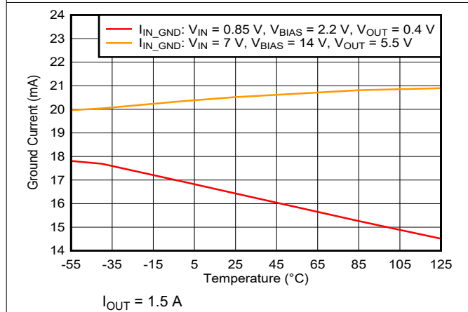
Figure 6-34. Ground Current vs Temperature
