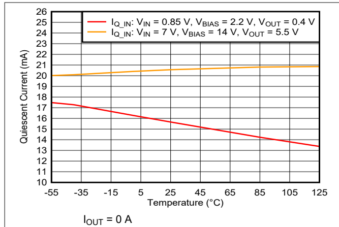
Figure 6-32. Quiescent Current vs Temperature
