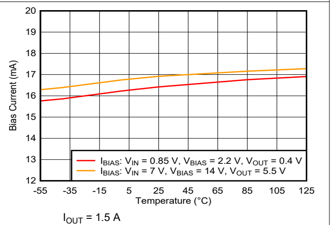
Figure 6-35. Bias Current vs Temperature
