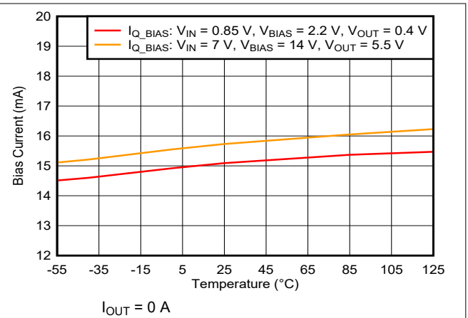
Figure 6-33. Bias Current vs Temperature
