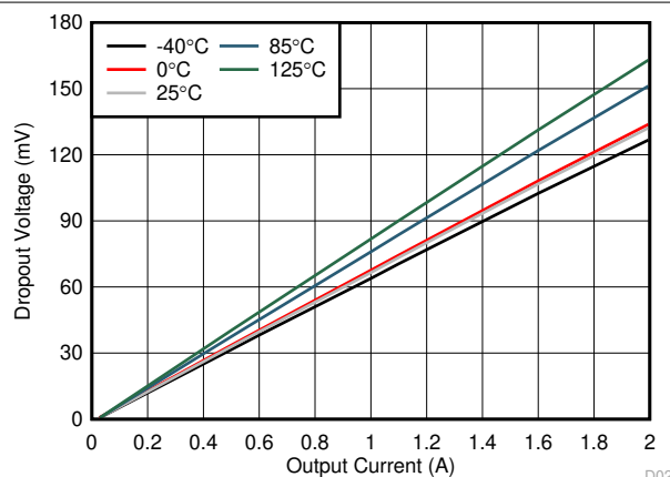
Figure 7-22. Dropout Voltage vs Output Current Without BIAS
