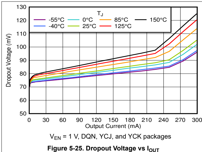
Figure 5-25. Dropout Voltage vs I_{OUT}
