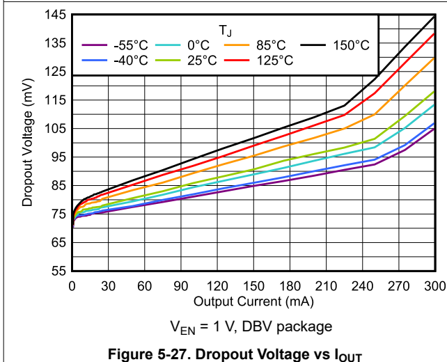
Figure 5-27. Dropout Voltage vs I_{OUT}
