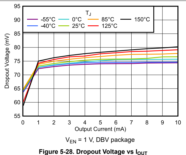
Figure 5-28. Dropout Voltage vs I_{OUT}
