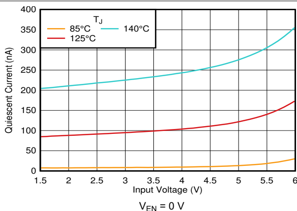
Figure 6-11. I_{SHDN} vs V_{IN} and Temperature
