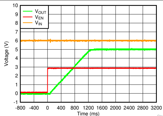
Figure 6-52. Startup With V_{EN} After V_{IN}
