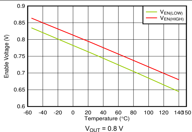
Figure 6-38. EN High and Low Threshold vs Temperature
