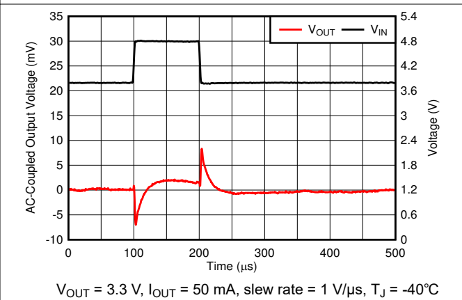
Figure 6-36. Line Transient
