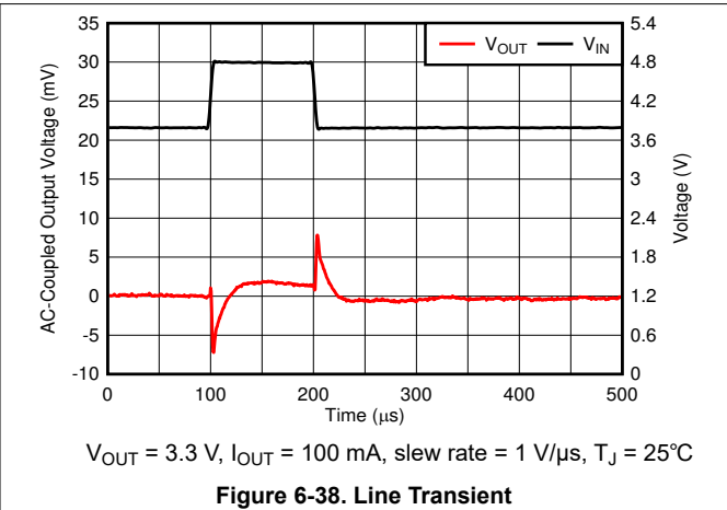
Figure 6-38. Line Transient
