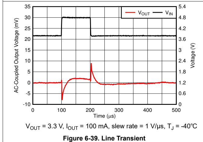
Figure 6-39. Line Transient
