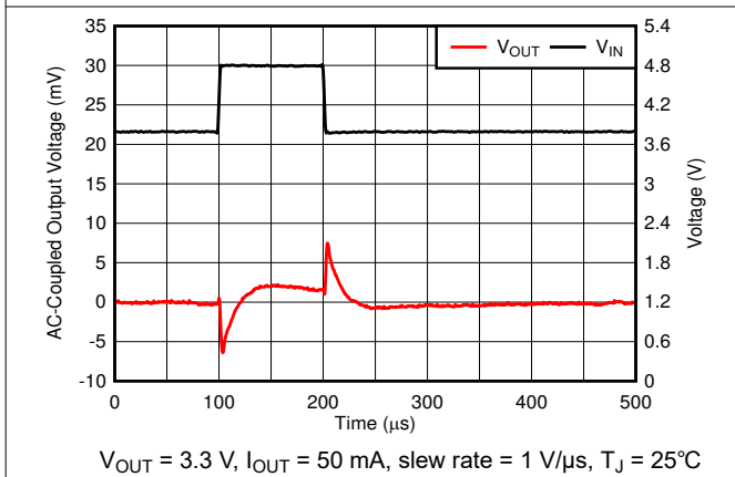
Figure 6-35. Line Transient
