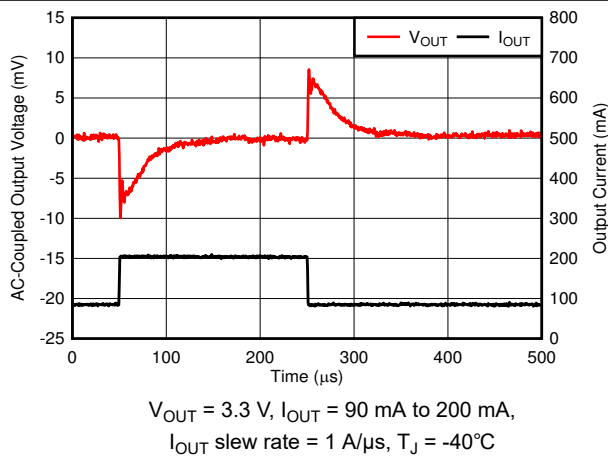
Figure 6-63. Load Transient
