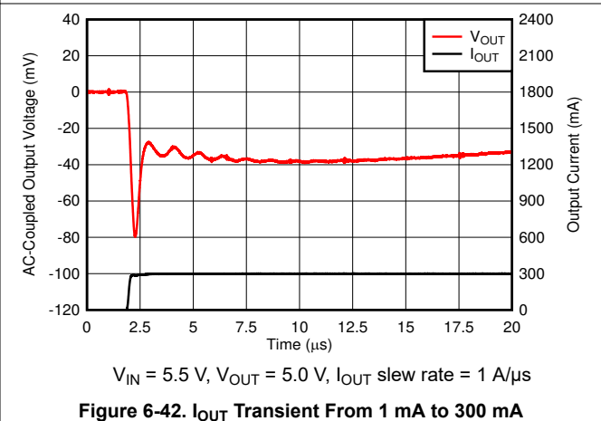
Figure 6-42. I_{OUT} Transient From 1 mA to 300 mA
