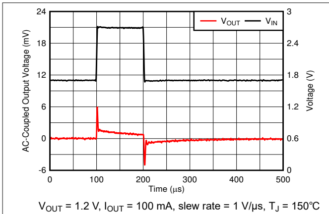
Figure 6-31. Line Transient
