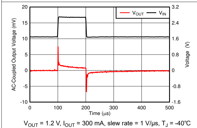
Figure 6-33. Line Transient
