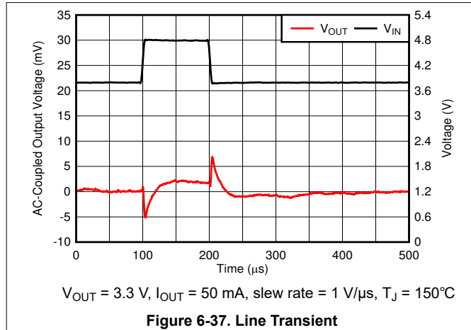
Figure 6-37. Line Transient
