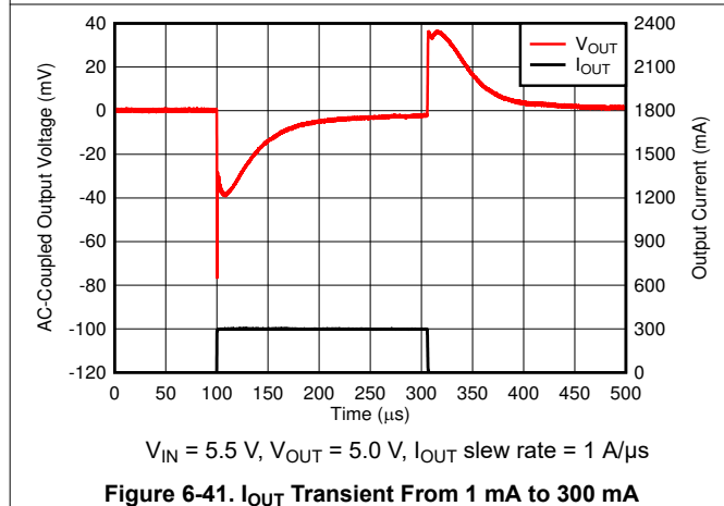
Figure 6-41. I_{OUT} Transient From 1 mA to 300 mA
