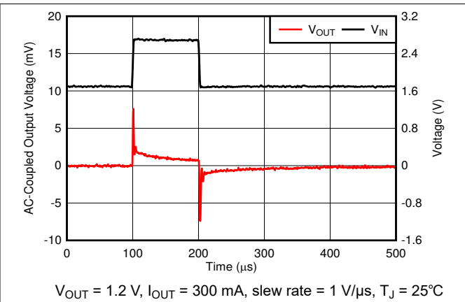
Figure 6-32. Line Transient
