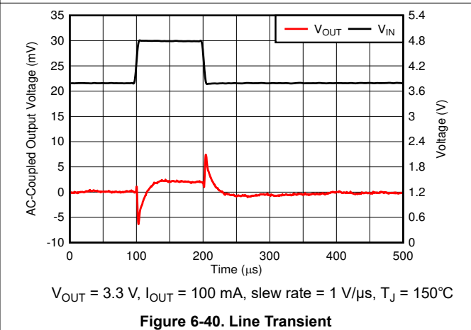
Figure 6-40. Line Transient
