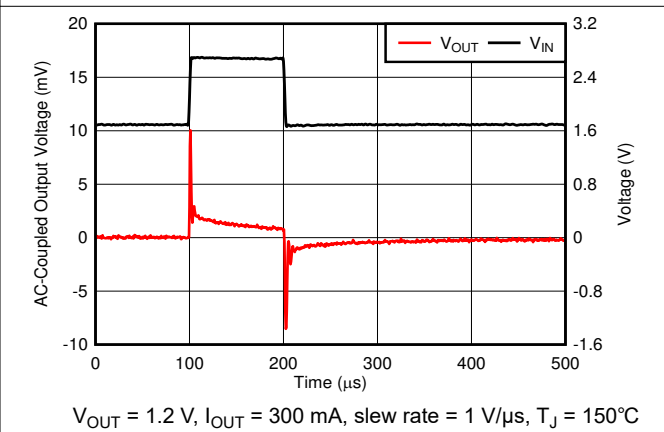
Figure 6-34. Line Transient
