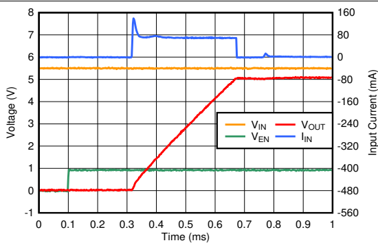
Figure 6-75. Start-Up Inrush Current With C_{OUT} = 1\text{ }\mu\text{F}
