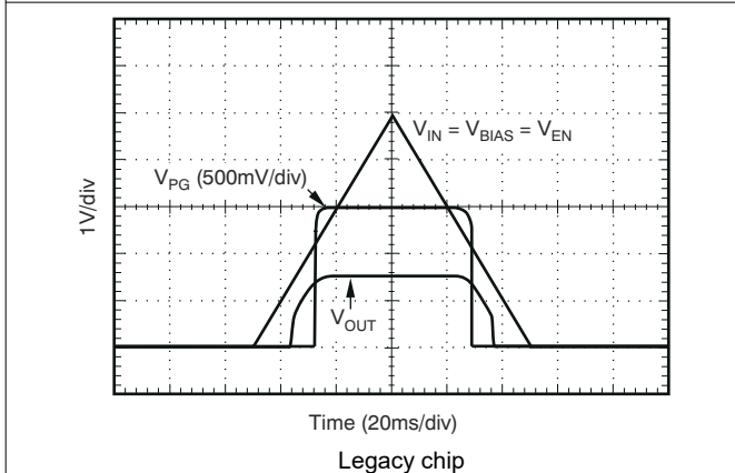
Figure 5-39. Power-Up, Power-Down
