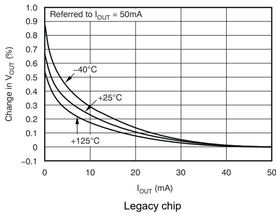
Figure 5-1. Load Regulation
