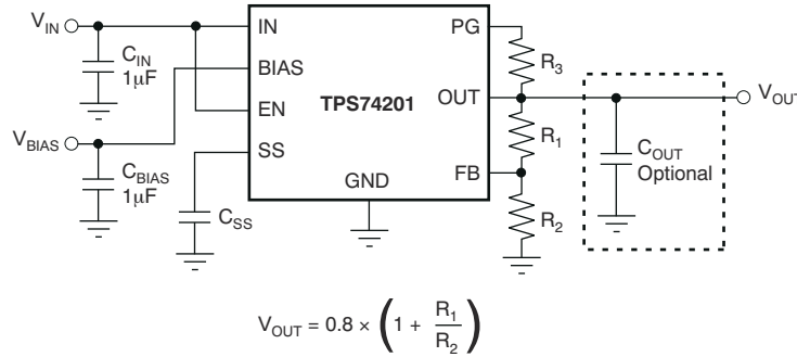
Figure 7-4. Typical Application Circuit for the TPS742
