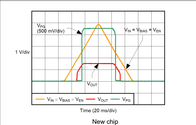
Figure 5-40. Power-Up, Power-Down
