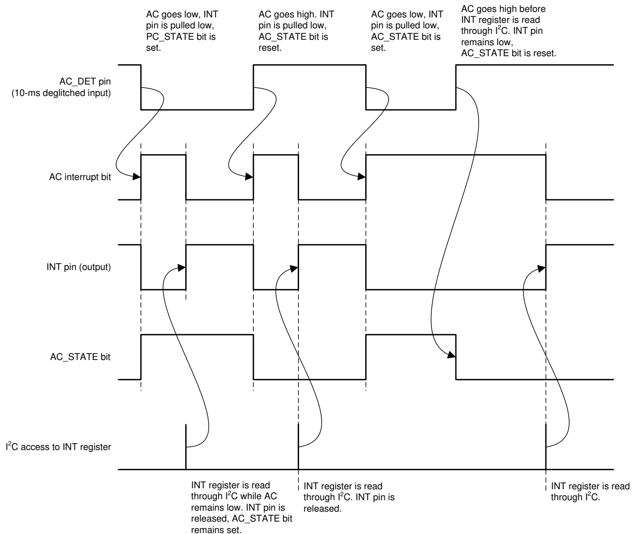
Figure 6-19. AC_STATE Pin
