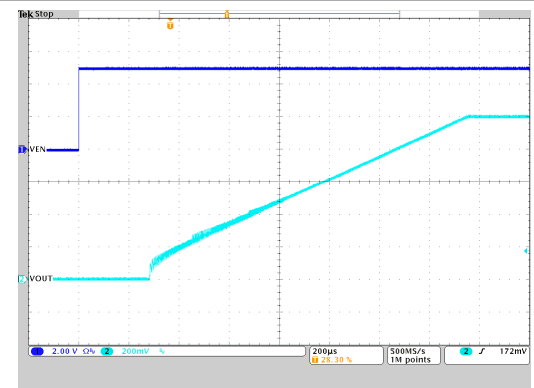
Figure 9-53. Start-Up Timing
