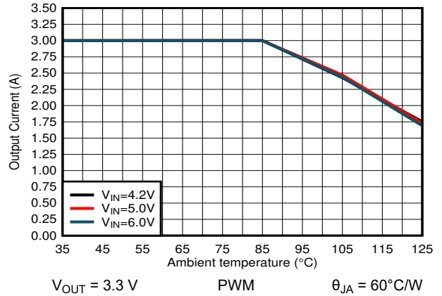
Figure 9-21. Output Current vs Ambient Temperature
