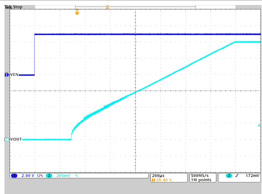
Figure 9-52. Start-Up Timing
