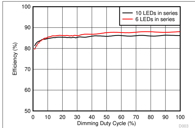
Figure 7-2. Efficiency vs Dimming Duty Cycle
