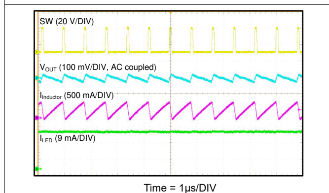
Figure 7-6. Switching-Dimming Duty = 100%
