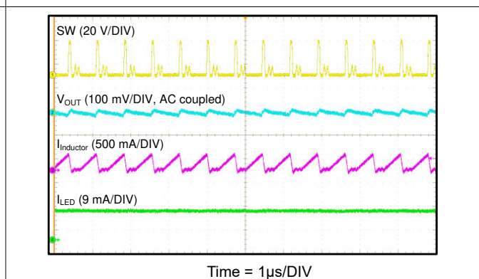
Figure 7-7. Switching-Dimming Duty = 50%
