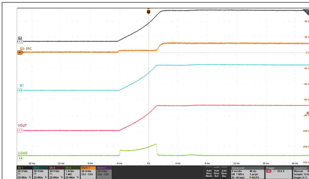
Figure 8-11. Inrush Current Profile With 220µF at the Output (LPM = Low)
