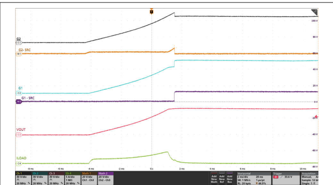
Figure 8-12. Inrush Current Profile With 220µF at the Output and 0.5A Load (LPM = Low)
