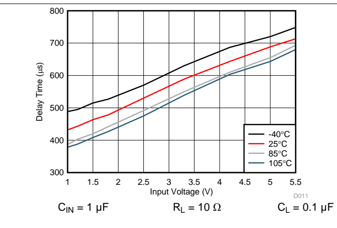
Figure 9. Delay Time vs Input Voltage
