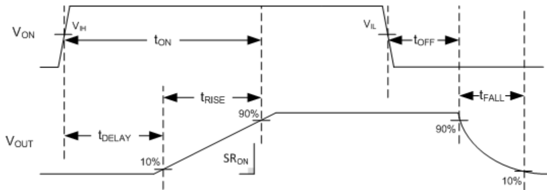
Figure 8-2. Timing Waveforms
