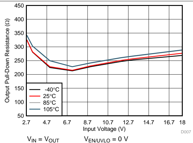
Figure 6. Output Pull-Down Resistance vs Input Voltage
