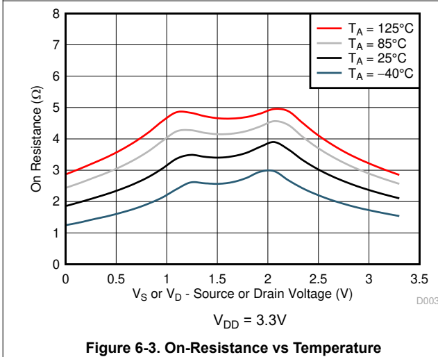
Figure 6-3. On-Resistance vs Temperature
