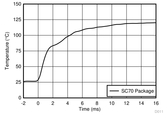
Figure 6-8. Thermal Response (Air-to-Fluid Bath)
