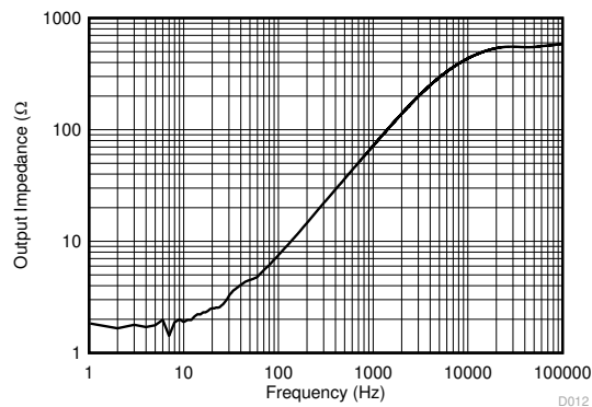
Figure 6-9. Output Impedance vs Frequency
