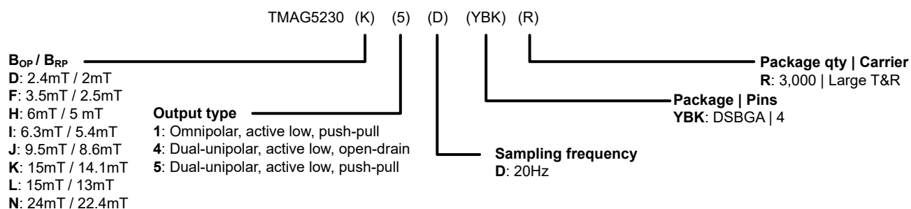
Figure 9-1. Device Nomenclature
