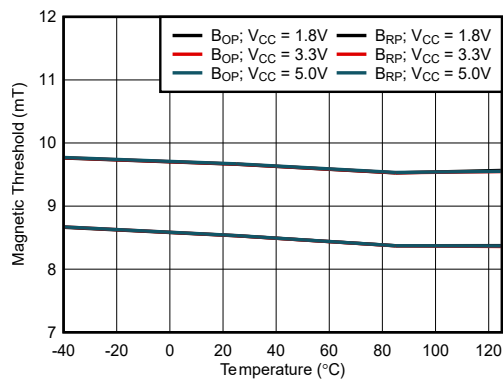
Figure 6-3. 9.5mT B OP : Thresholds vs Temperature
