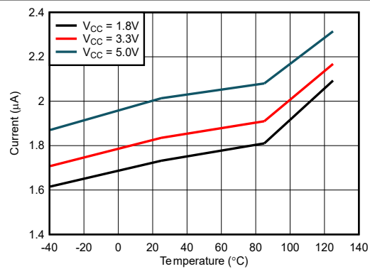
Figure 6-7. 20Hz I_{CAVG} vs Temperature
