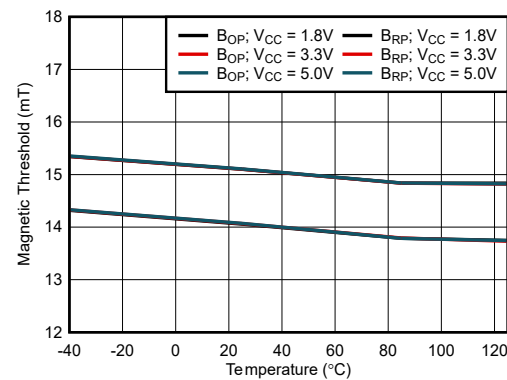
Figure 6-4. 15mT B OP , 14.1mT B RP : Thresholds vs Temperature
