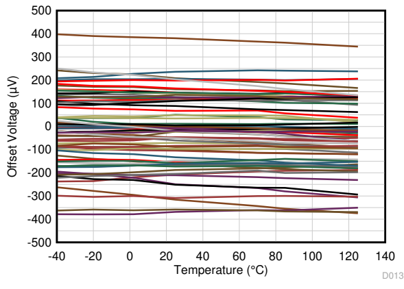
V_{CM} = V_- Data from 74 amplifiers
