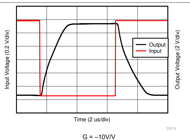
Figure 6-22. Overload Recovery
