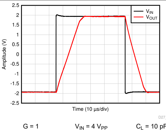
Figure 6-35. Large-Signal Step Response
