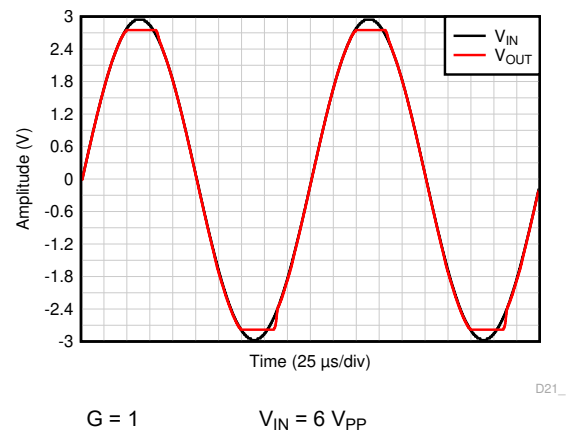
Figure 6-32. No Phase Reversal
