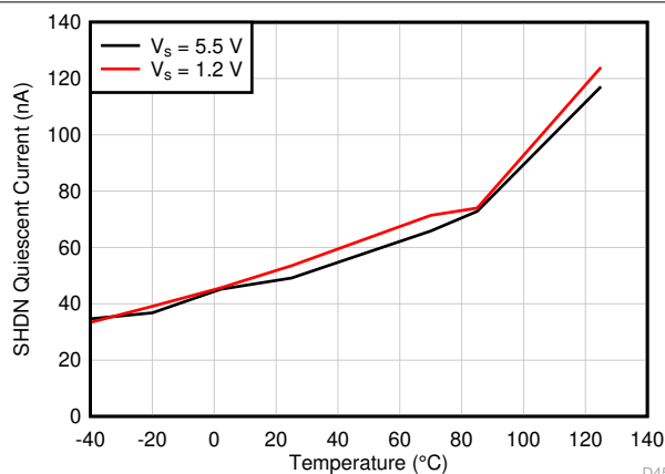
Figure 6-42. Shutdown Mode Quiescent Current vs Temperature
