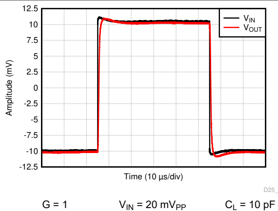
Figure 6-34. Small-Signal Step Response
