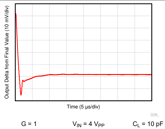
Figure 6-36. Large-Signal Settling Time (Negative)
