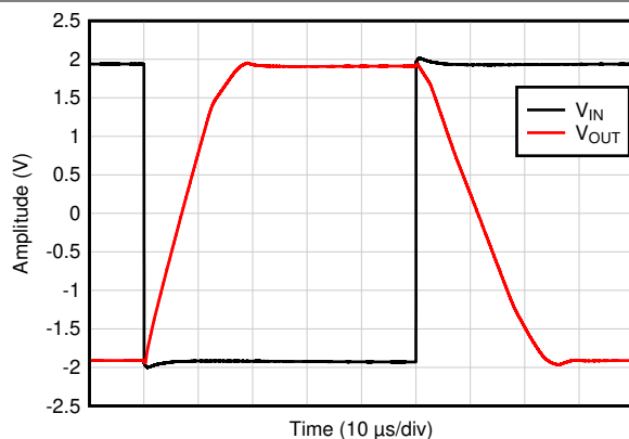
Figure 6-38. Large-Signal Step Response
