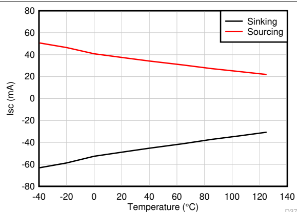
Figure 6-40. Short-Circuit Current vs Temperature
