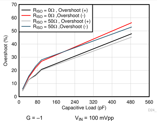
Figure 6-30. Small Signal Overshoot vs Capacitive Load
