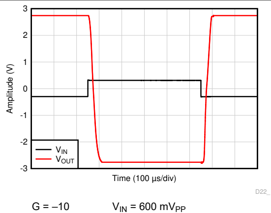
Figure 6-33. Overload Recovery
