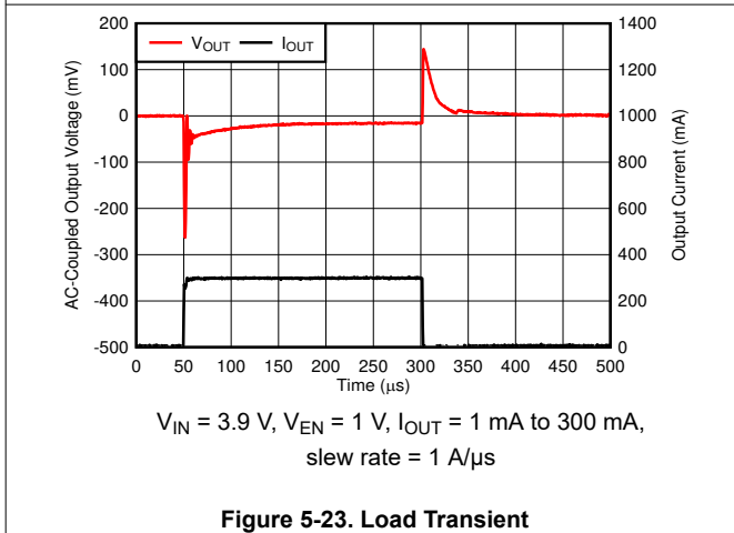
Figure 5-23. Load Transient
