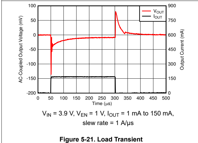
Figure 5-21. Load Transient
