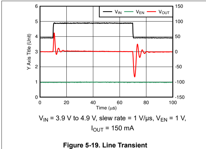
Figure 5-19. Line Transient
