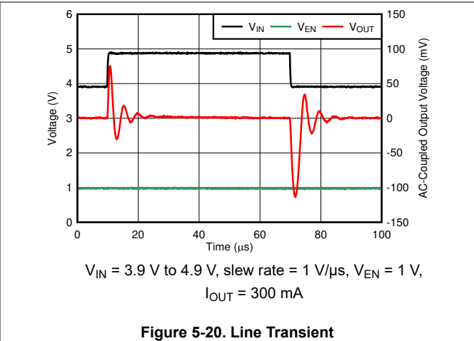
Figure 5-20. Line Transient
