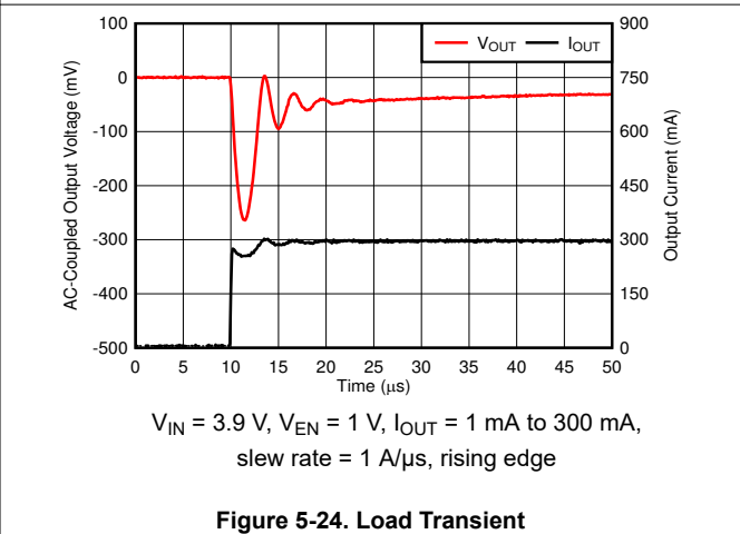
Figure 5-24. Load Transient
