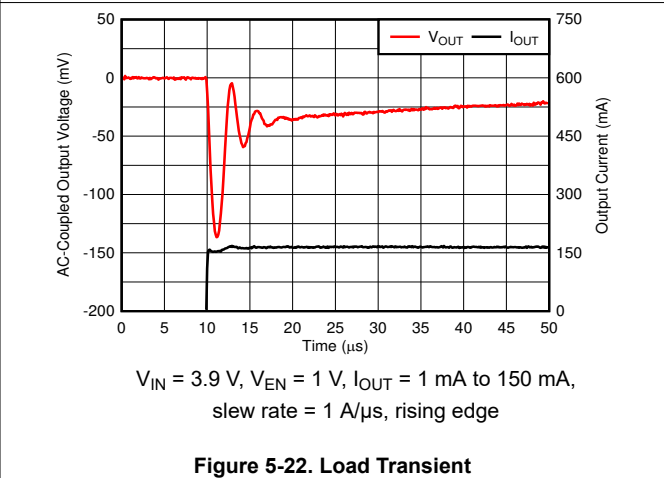
Figure 5-22. Load Transient
