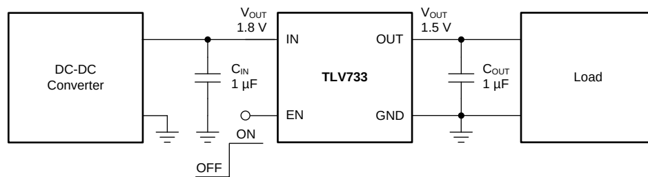
Figure 35. DC-DC Converter Post Regulation
