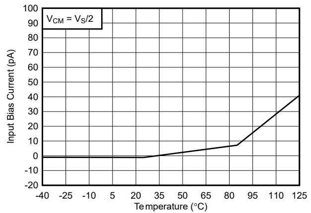
Figure 5-6. Bias Current vs. Temperature, 40V
