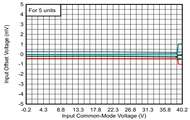
Figure 5-4. Offset Voltage vs. Common-Mode, 40V
