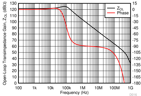
Full-bias simulation
