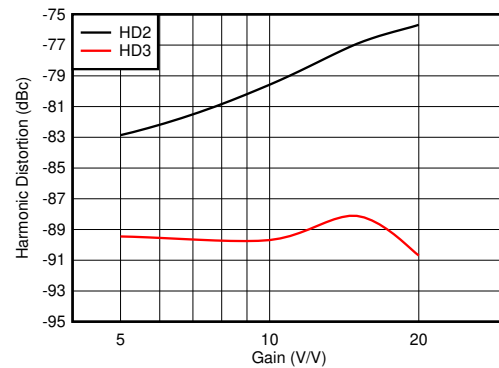
f = 1\text{ MHz} , V_O = 2\text{ V}_{PP}
