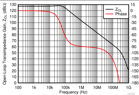
Low-bias simulation
