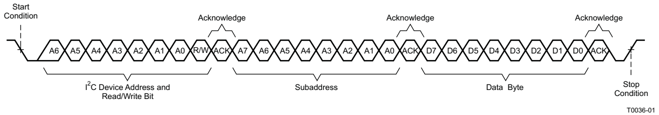
Figure 51. Write Transfer
