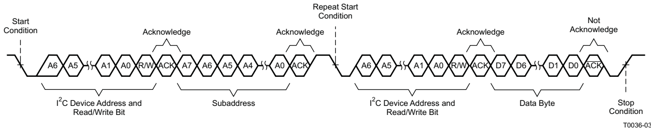
Figure 52. Read Transfer
