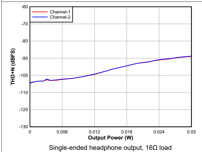
Figure 5-23. DAC THD+N Level vs Output Power
