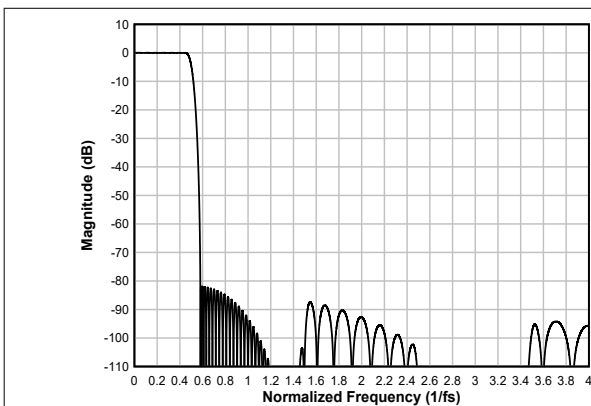
Figure 6-69. Linear-phase Interpolation Filter Magnitude Response
