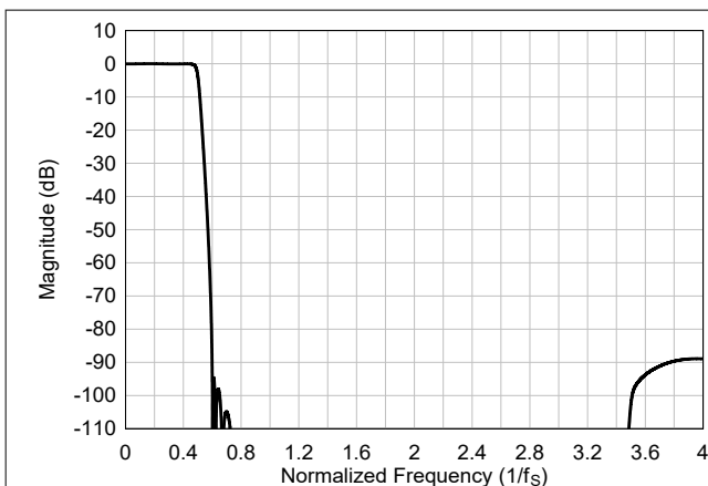
Figure 6-95. Ultra-Low-Latency interpolation Filter Magnitude Response
