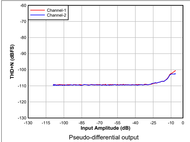
Figure 5-21. DAC THD+N Level vs Input
