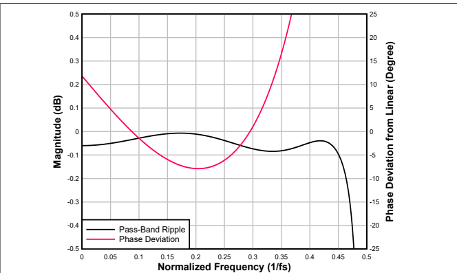
Figure 6-94. Ultra-Low-Latency interpolation Filter Pass-Band Ripple and Phase Deviation
