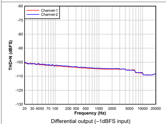
Figure 5-25. DAC THD+N Level vs Frequency
