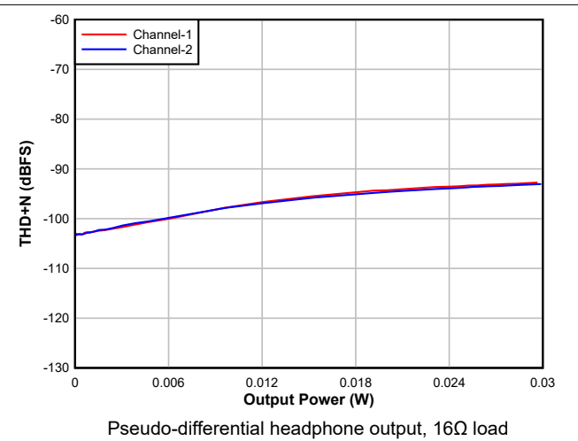
Figure 5-24. DAC THD+N Level vs Output Power
