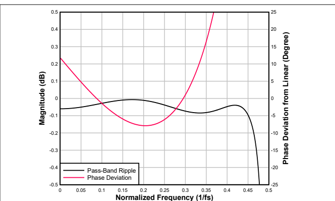
Figure 6-96. Ultra-Low-Latency interpolation Filter Pass-Band Ripple and Phase Deviation
