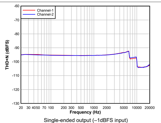
Figure 5-26. DAC THD+N Level vs Frequency
