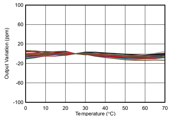
Output Voltage vs Free-Air-Temperature
