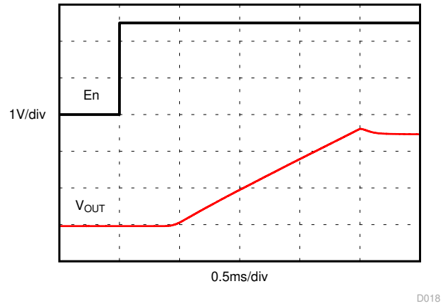
Figure 6-20. Turn-on Time (Enable)
