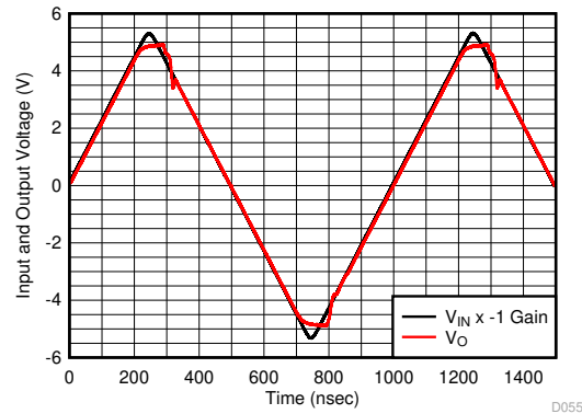
Figure 6-14. Output Overdrive Recovery
