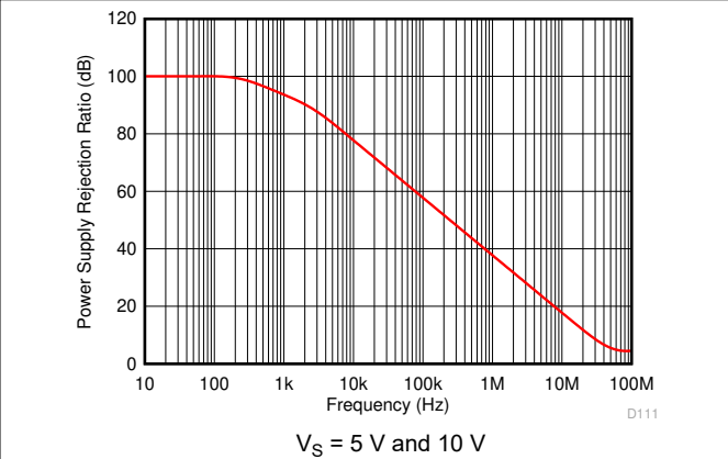
Figure 6-51. Power Supply Rejection Ratio vs Frequency
