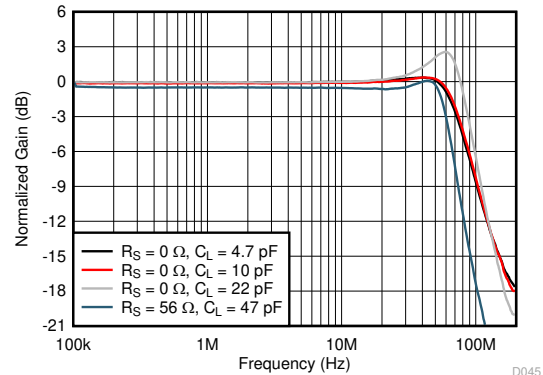
See Figure 8-1 and Figure 7-1, V_O = 20\text{ mV}_{PP} , gain = 2 V/V
