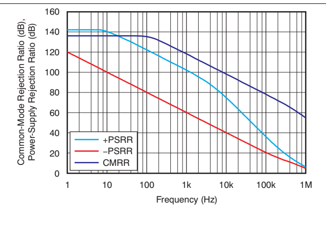
Figure 10. CMRR and PSRR vs Frequency (Referred-to-Input)
