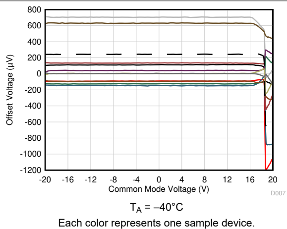
Figure 5-26. Offset Voltage vs Common-Mode Voltage (New Die)
