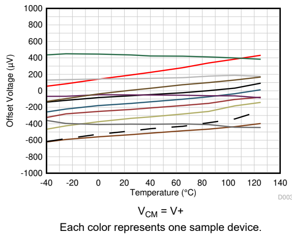
Figure 5-21. Offset Voltage vs Temperature (New Die)
