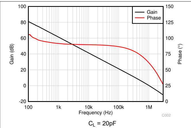
Figure 5-28. Open-Loop Gain and Phase vs Frequency (New Die)
