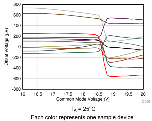
Figure 5-24. Offset Voltage vs Common-Mode Voltage (Transition Region) (New Die)
