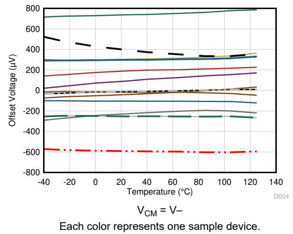
Figure 5-22. Offset Voltage vs Temperature (New Die)
