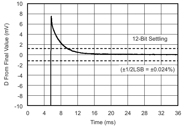
Figure 5-32. Large-Signal Settling Time (10-V Positive Step)
