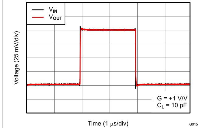
Figure 5-17. Small-Signal Step Response
