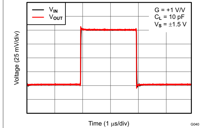
Figure 5-18. Small-Signal Step Response
