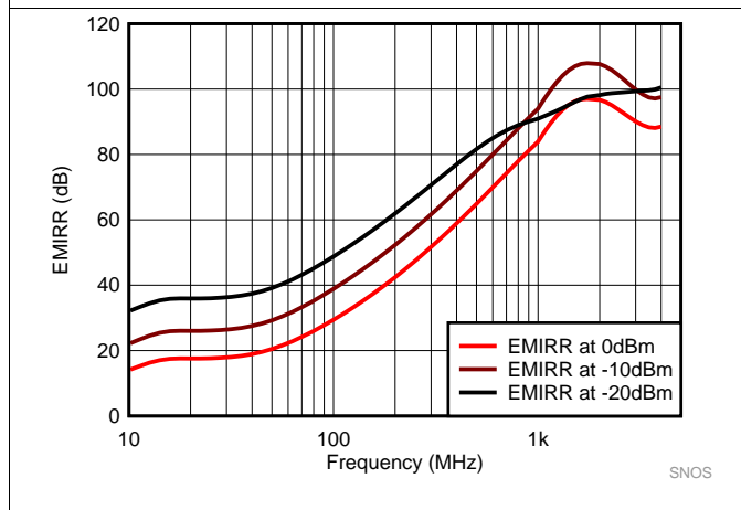
Figure 23. EMIRR Performance
