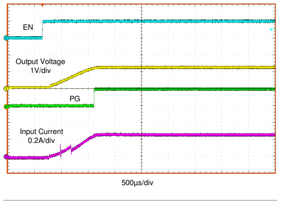
Figure 8-16. Start-Up
