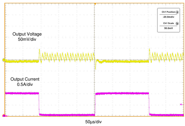
Figure 8-20. Load Transients In AUTO Mode
