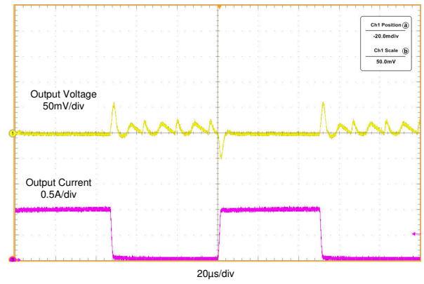
Figure 8-14. Load Transients In AUTO Mode
