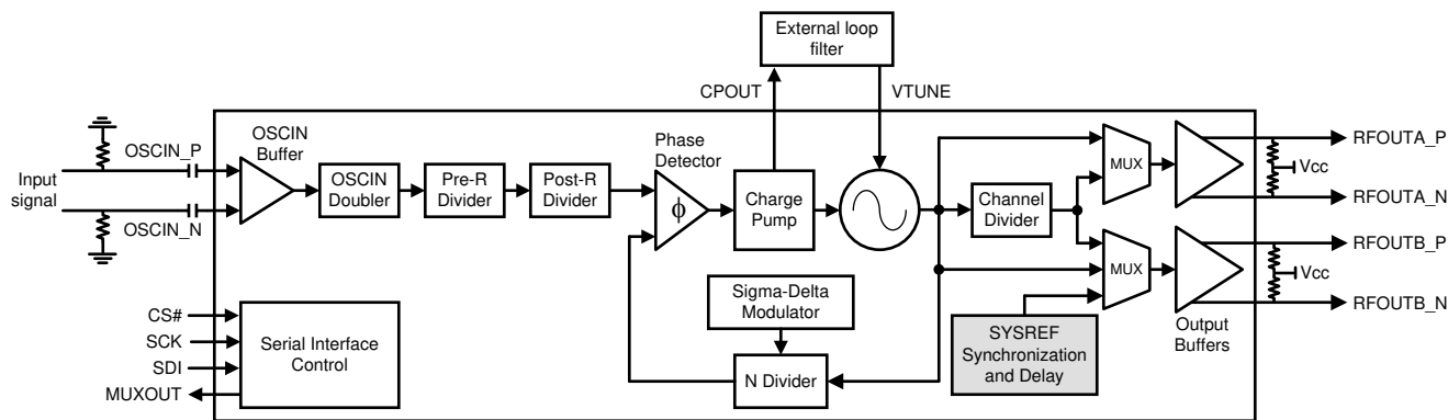
Simplified Schematic
