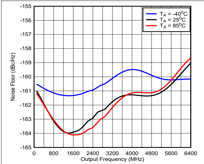
Figure 5-8. Noise Floor in Divider Mode
