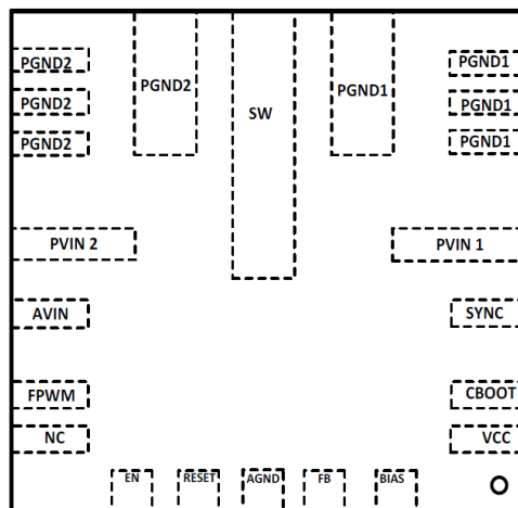
Figure 6-1. RNL Package 22-Pin VQFN Top View
