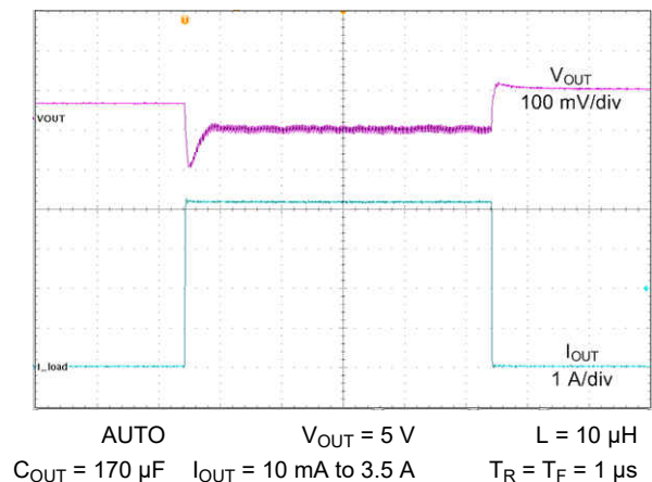
Figure 9-14. Load Transients
