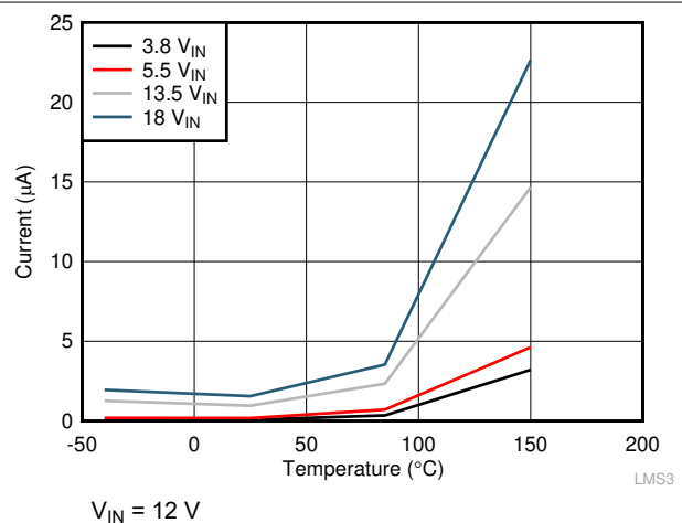
Figure 7-6. Shutdown Current
