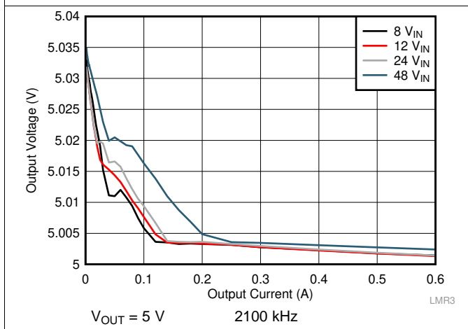
Figure 45. Load Regulation
