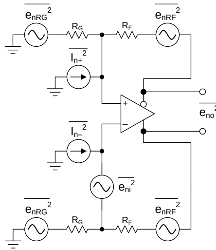
Figure 63. FDA Noise-Analysis Circuit
