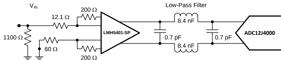
Figure 65. Low-Loss ADC
