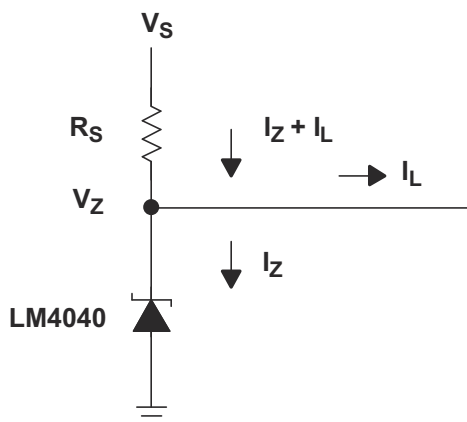
Simplified Schematic
